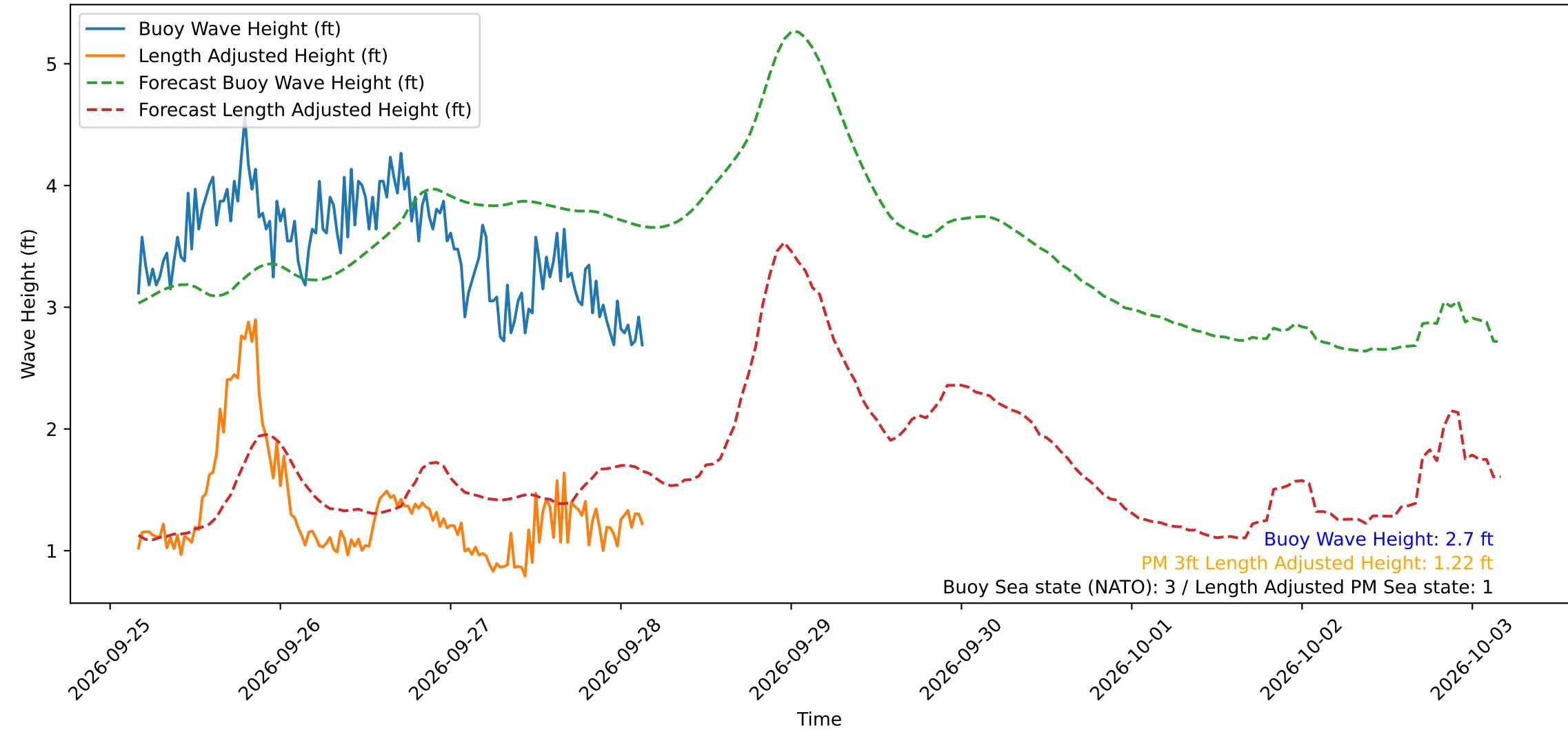
Wave Heights over Time for Green Beach at 2026-09-28 03:51:14
