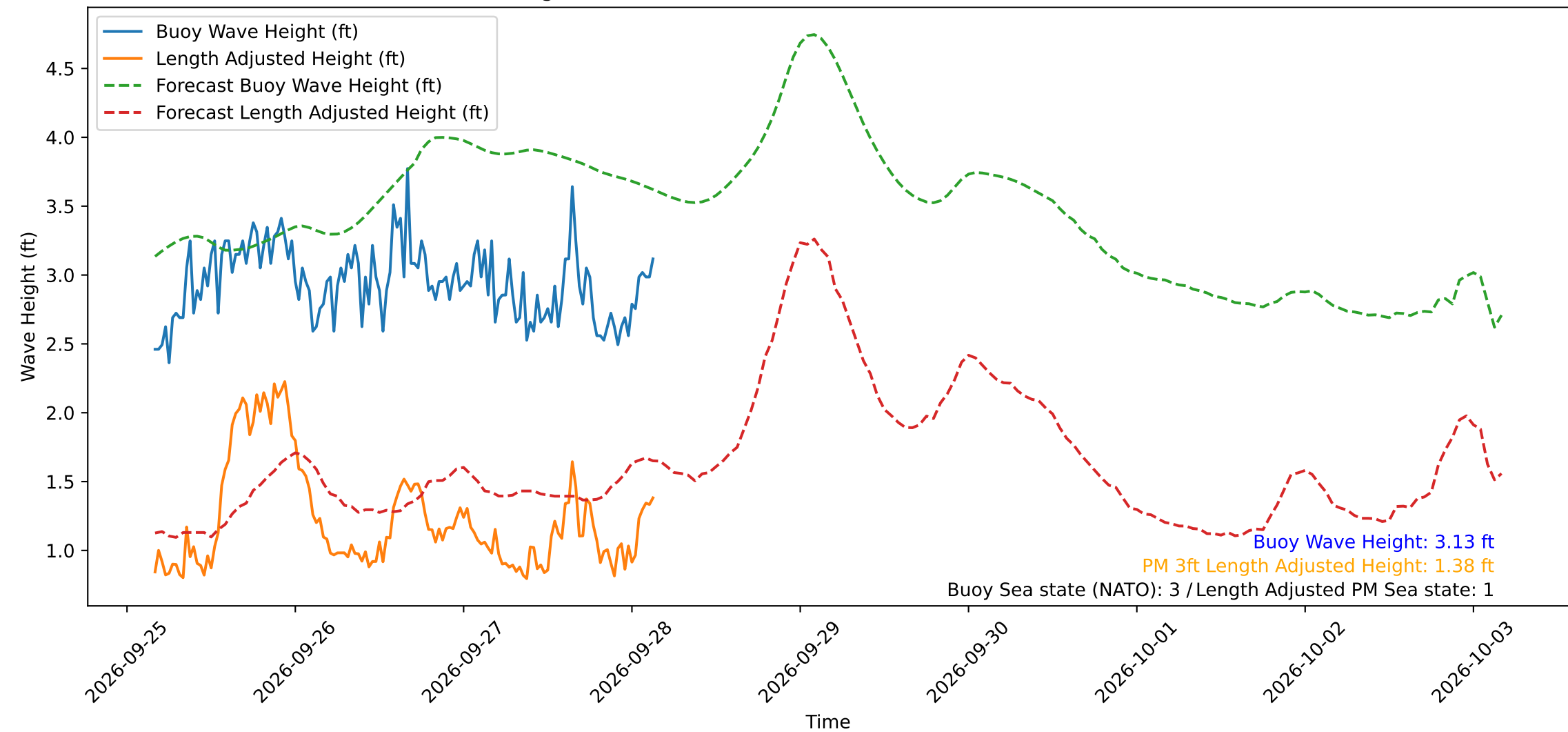
Wave Heights over Time for Oceanside Harbor at 2026-09-28 03:50:30
