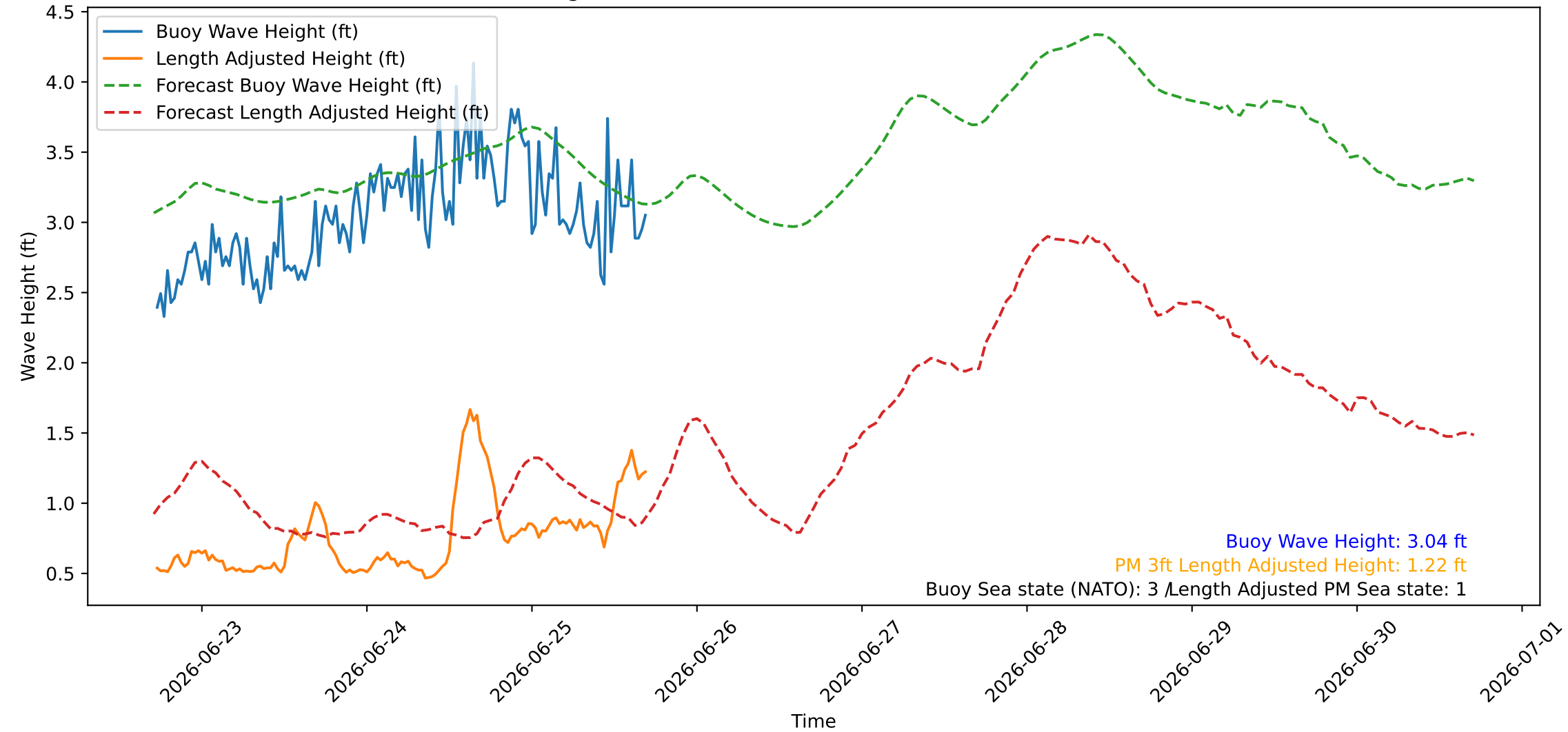
Wave Heights over Time for Red Beach at 2026-06-25 17:10:45
