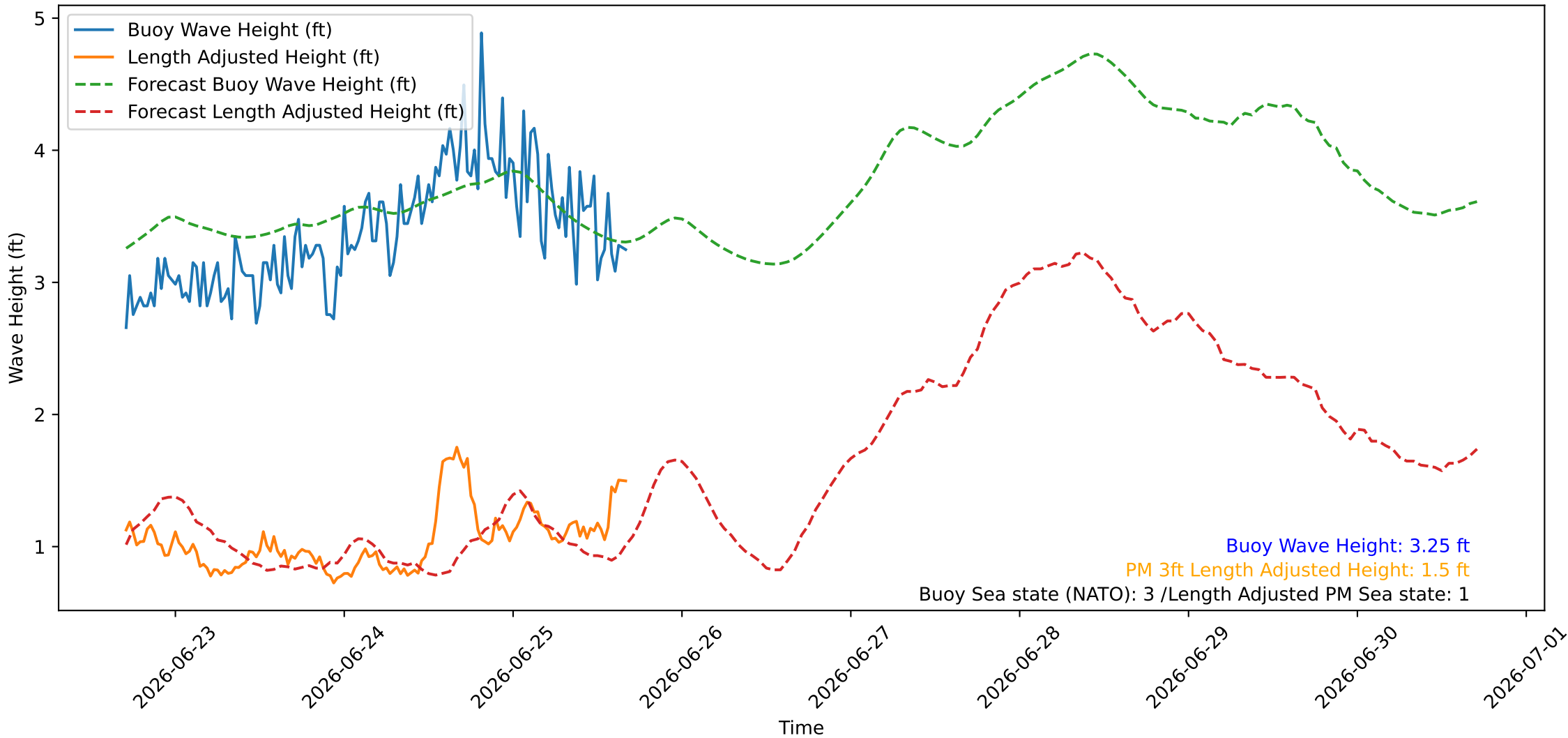
Wave Heights over Time for Oceanside Harbor at 2026-06-25 17:10:26
