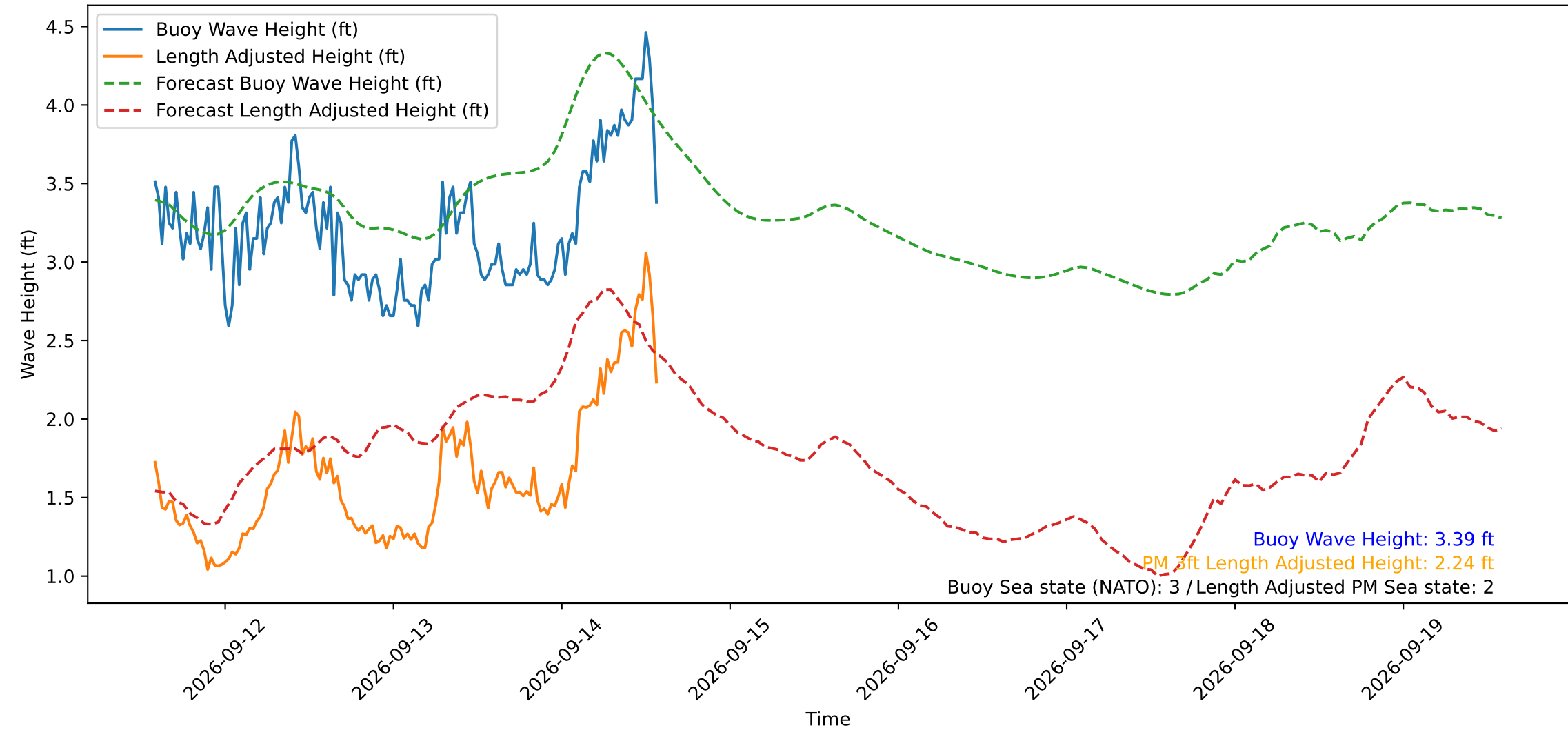
Wave Heights over Time for Oceanside Harbor at 2026-09-14 14:00:30
