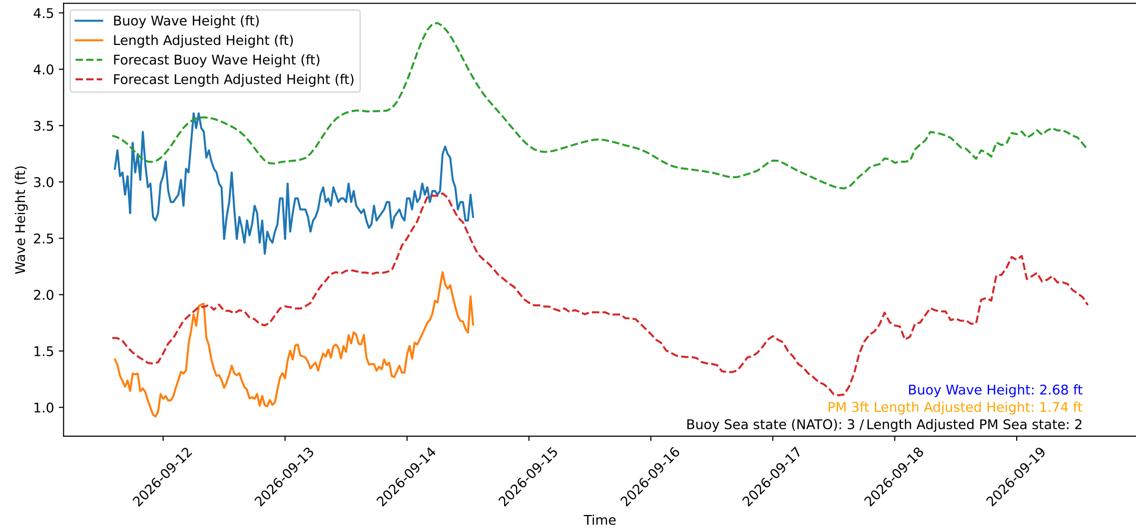
Wave Heights over Time for Green Beach at 2026-09-14 14:01:13
