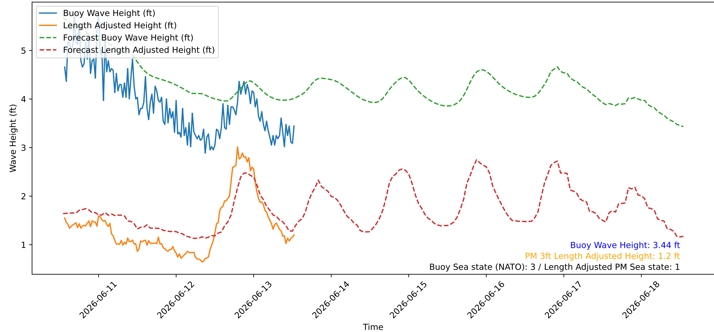
Wave Heights over Time for Green Beach at 2026-06-13 13:21:10
