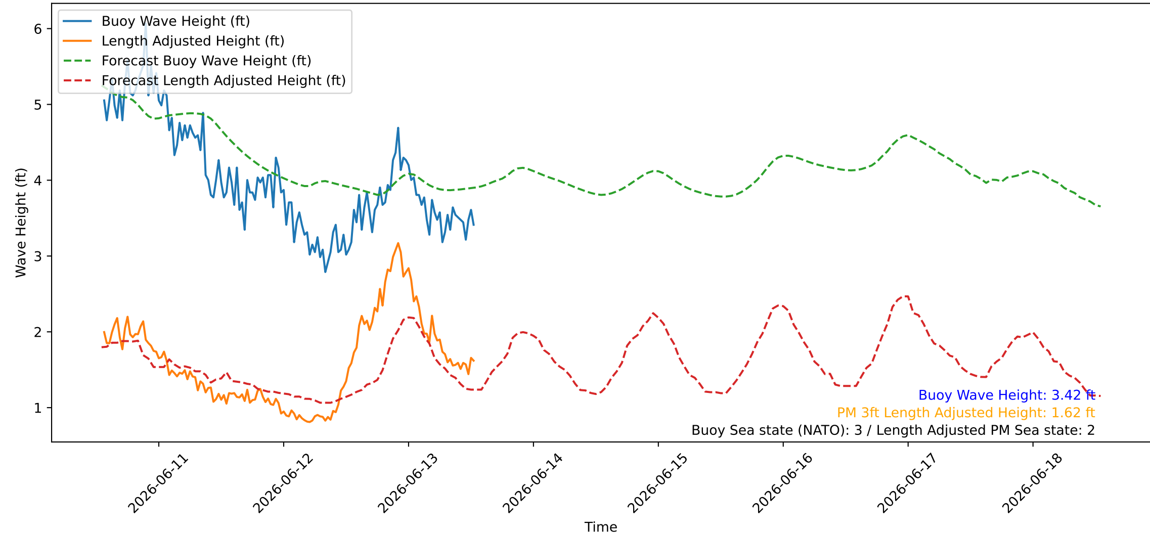
Wave Heights over Time for Oceanside Harbor at 2026-06-13 13:20:27
