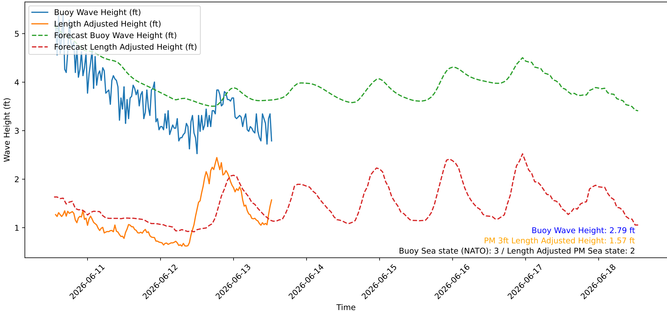
Wave Heights over Time for Red Beach at 2026-06-13 13:20:48
