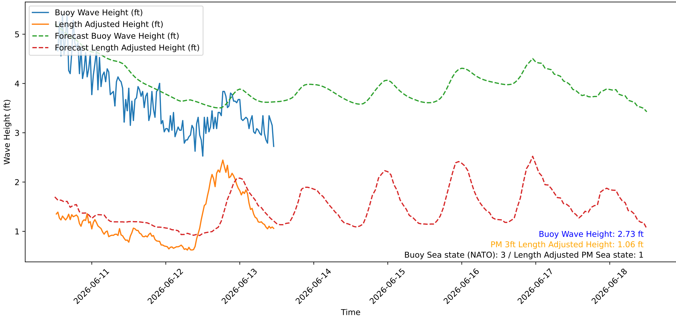
Wave Heights over Time for Red Beach at 2026-06-13 12:00:45
