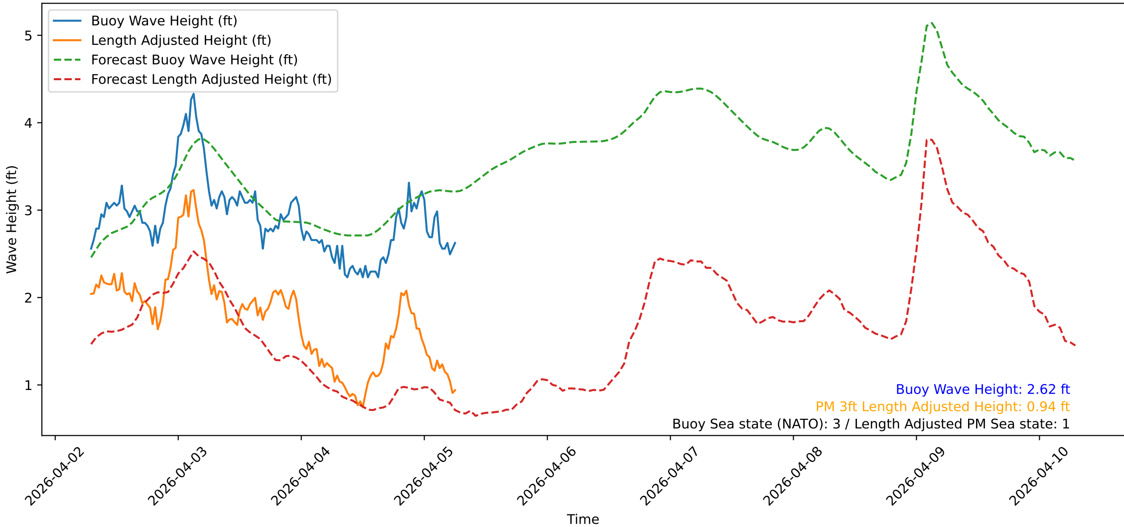
Wave Heights over Time for Green Beach at 2026-04-05 07:01:10
