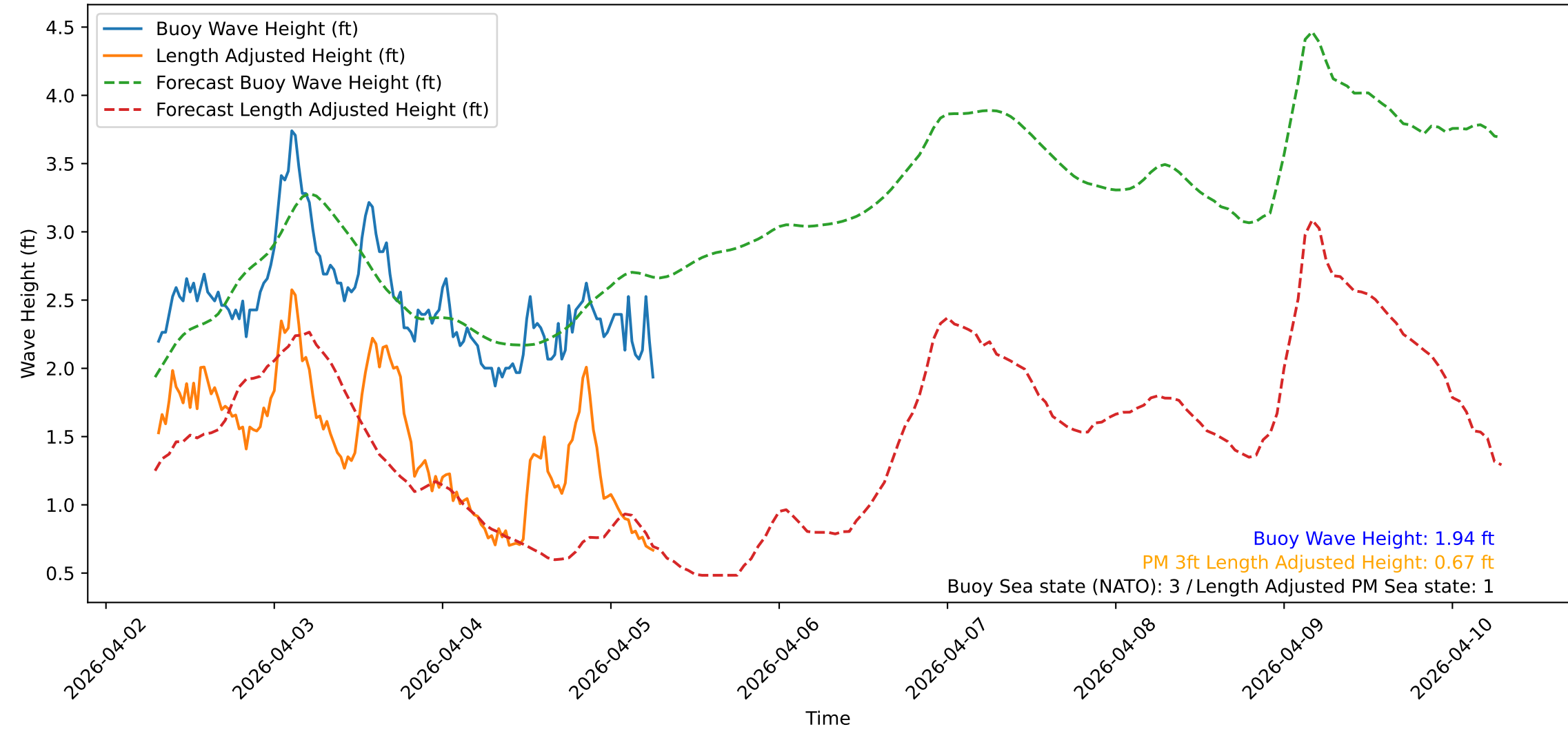
Wave Heights over Time for Red Beach at 2026-04-05 07:00:48
