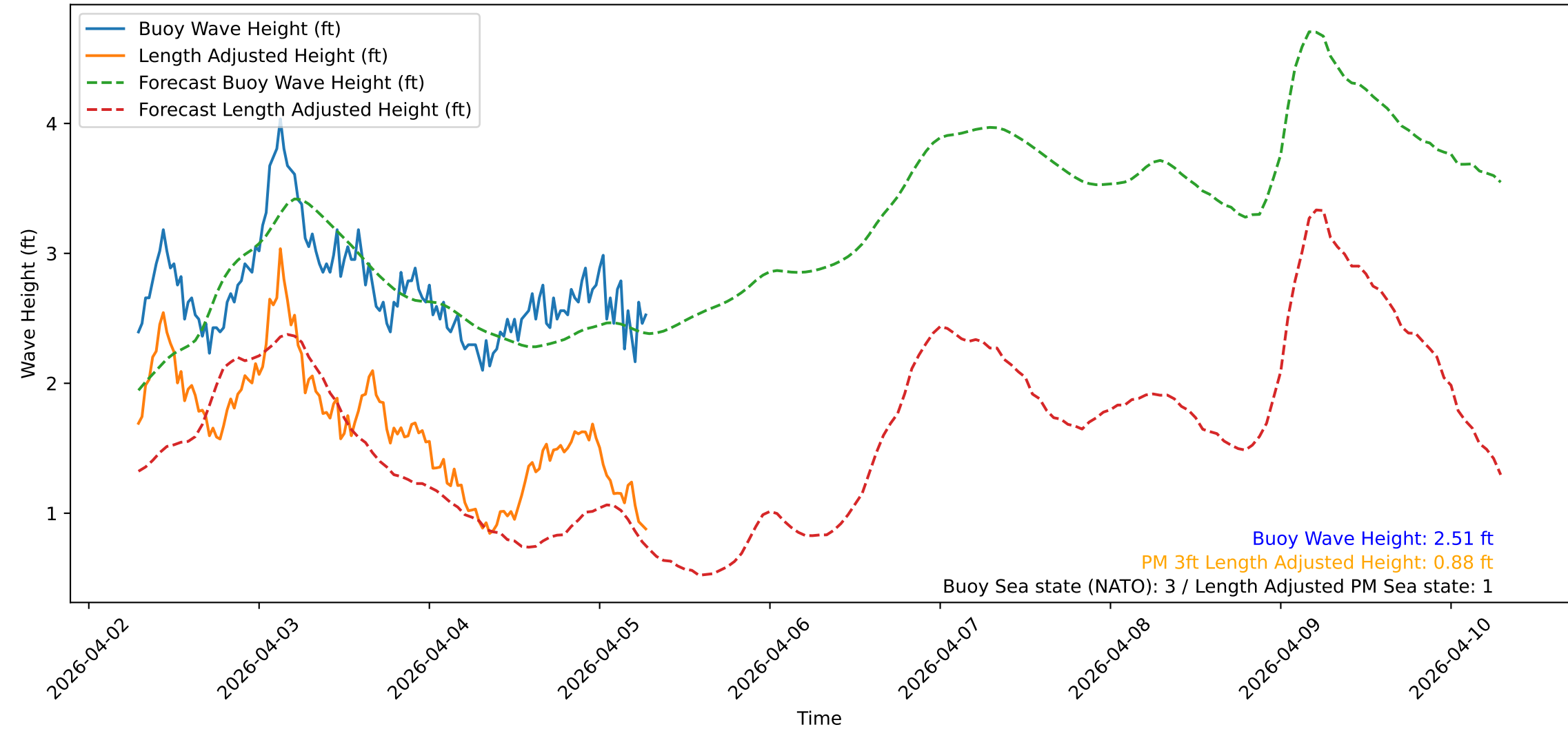
Wave Heights over Time for Oceanside Harbor at 2026-04-05 07:00:32
