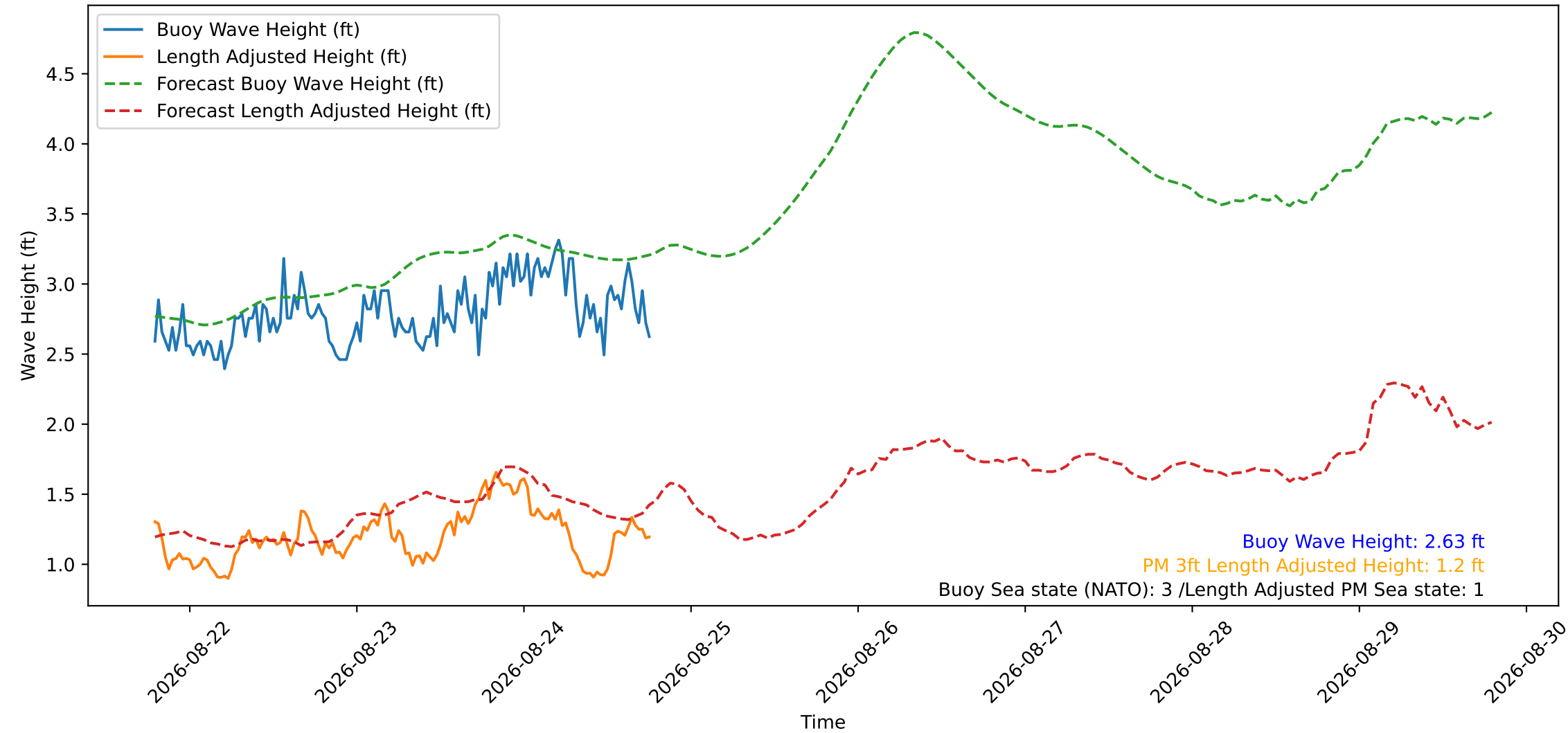
Wave Heights over Time for Green Beach at 2026-08-24 18:41:13
