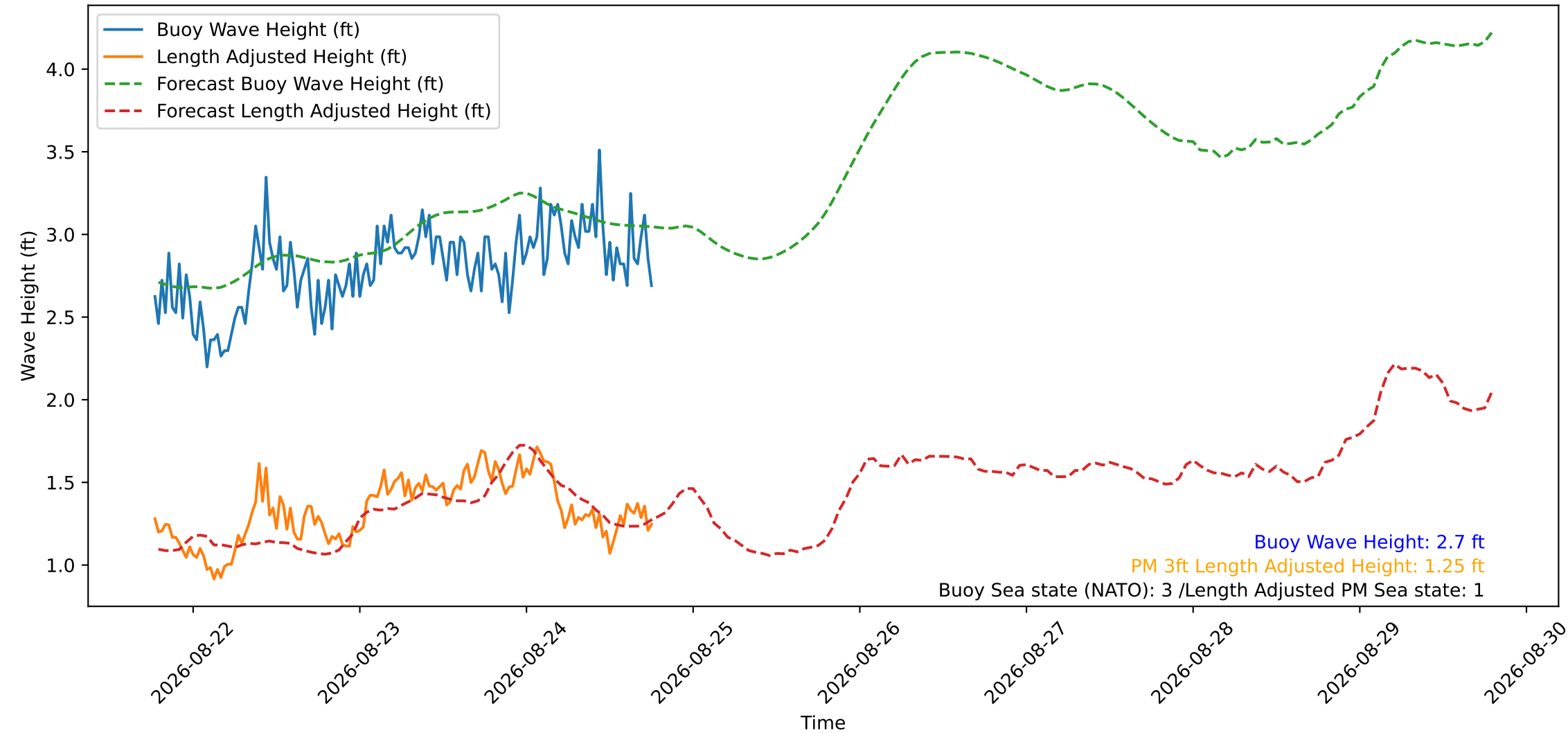
Wave Heights over Time for Oceanside Harbor at 2026-08-24 18:40:30
