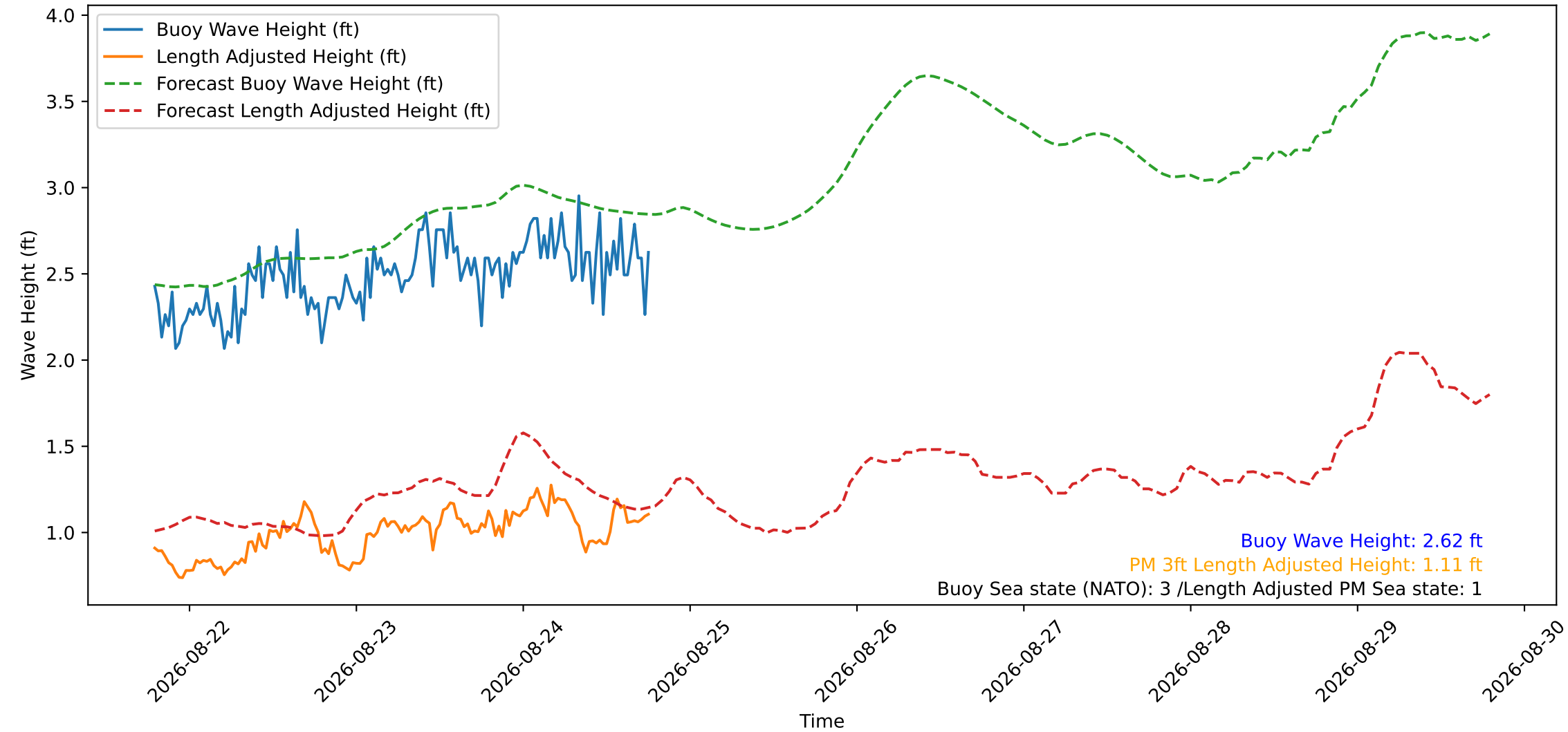
Wave Heights over Time for Red Beach at 2026-08-24 18:40:50
