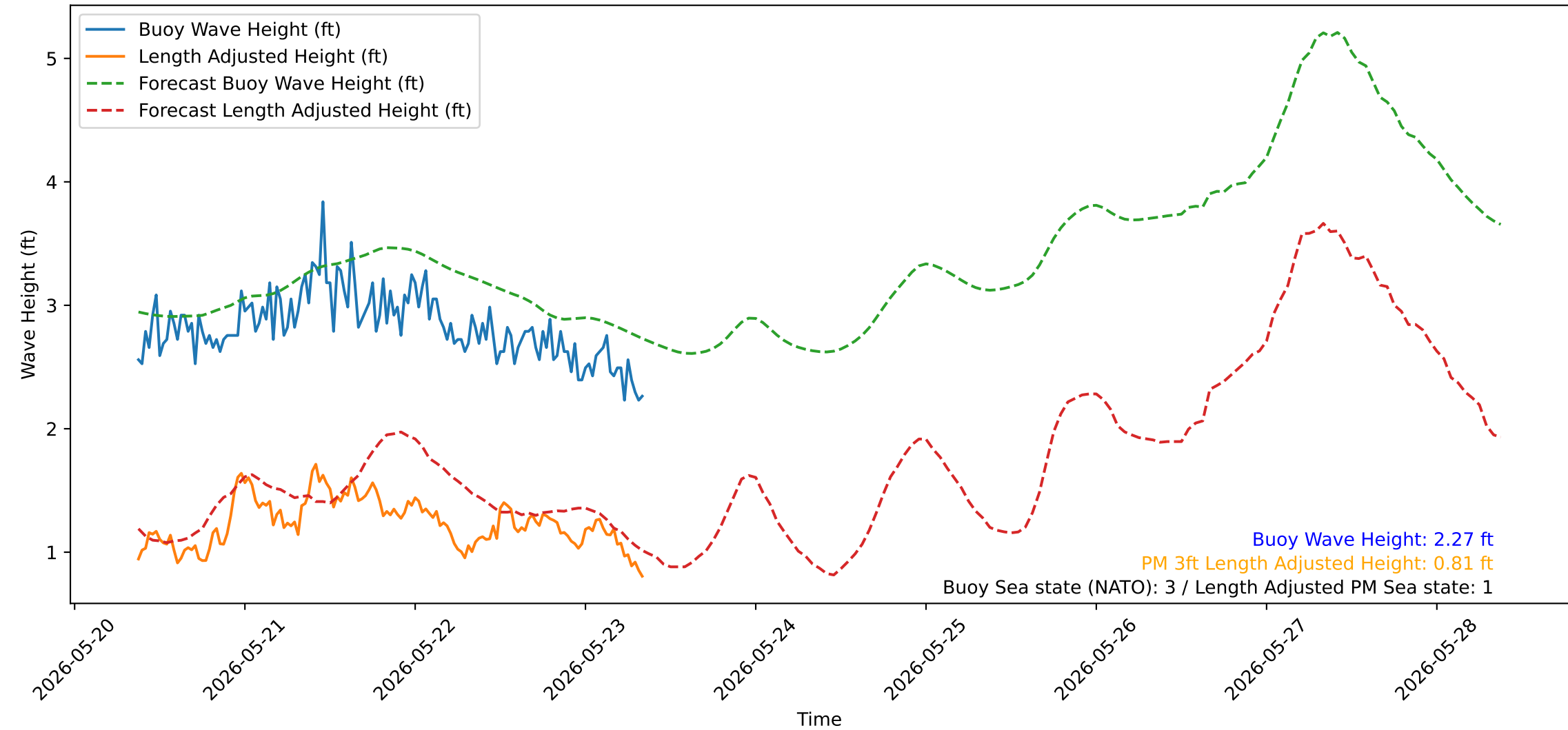
Wave Heights over Time for Oceanside Harbor at 2026-05-23 08:50:31
