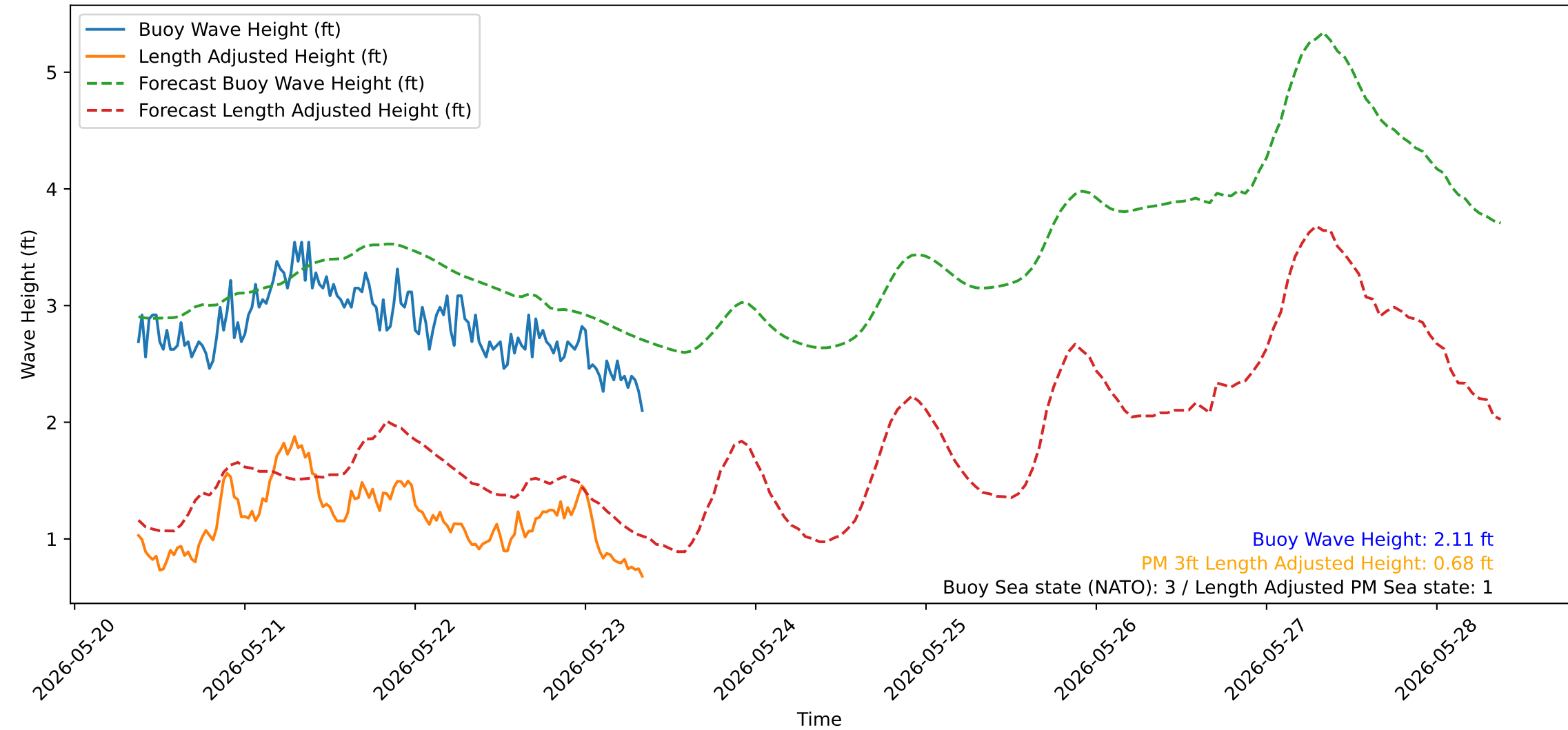
Wave Heights over Time for Green Beach at 2026-05-23 08:51:14
