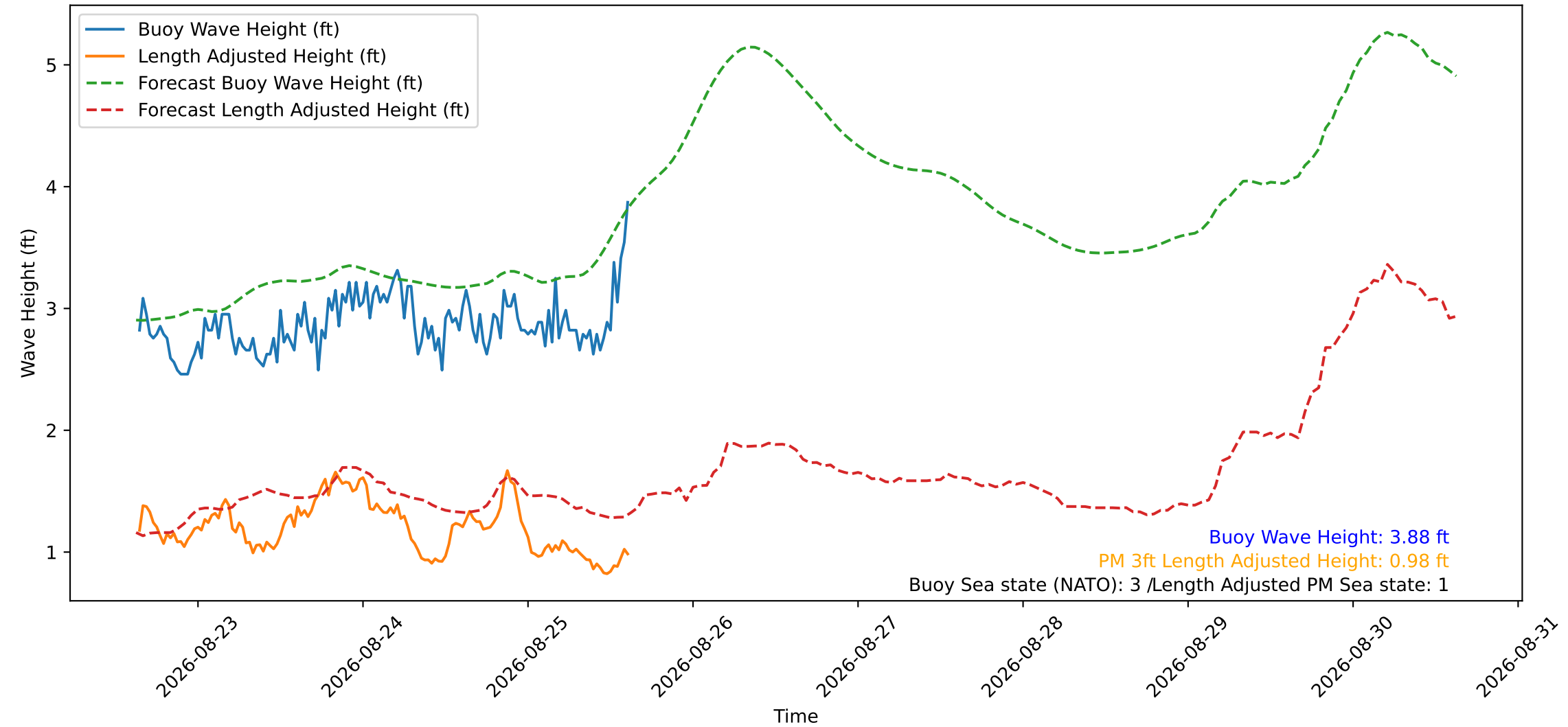
Wave Heights over Time for Green Beach at 2026-08-25 15:11:12
