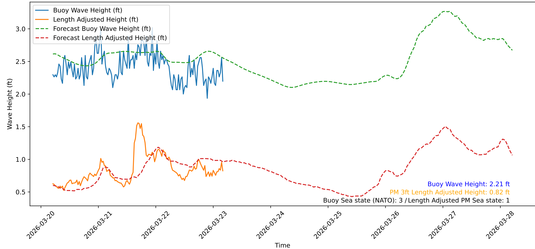
Wave Heights over Time for Oceanside Harbor at 2026-03-23 04:50:31
