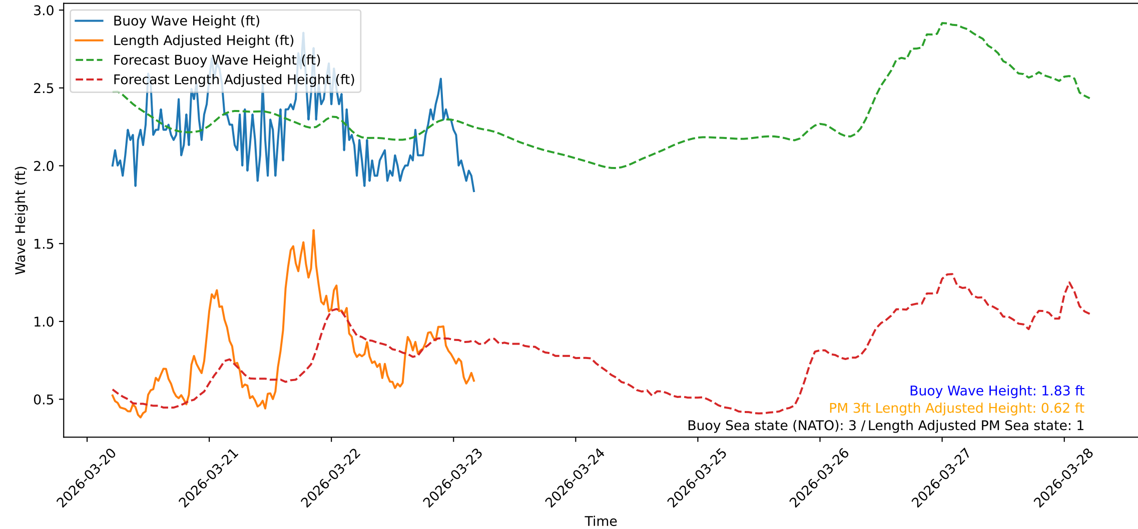
Wave Heights over Time for Red Beach at 2026-03-23 04:50:48
