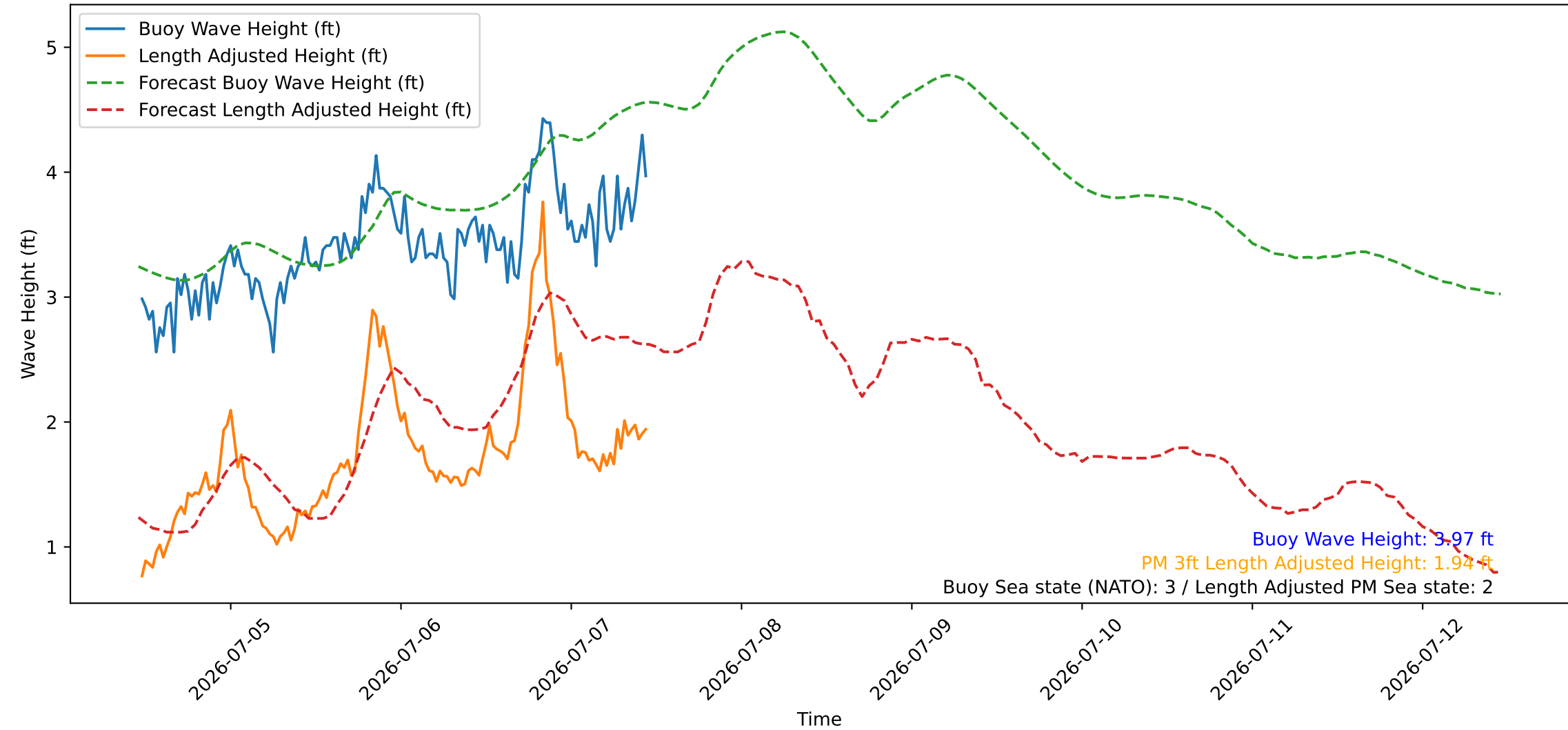
Wave Heights over Time for Green Beach at 2026-07-07 11:21:09
