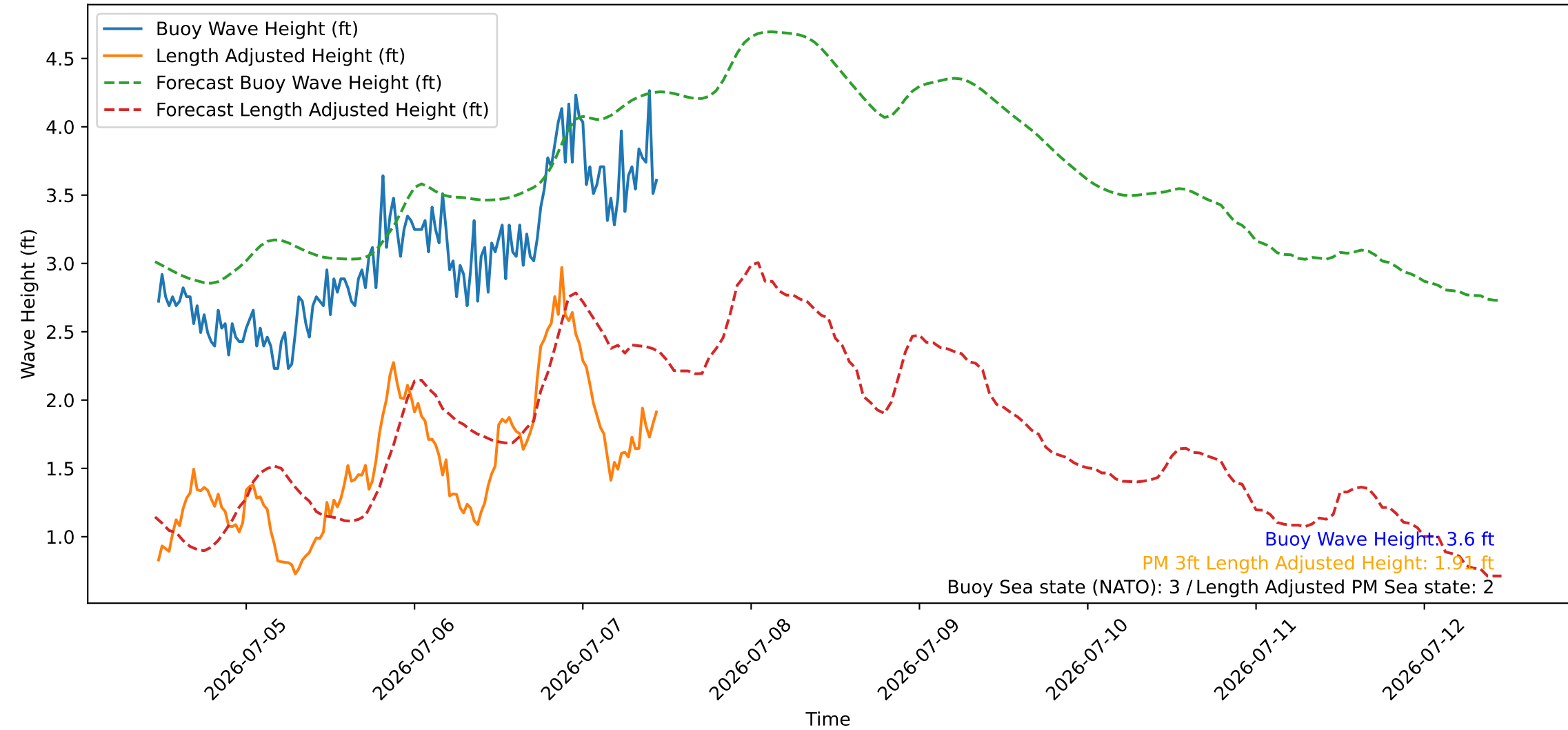
Wave Heights over Time for Red Beach at 2026-07-07 11:20:46
