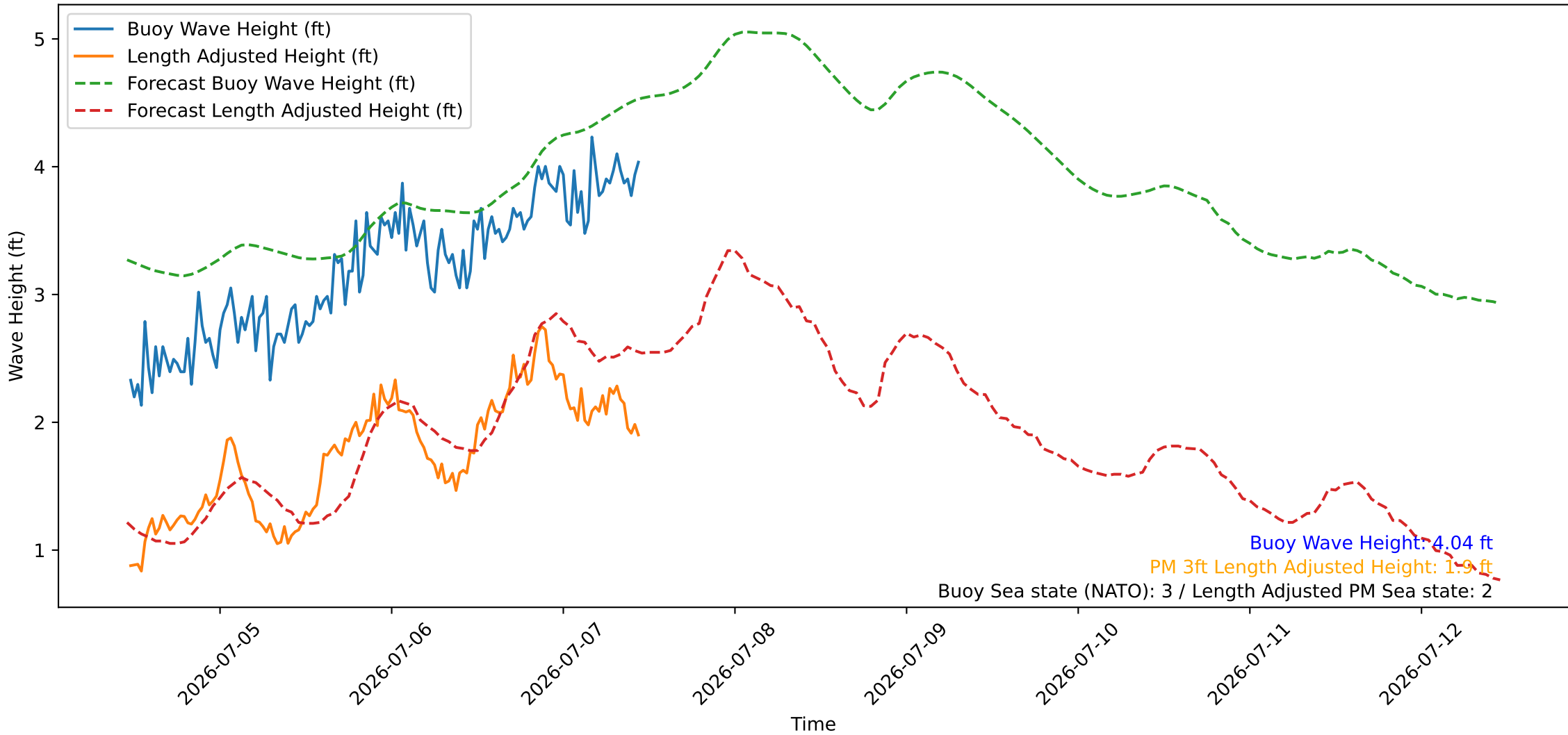
Wave Heights over Time for Oceanside Harbor at 2026-07-07 11:20:25
