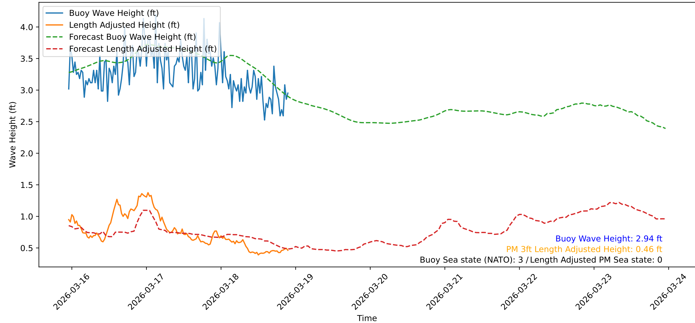
Wave Heights over Time for Green Beach at 2026-03-18 23:01:10
