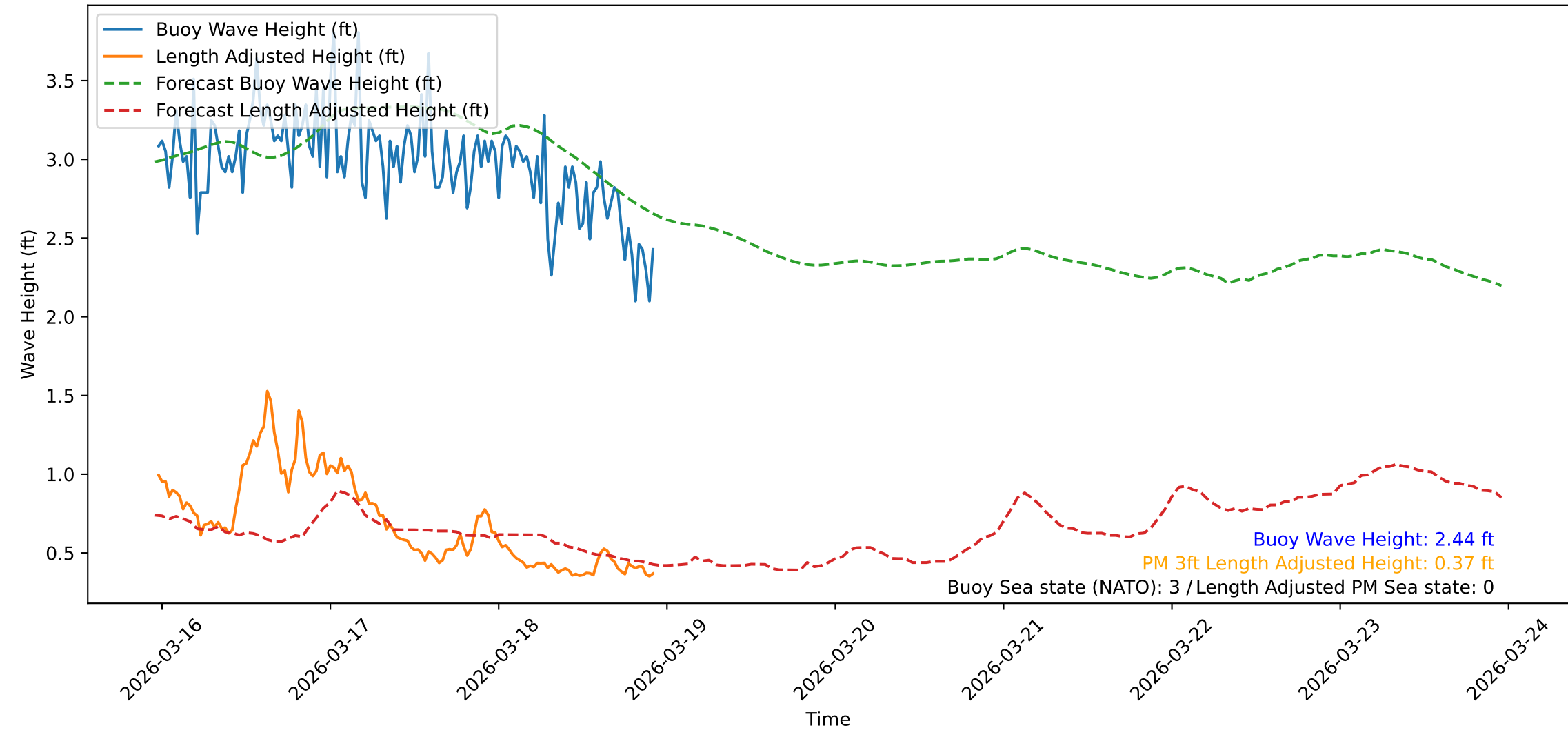
Wave Heights over Time for Red Beach at 2026-03-18 23:00:47
