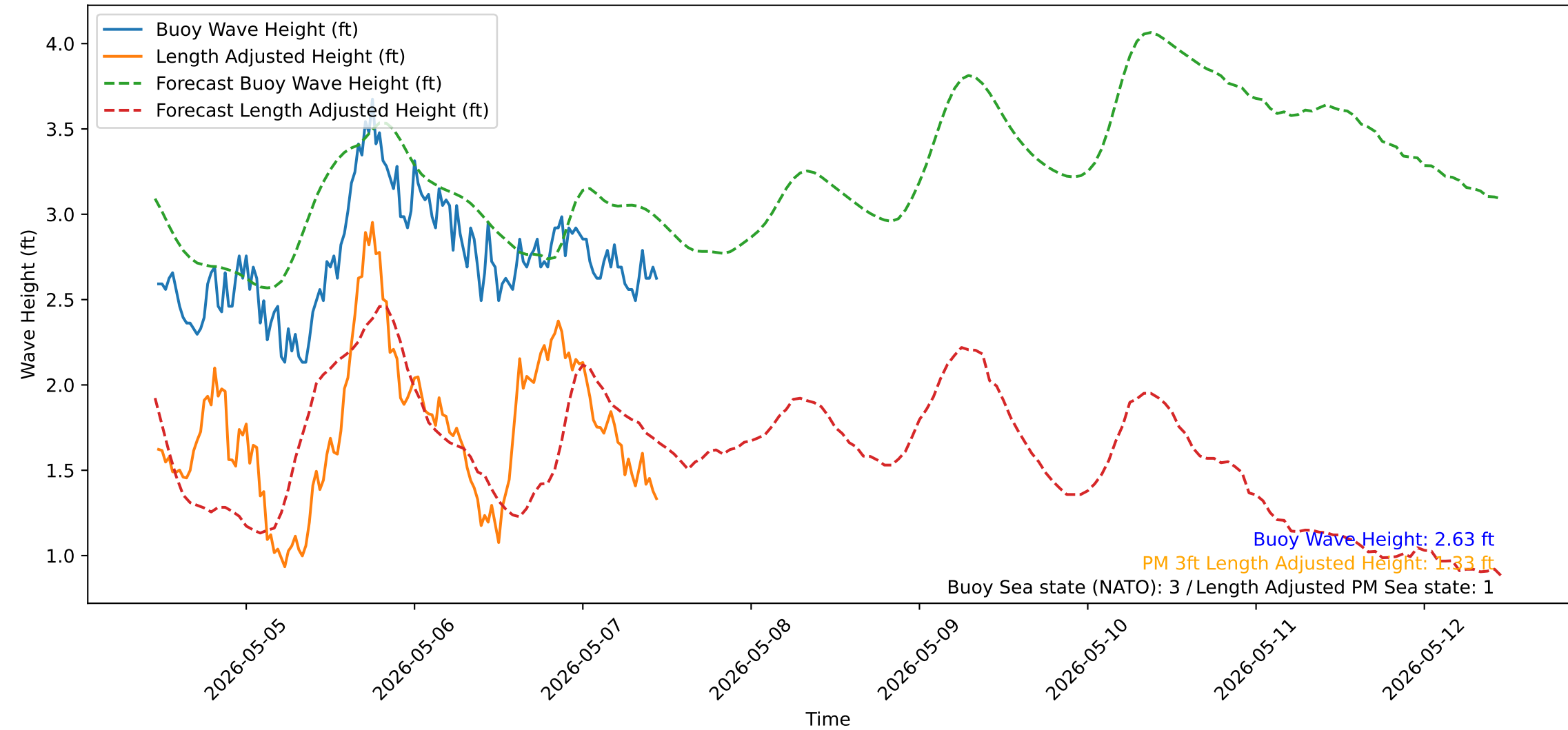
Wave Heights over Time for Green Beach at 2026-05-07 11:21:13
