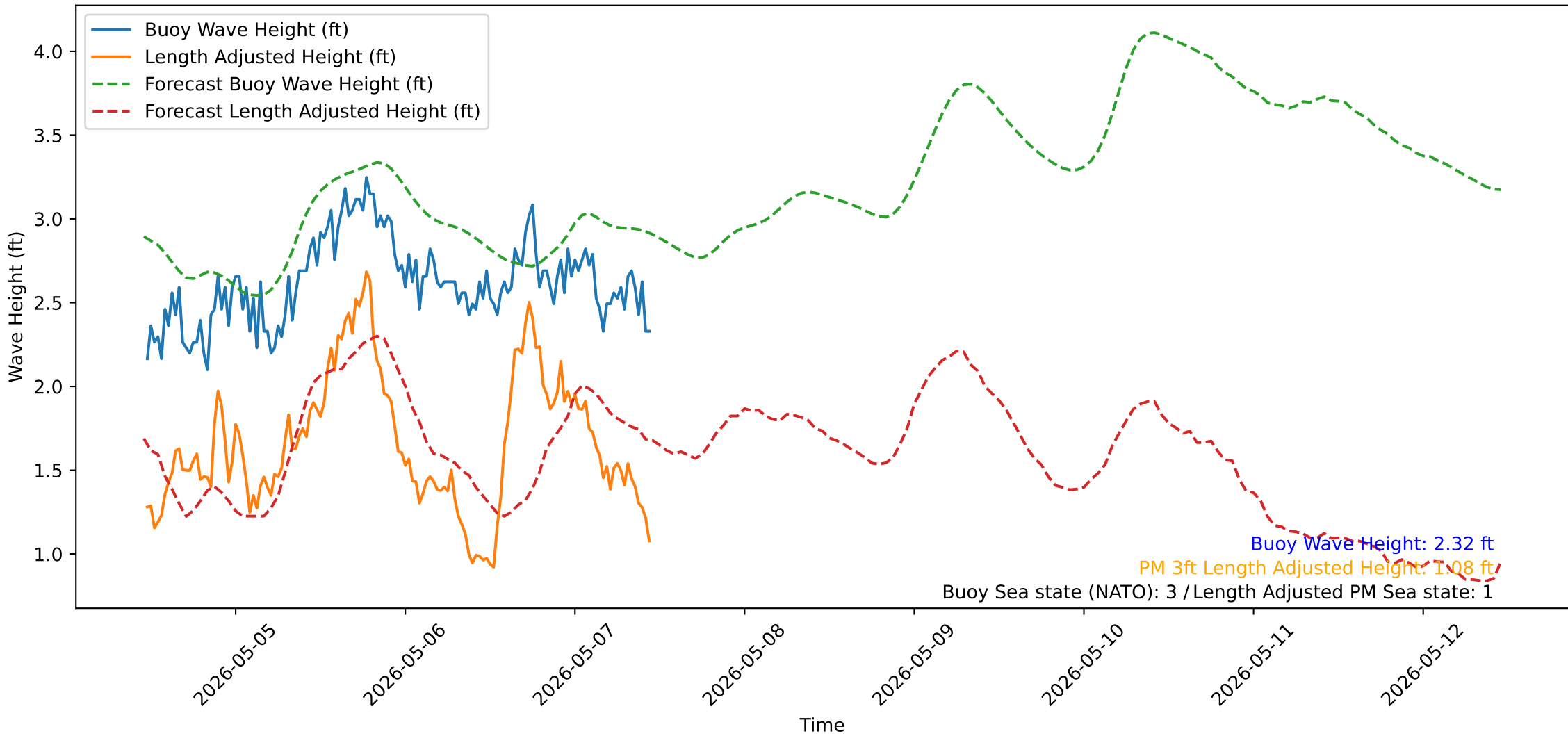
Wave Heights over Time for Oceanside Harbor at 2026-05-07 11:20:31
