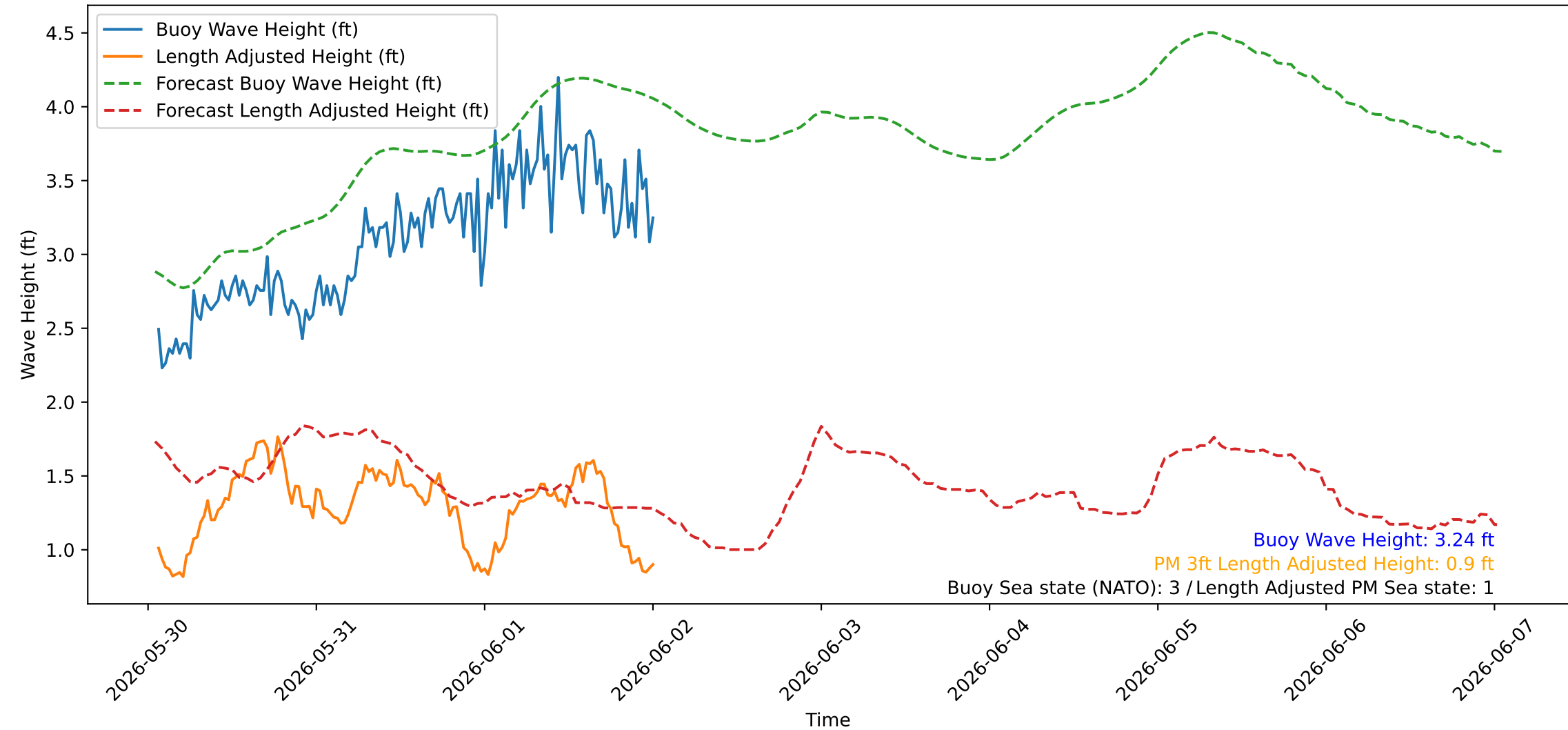
Wave Heights over Time for Red Beach at 2026-06-02 01:10:44
