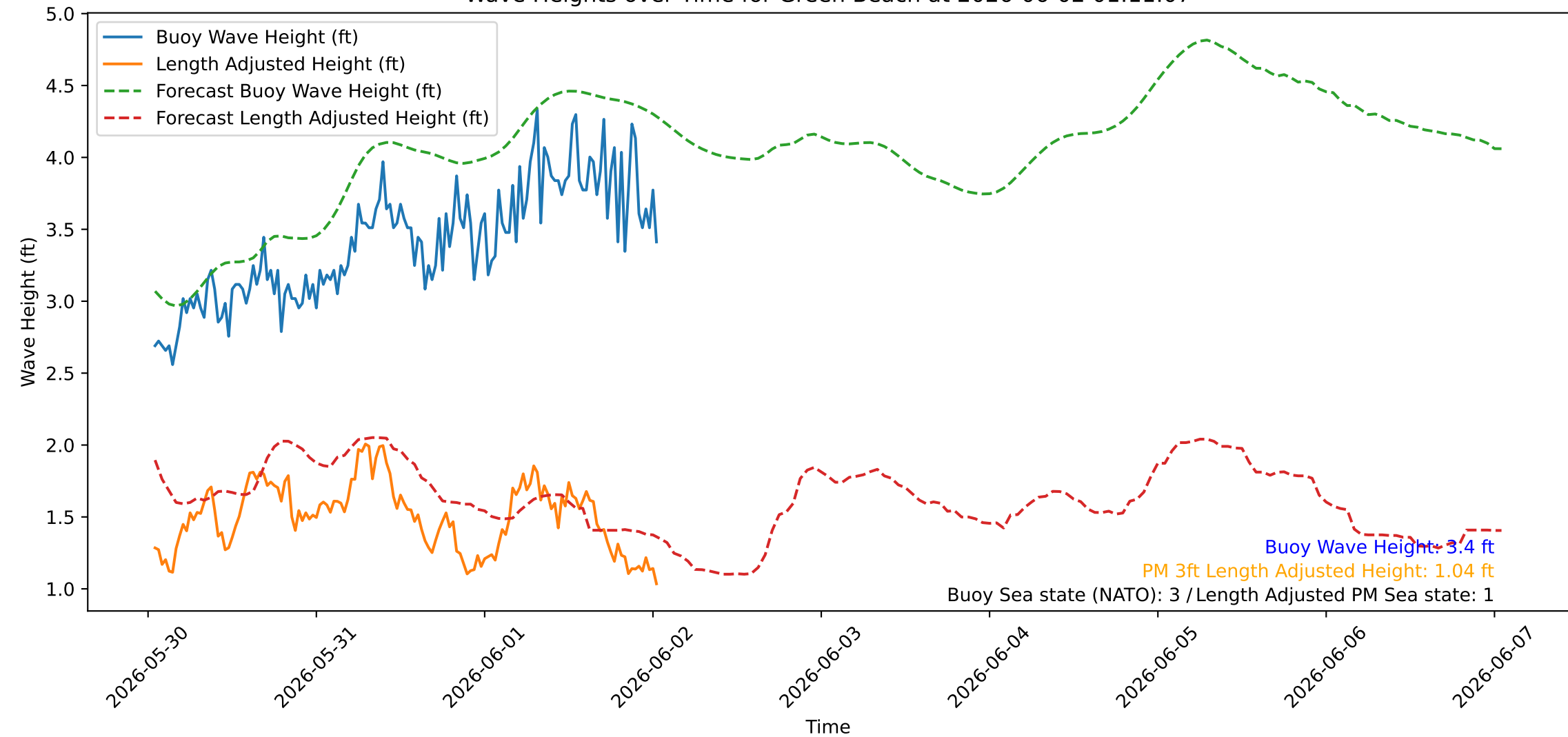
Wave Heights over Time for Green Beach at 2026-06-02 01:11:07
