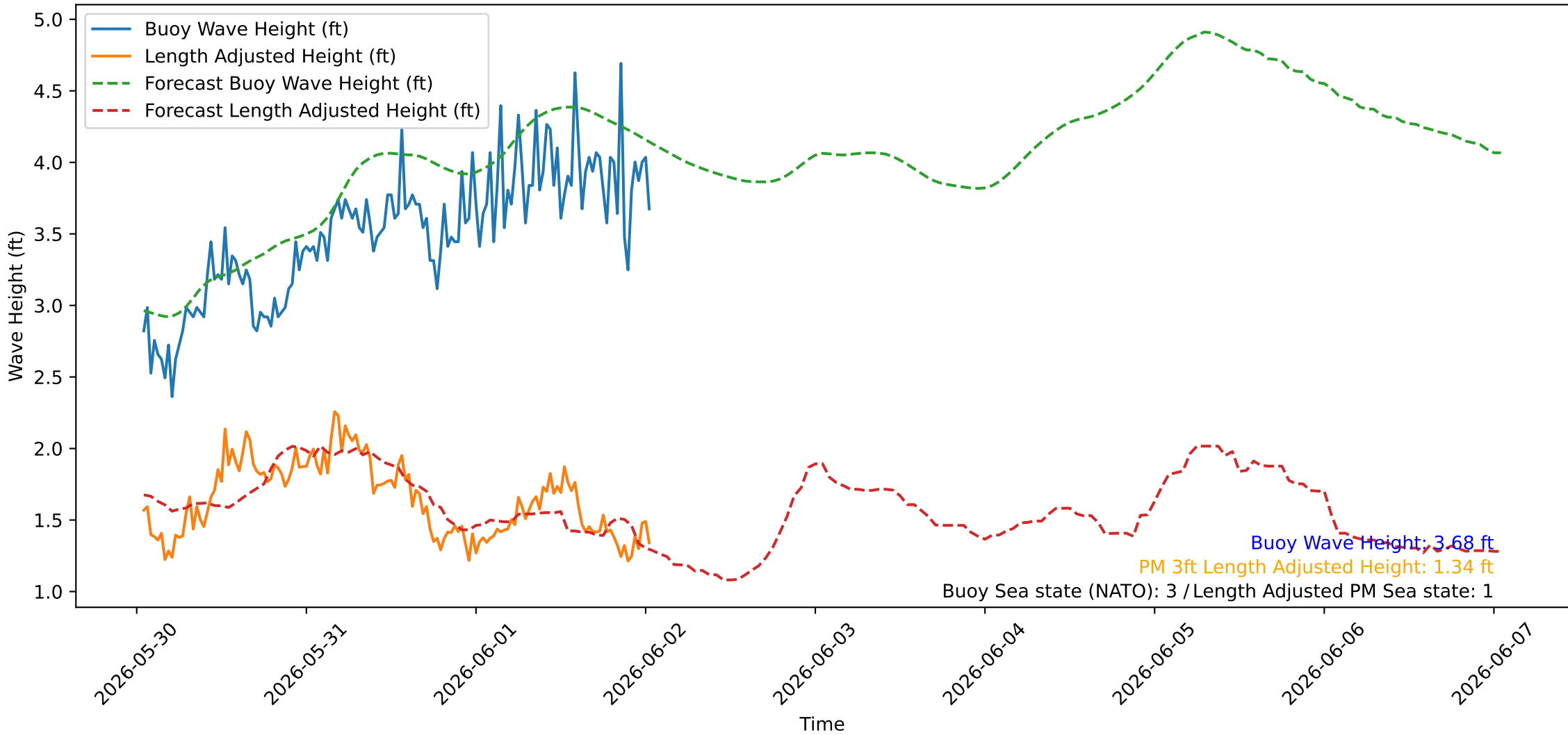
Wave Heights over Time for Oceanside Harbor at 2026-06-02 01:10:25
