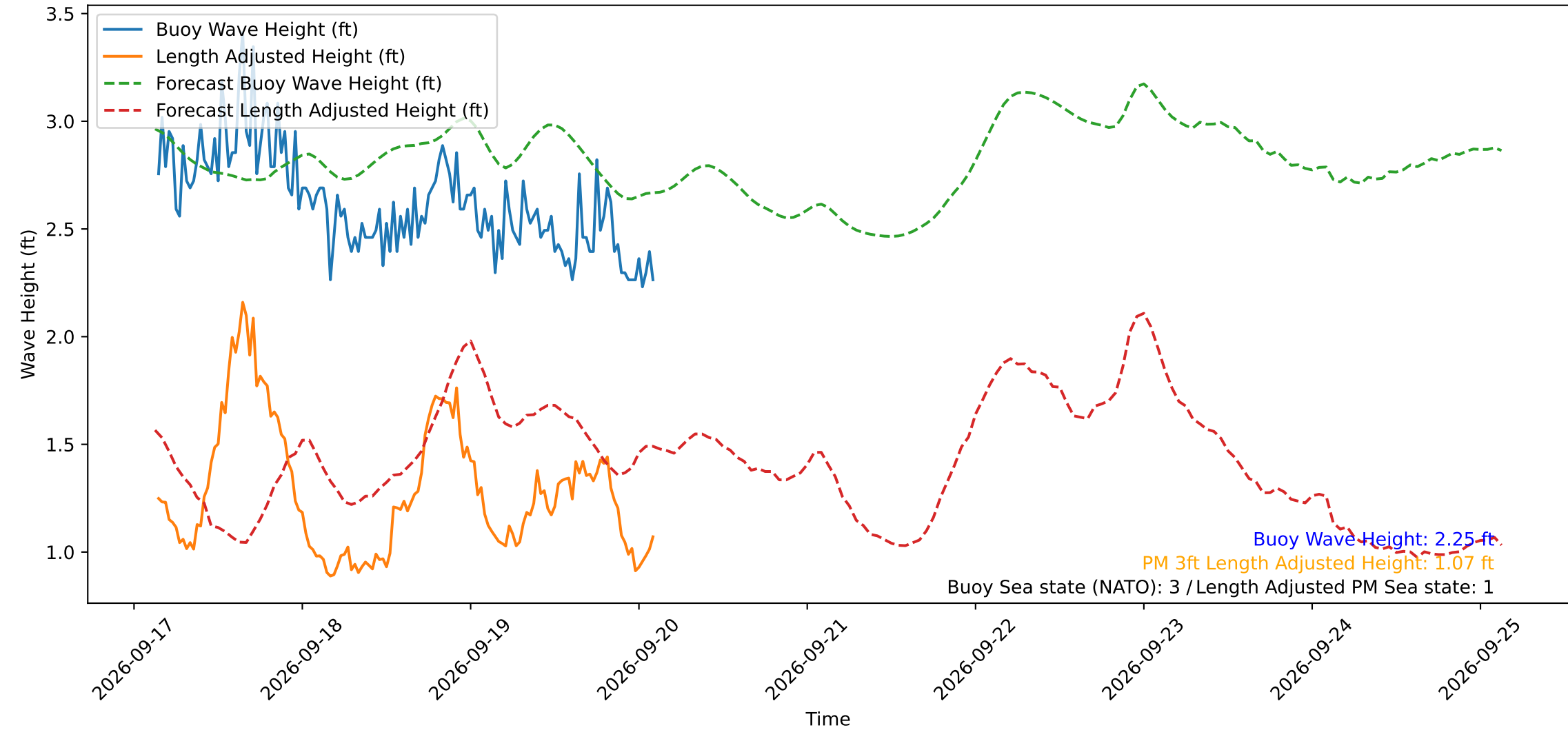
Wave Heights over Time for Red Beach at 2026-09-20 03:00:48
