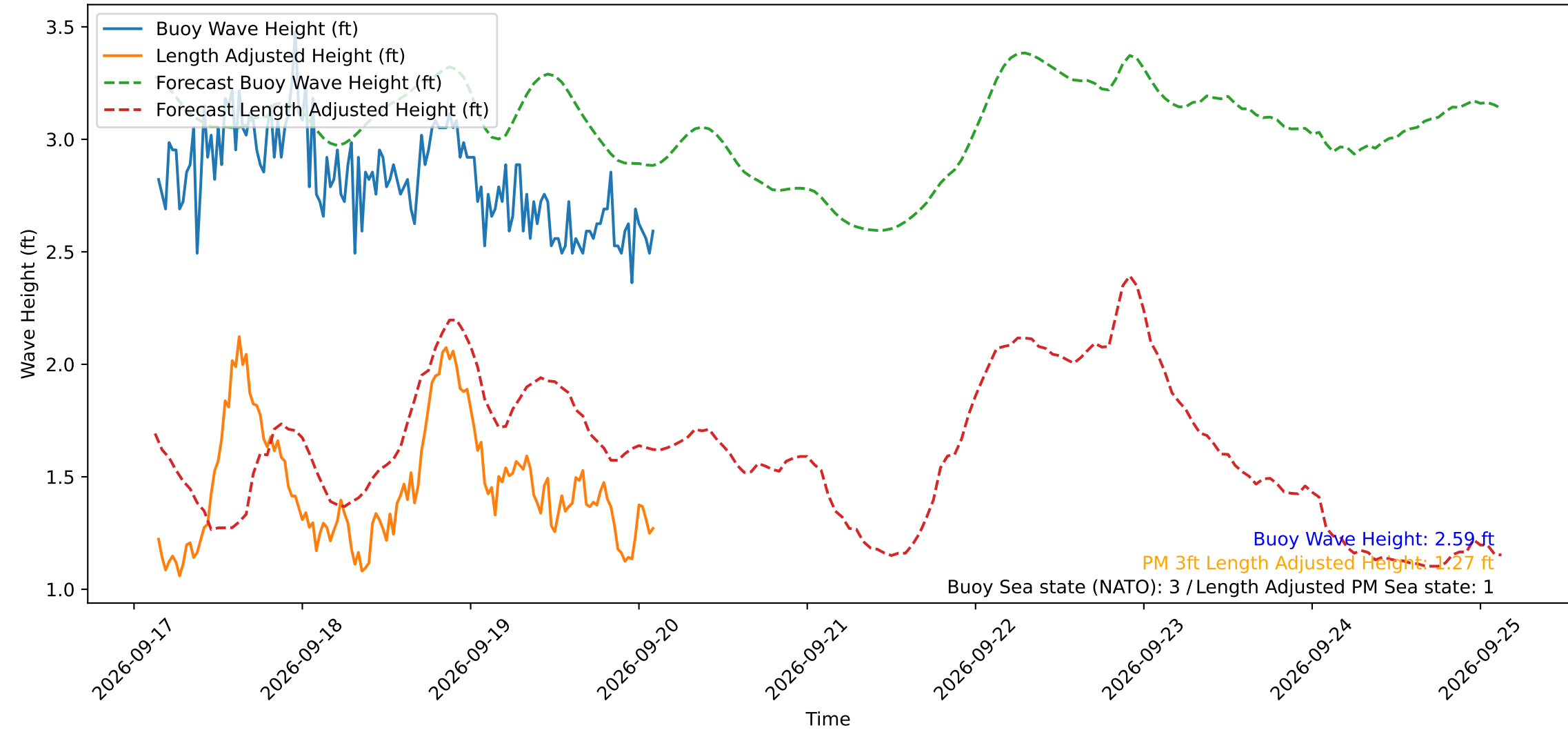
Wave Heights over Time for Green Beach at 2026-09-20 03:01:10
