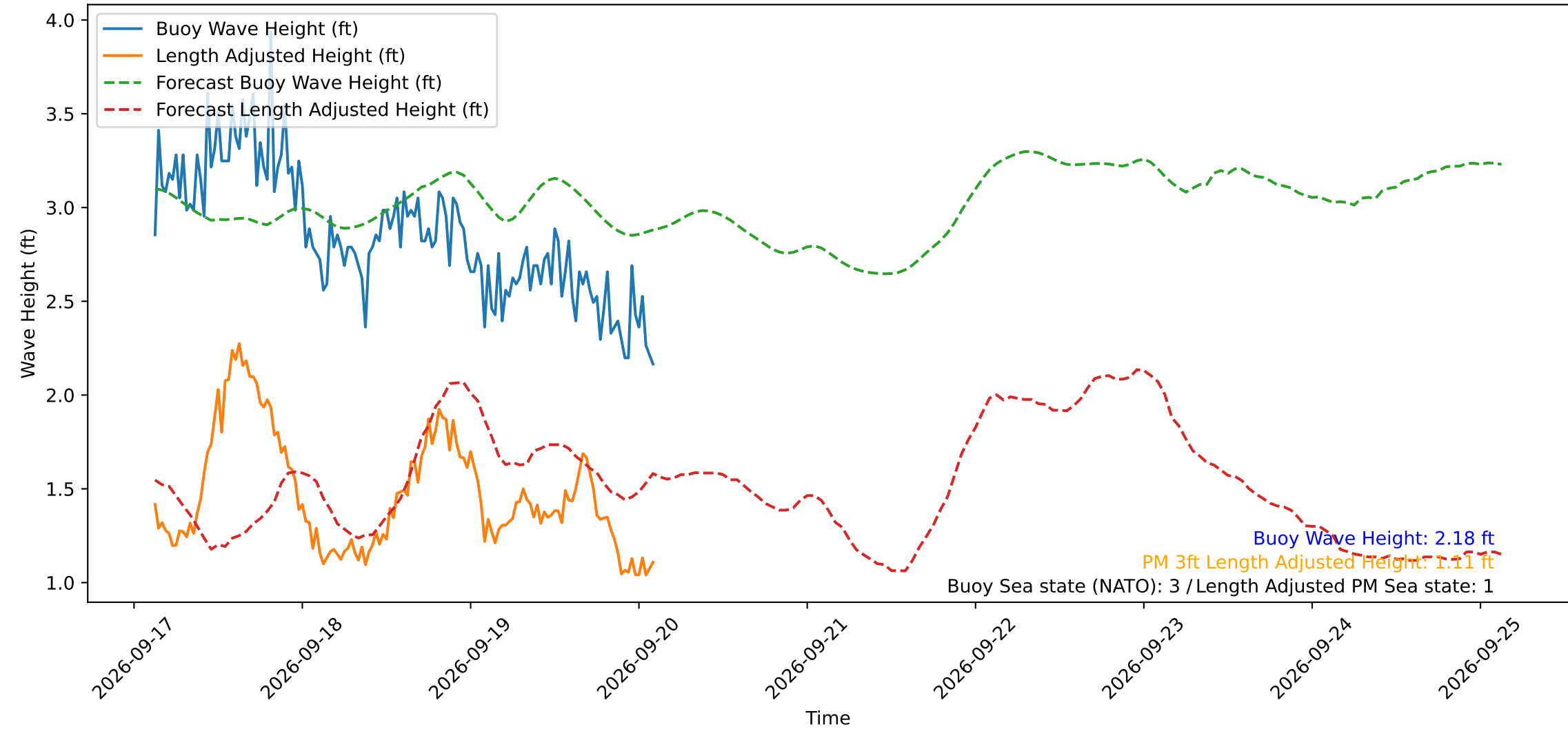
Wave Heights over Time for Oceanside Harbor at 2026-09-20 03:00:29
