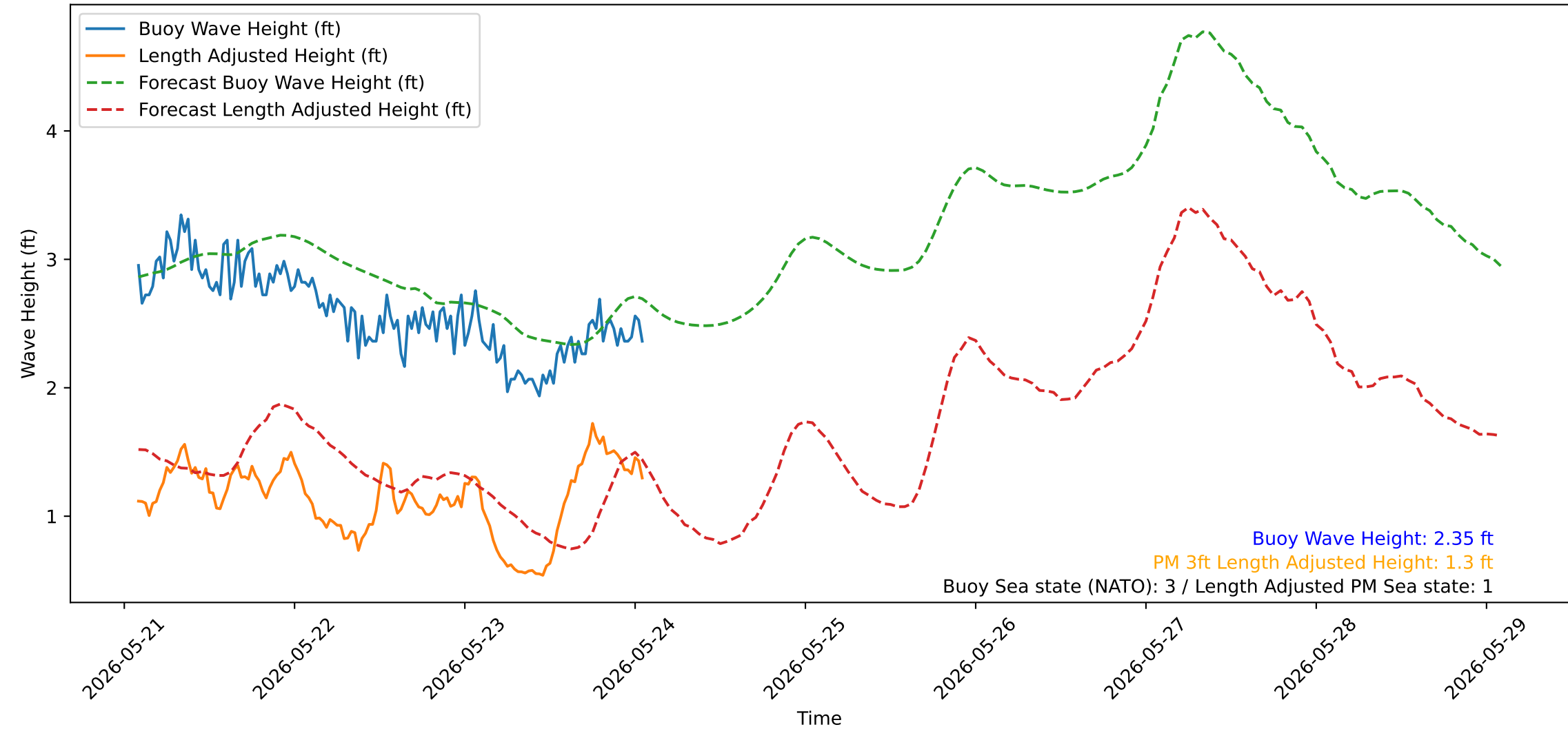
Wave Heights over Time for Red Beach at 2026-05-24 01:50:52
