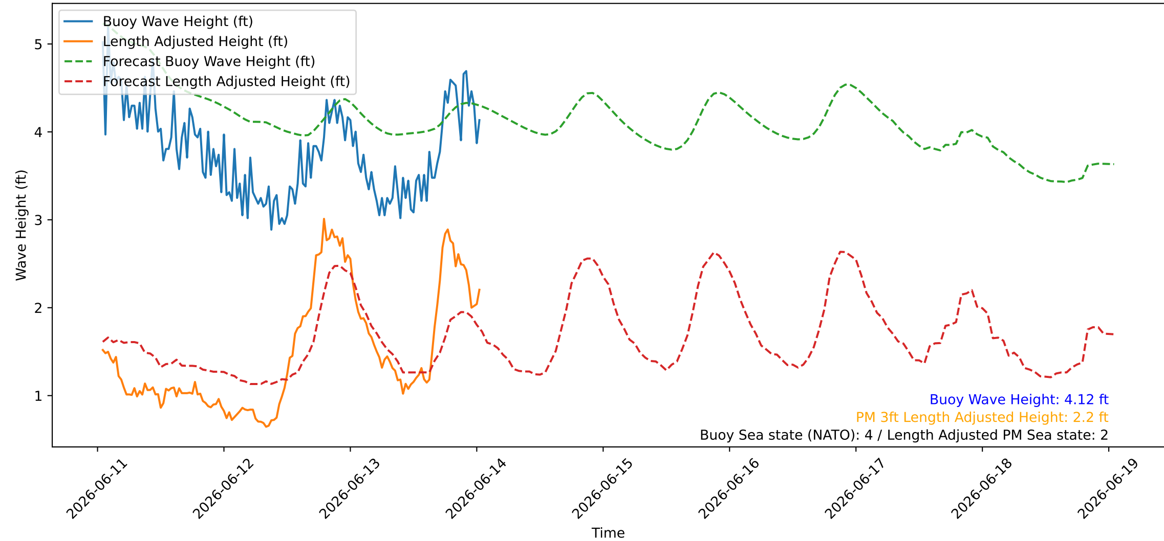
Wave Heights over Time for Green Beach at 2026-06-14 01:11:08
