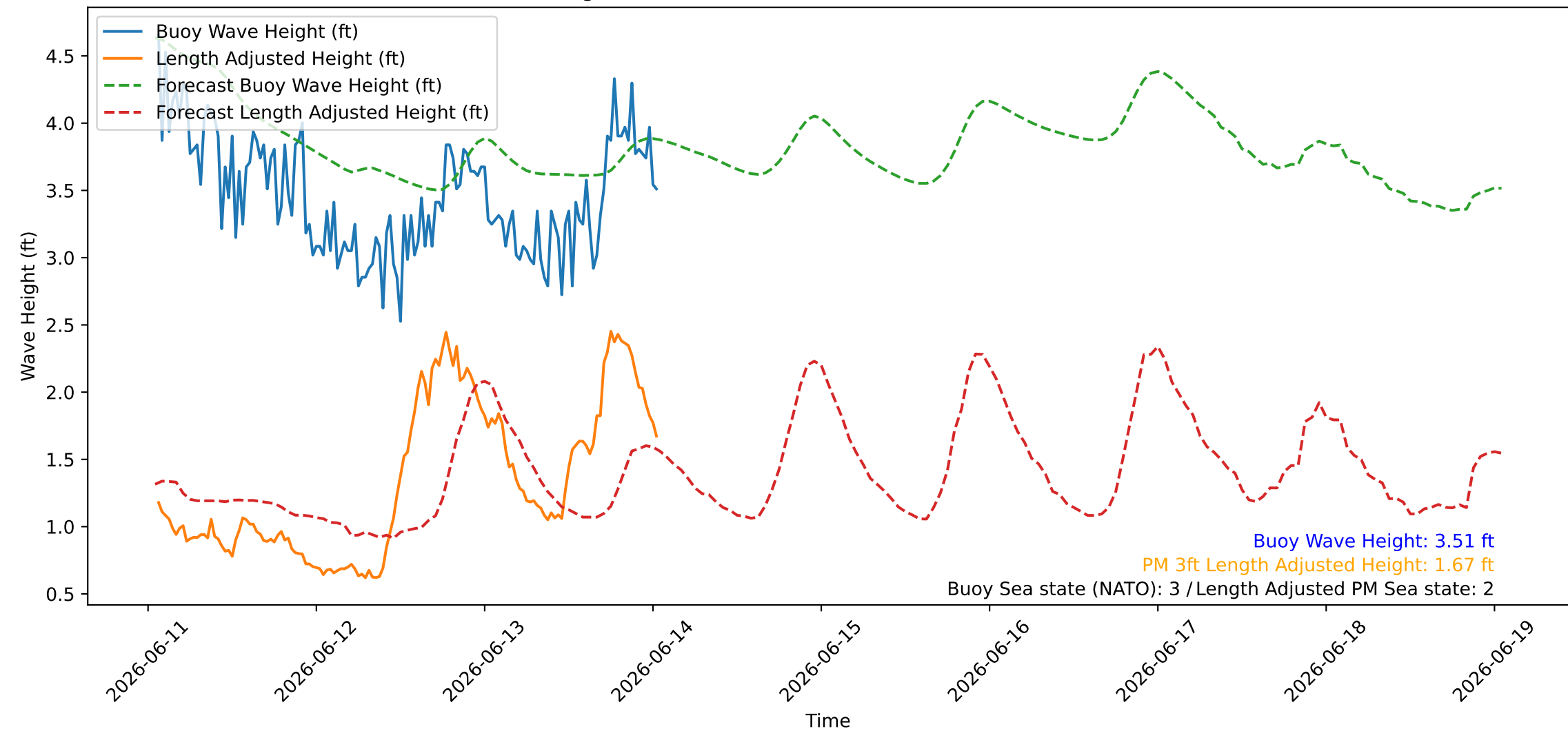
Wave Heights over Time for Red Beach at 2026-06-14 01:10:46
