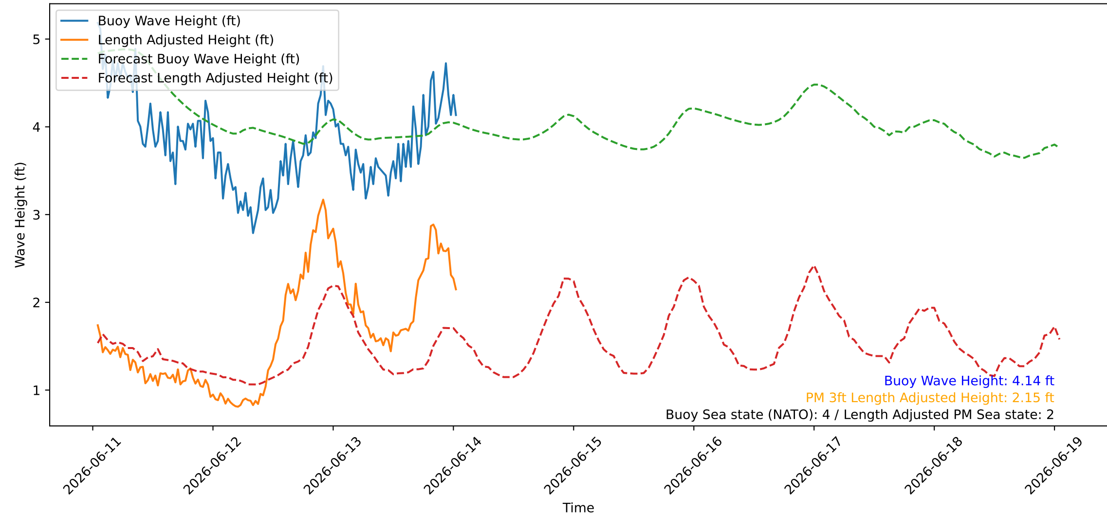
Wave Heights over Time for Oceanside Harbor at 2026-06-14 01:10:26
