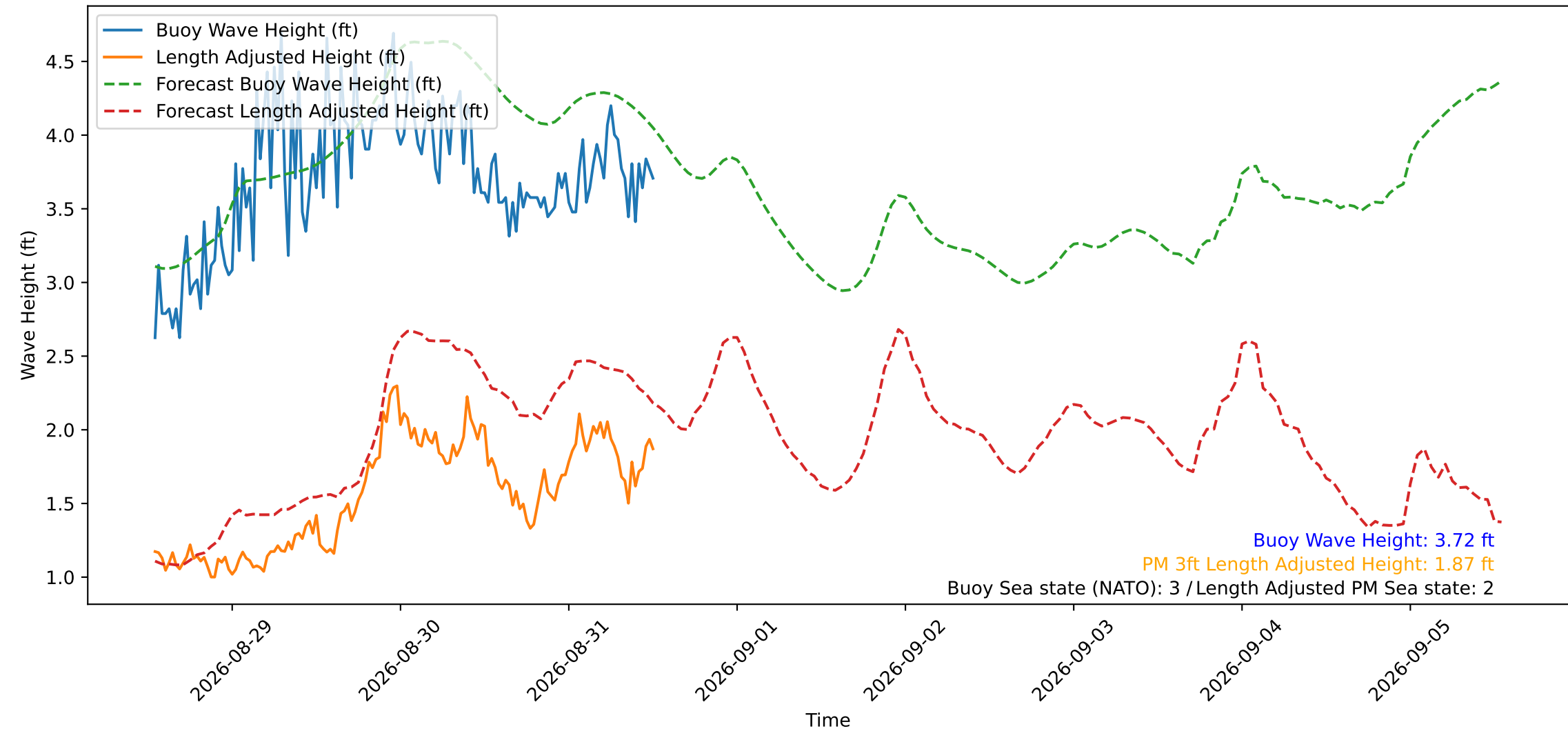
Wave Heights over Time for Red Beach at 2026-08-31 12:50:51
