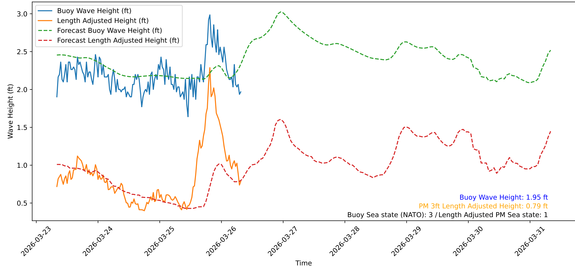
Wave Heights over Time for Green Beach at 2026-03-26 08:12:55
