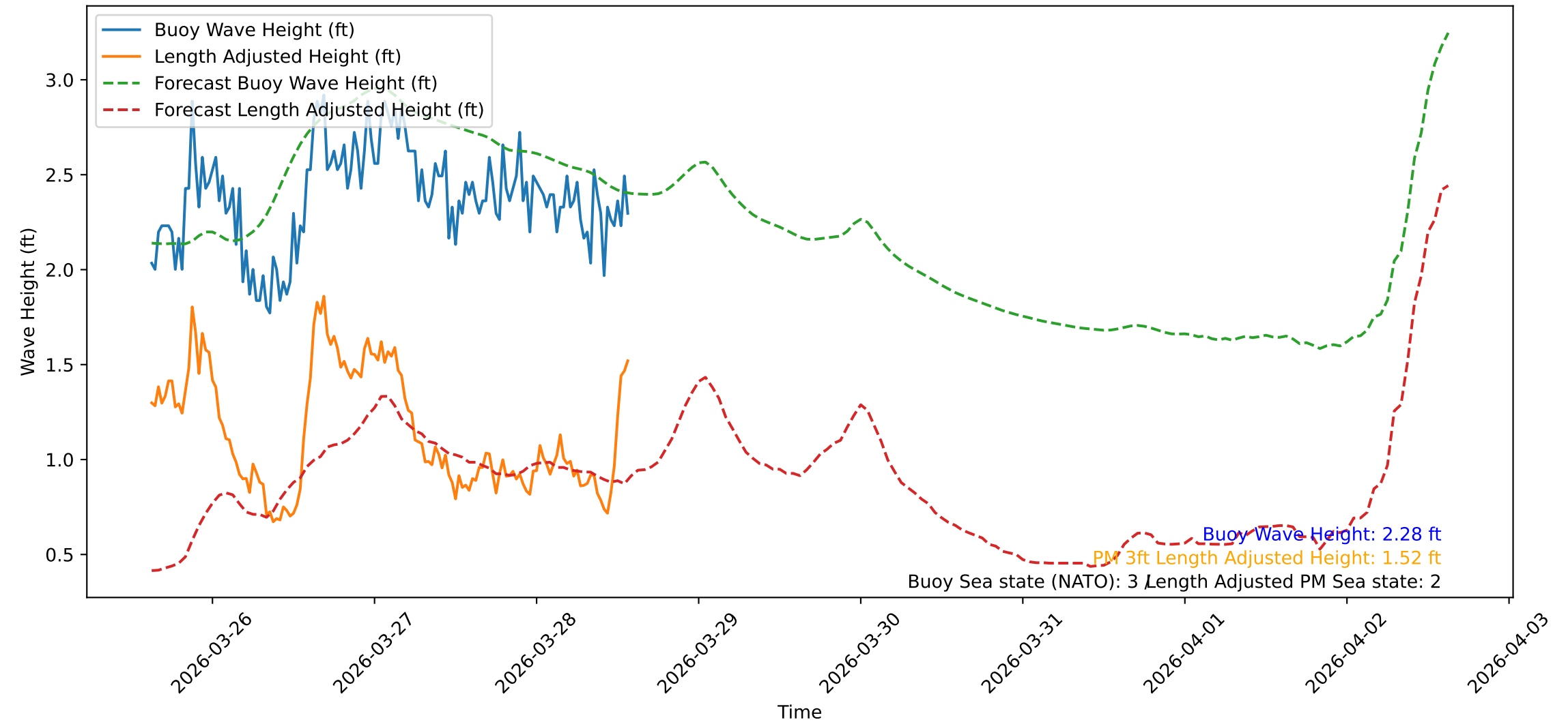
Wave Heights over Time for Oceanside Harbor at 2026-03-28 15:10:31
