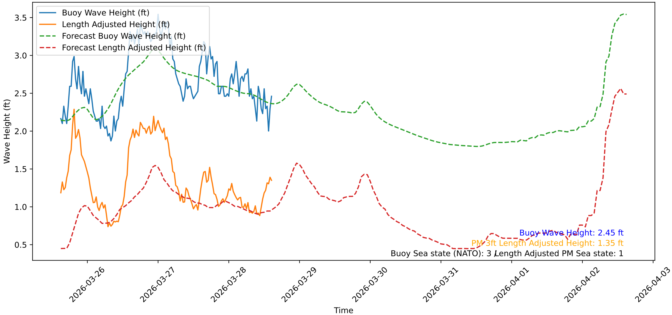
Wave Heights over Time for Green Beach at 2026-03-28 15:11:09
