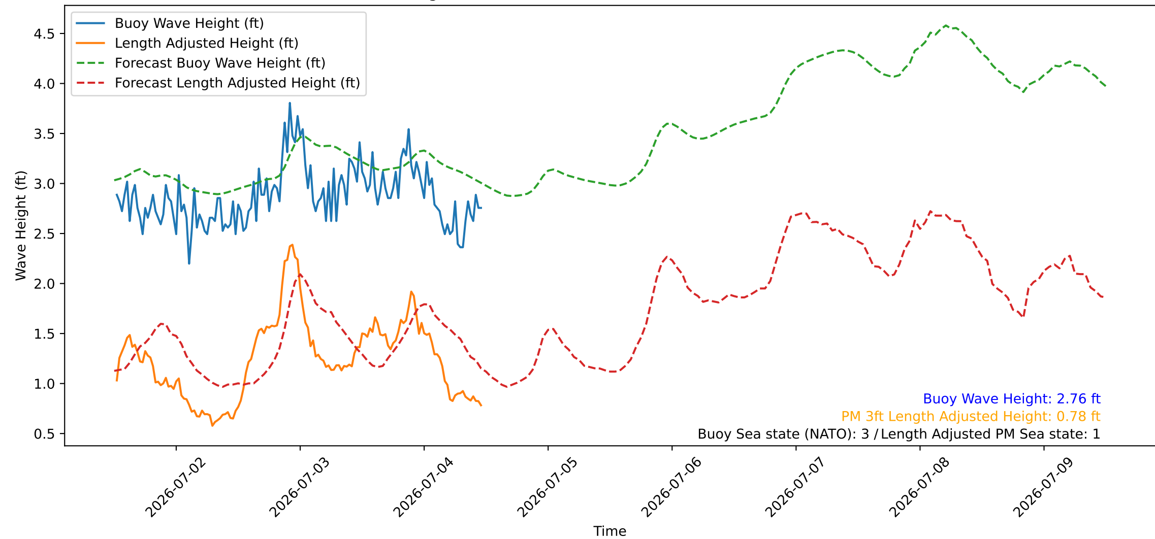
Wave Heights over Time for Red Beach at 2026-07-04 12:00:45
