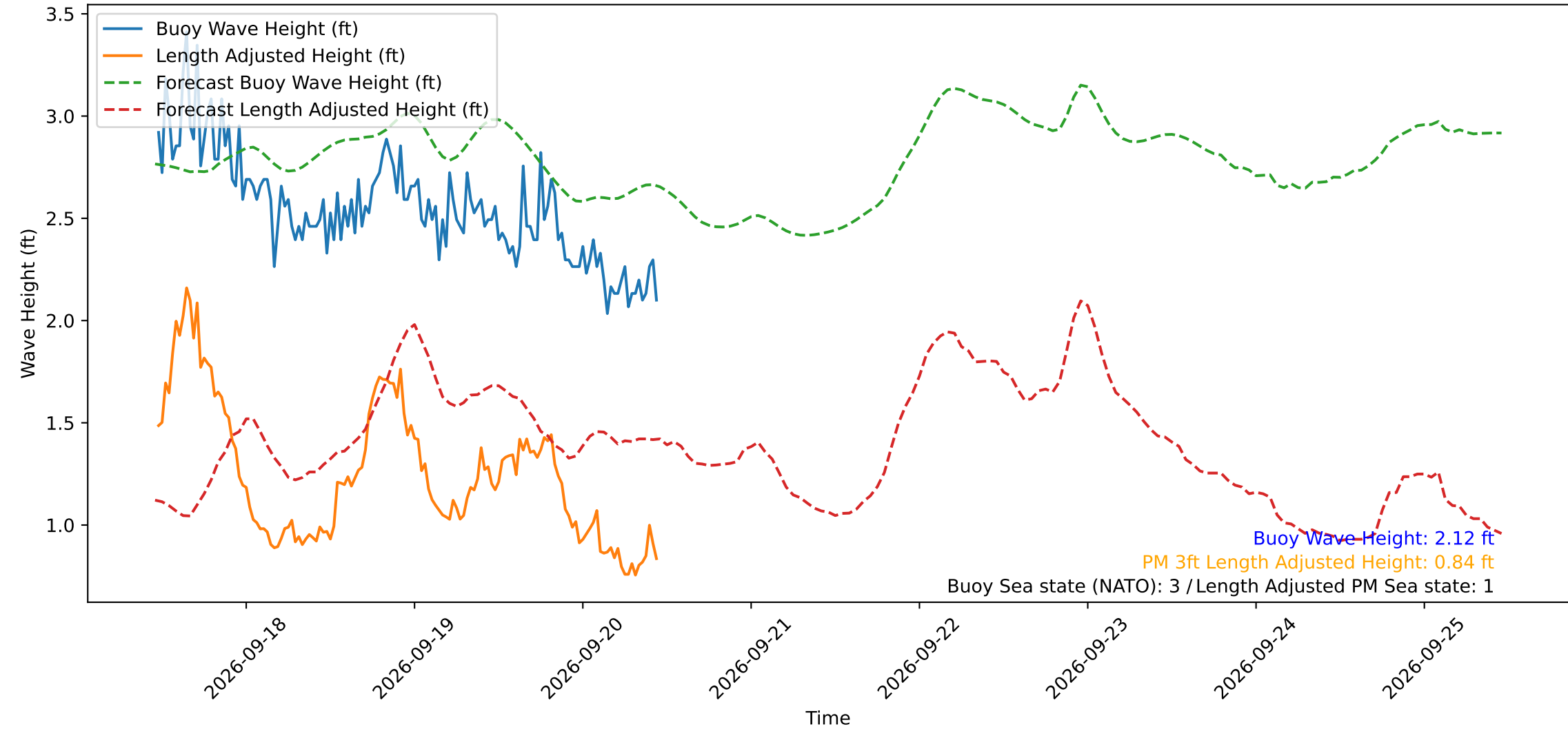
Wave Heights over Time for Red Beach at 2026-09-20 11:20:51
