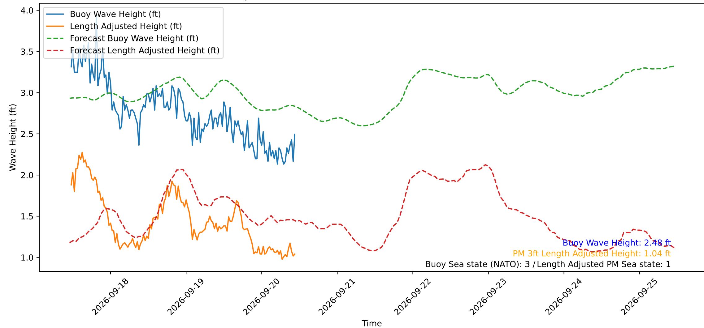
Wave Heights over Time for Oceanside Harbor at 2026-09-20 11:20:30
