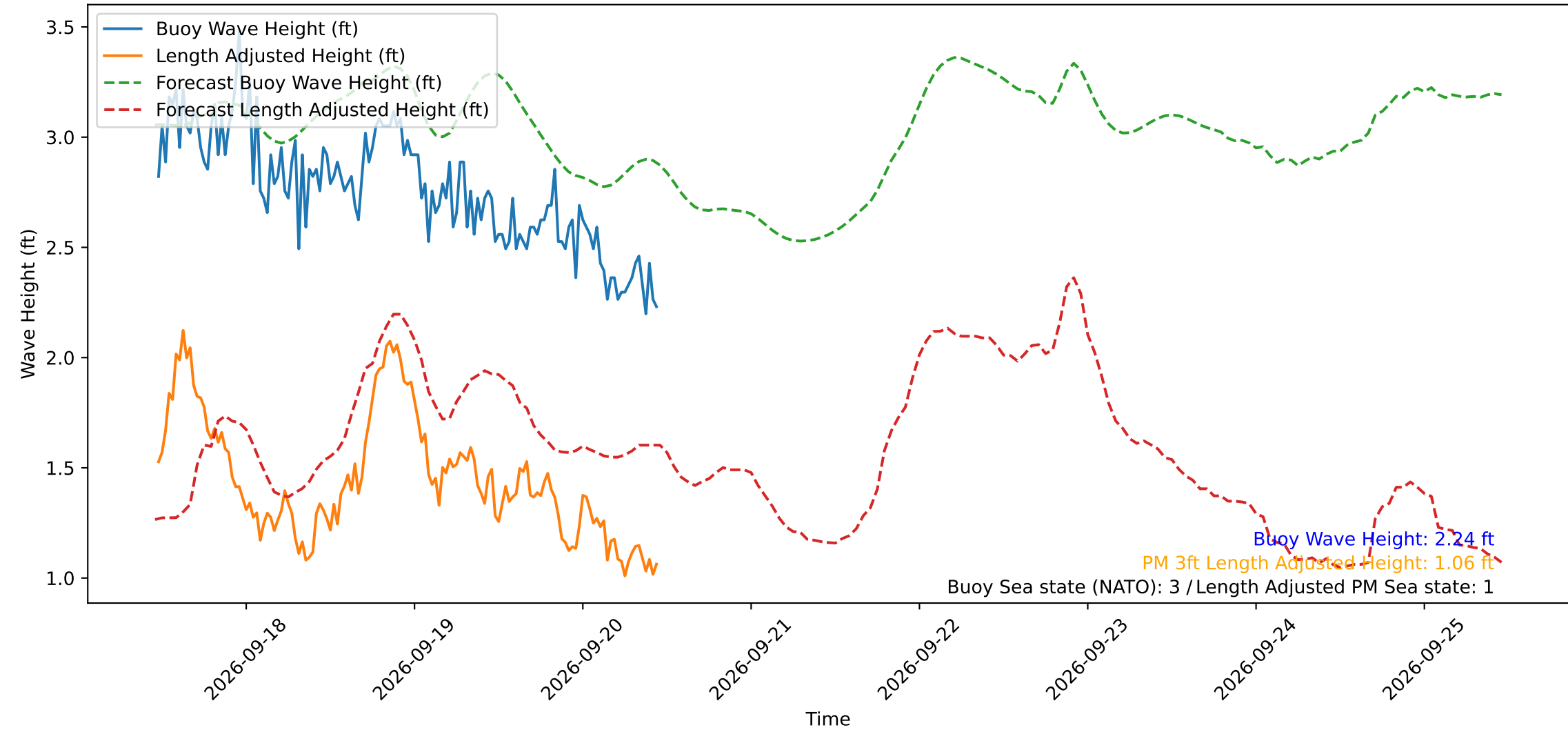
Wave Heights over Time for Green Beach at 2026-09-20 11:21:15
