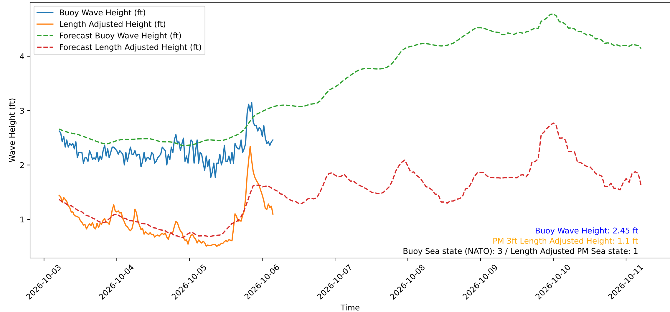
Wave Heights over Time for Green Beach at 2026-10-06 04:31:12
