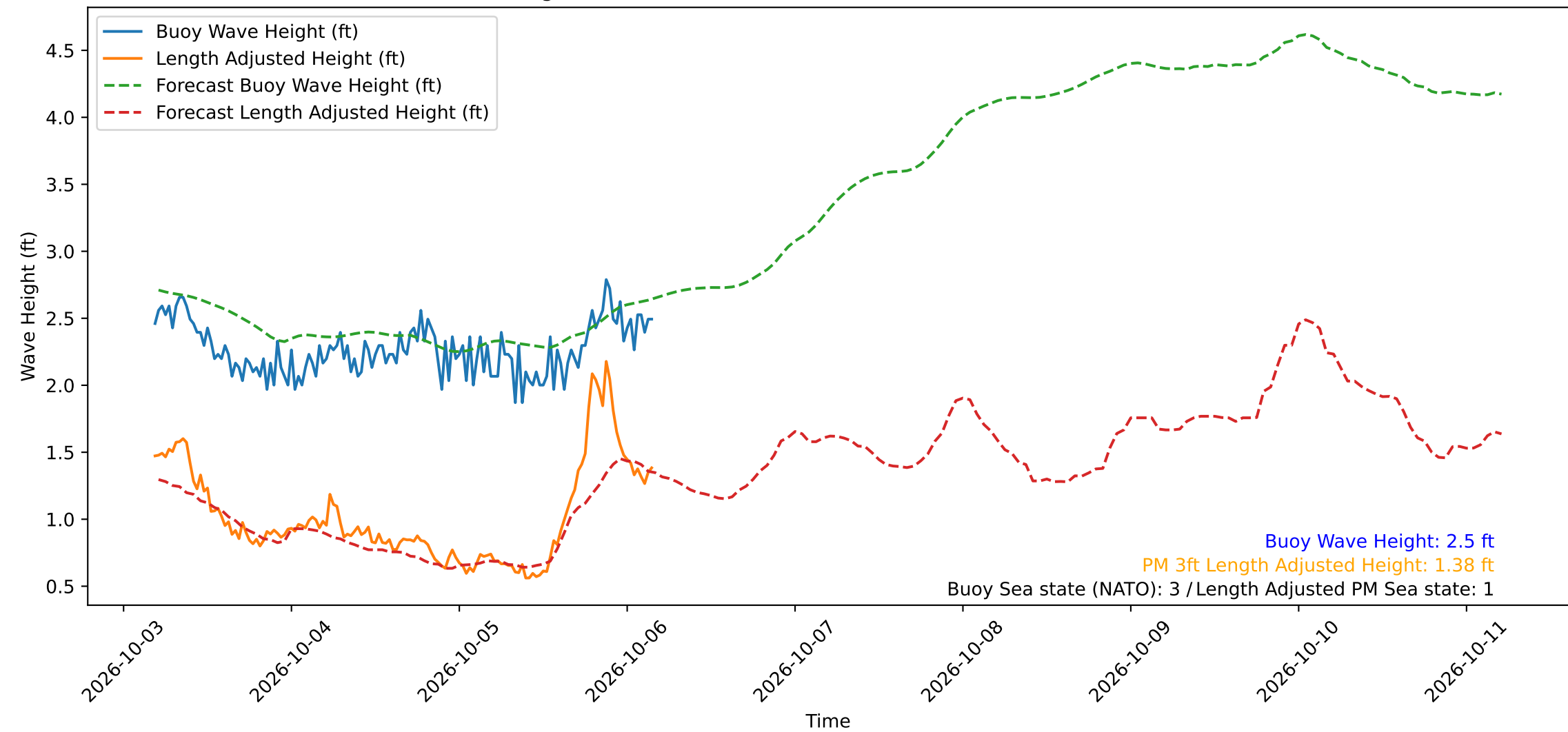
Wave Heights over Time for Oceanside Harbor at 2026-10-06 04:30:29
