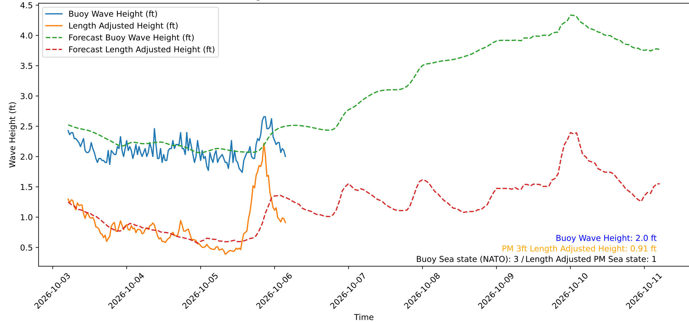
Wave Heights over Time for Red Beach at 2026-10-06 04:30:50
