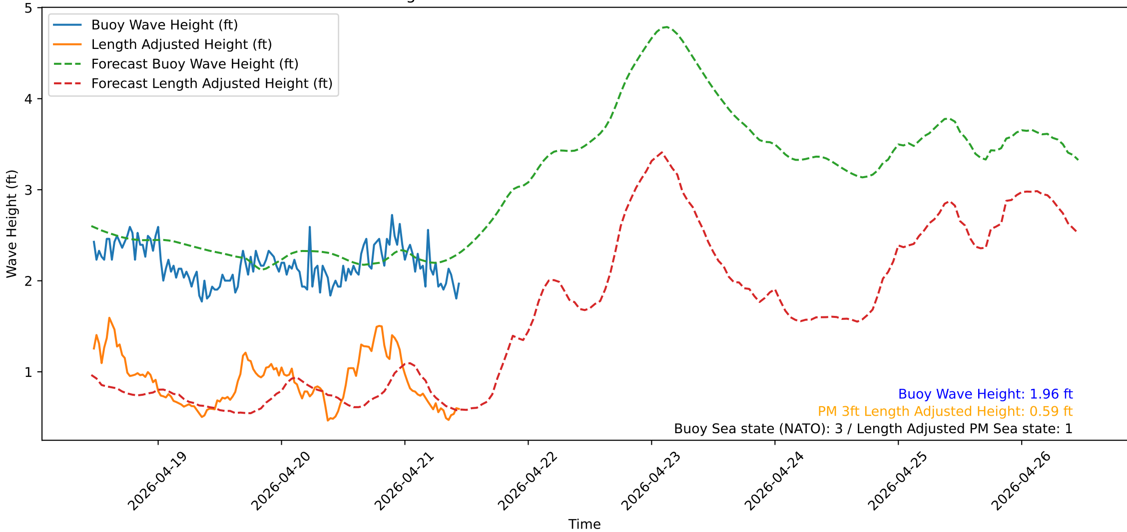
Wave Heights over Time for Red Beach at 2026-04-21 11:20:52
