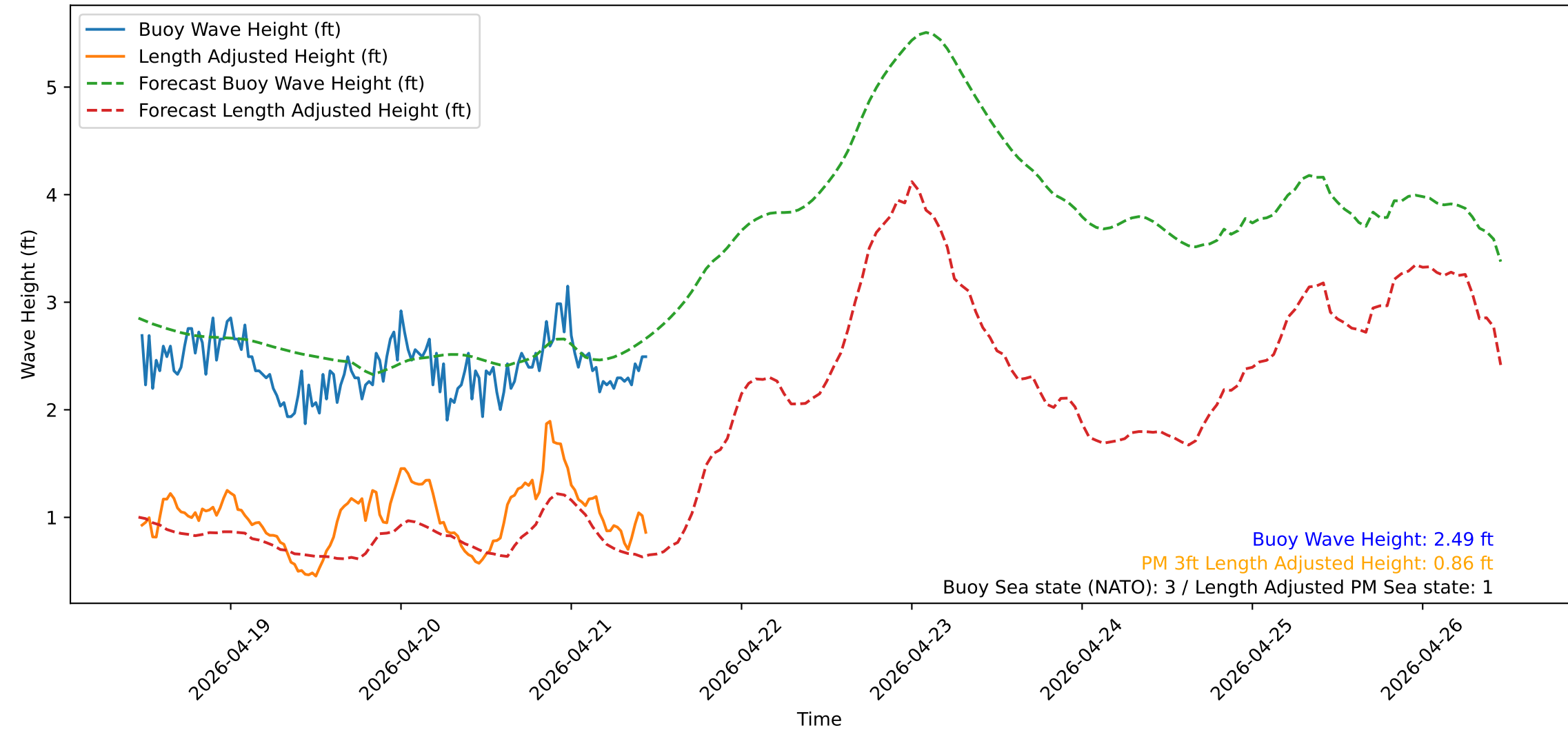
Wave Heights over Time for Green Beach at 2026-04-21 11:21:15
