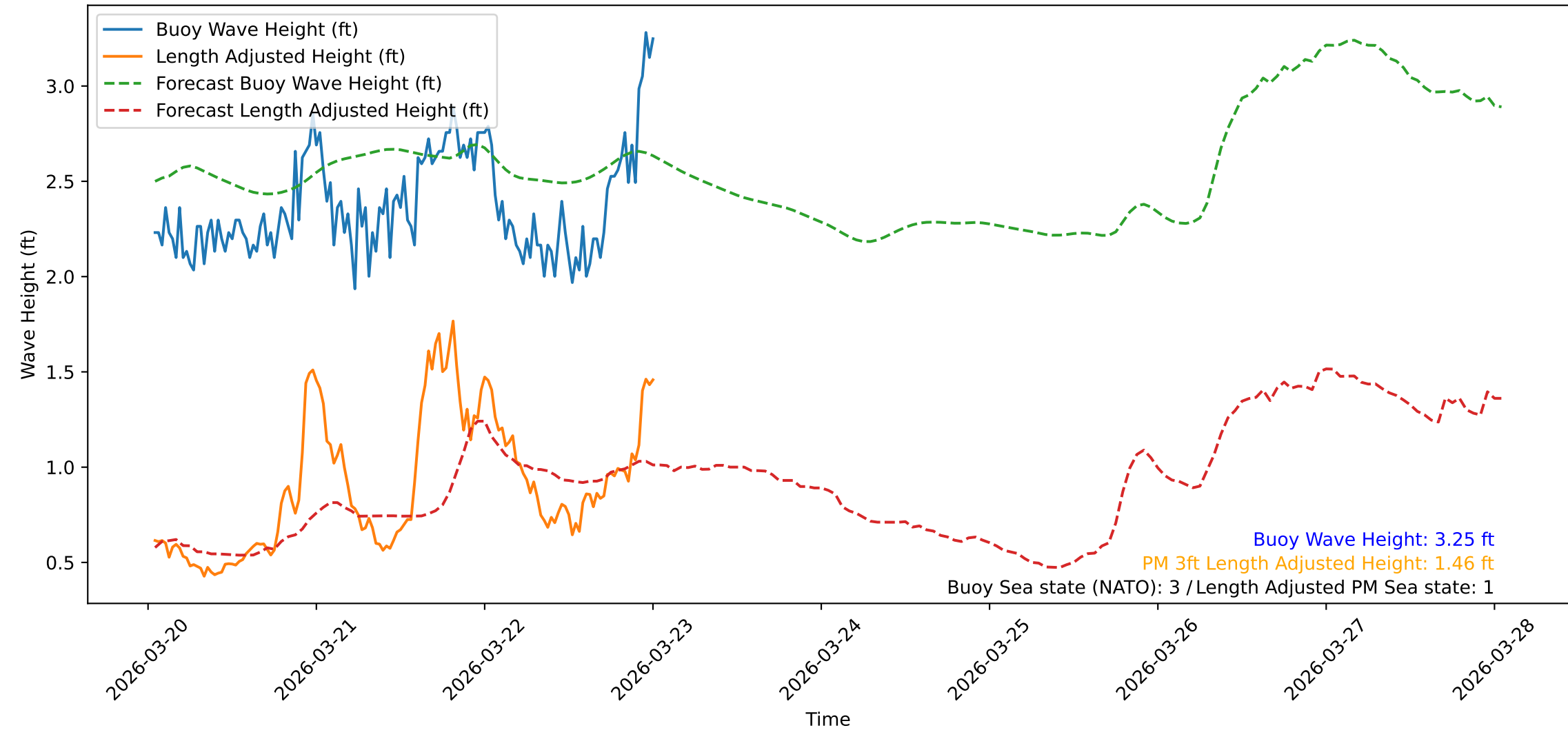
Wave Heights over Time for Green Beach at 2026-03-23 00:51:10
