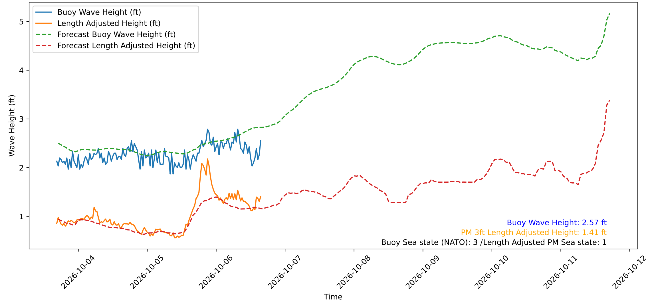
Wave Heights over Time for Oceanside Harbor at 2026-10-06 16:30:30
