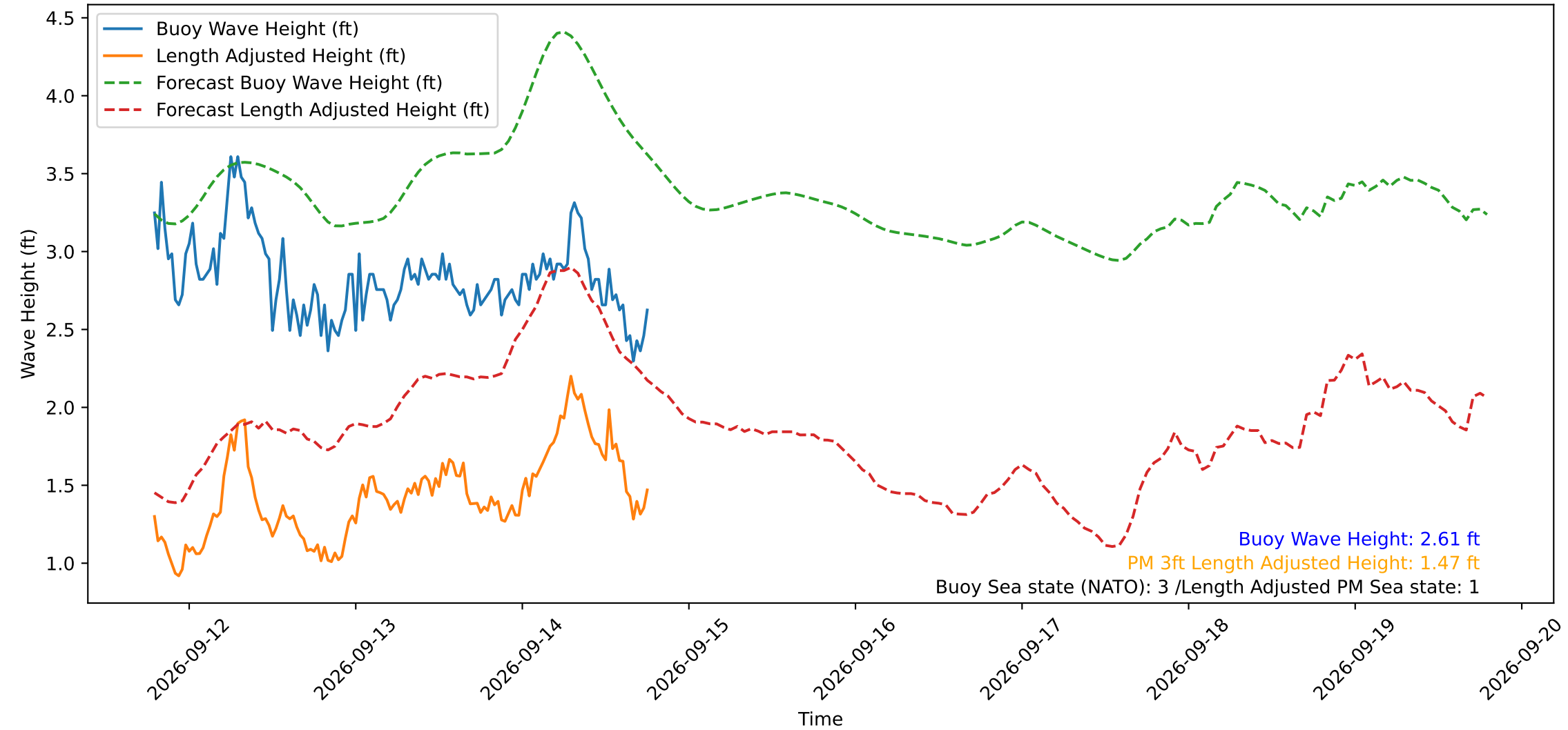
Wave Heights over Time for Green Beach at 2026-09-14 18:51:14
