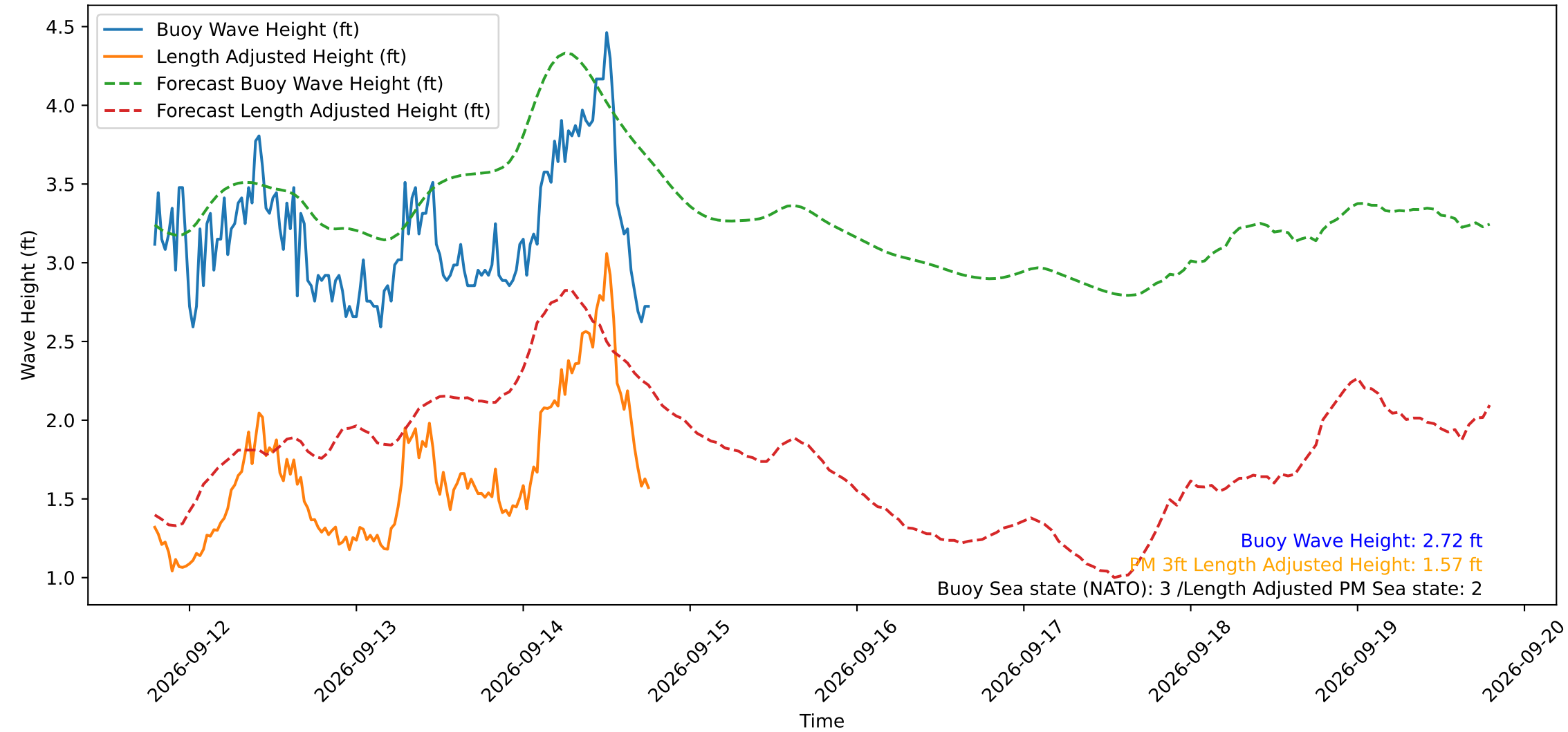
Wave Heights over Time for Oceanside Harbor at 2026-09-14 18:50:29
