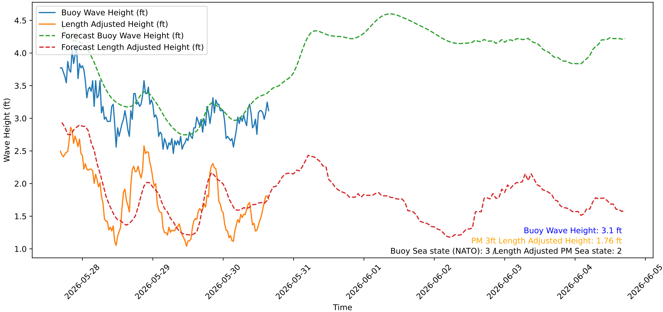
Wave Heights over Time for Green Beach at 2026-05-30 16:31:05
