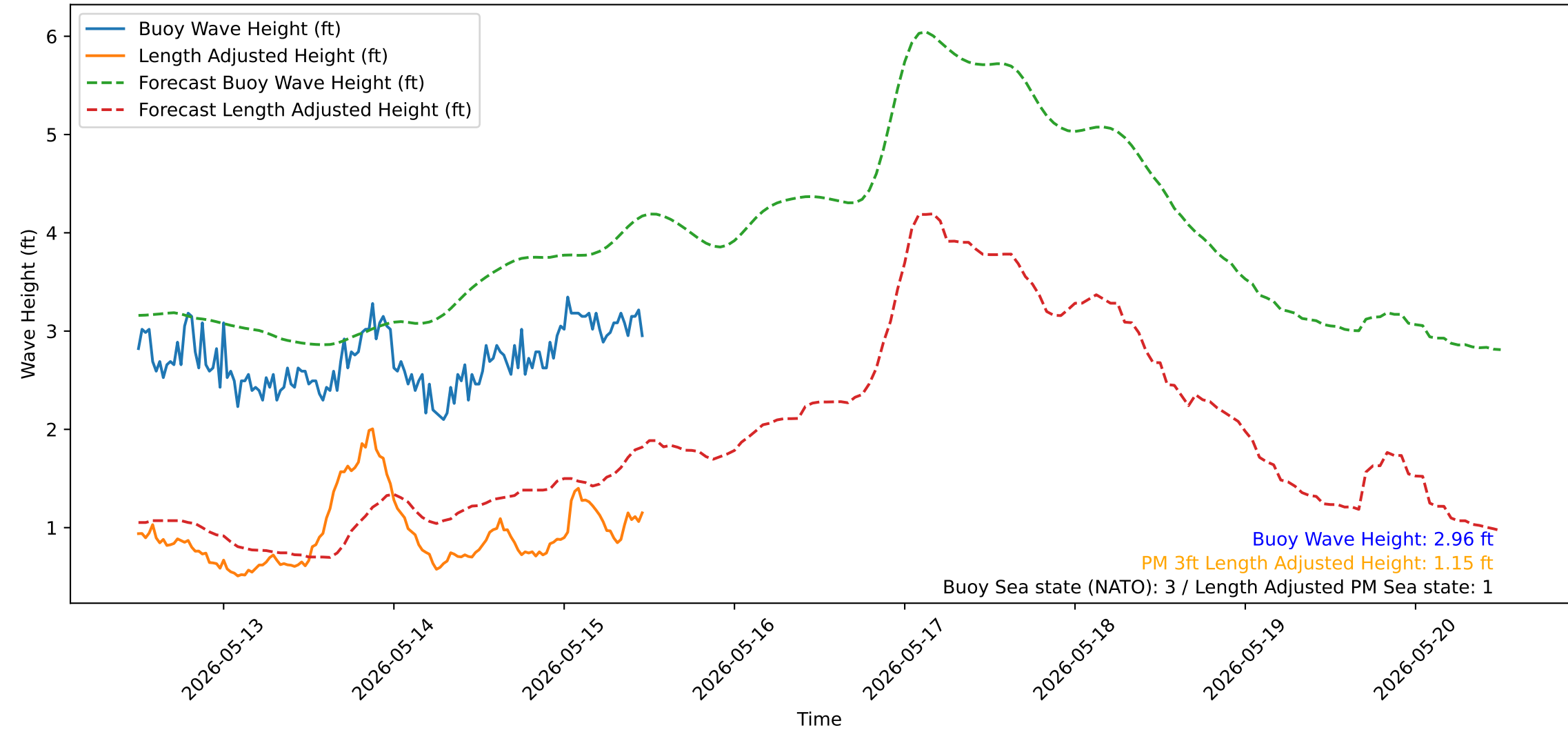
Wave Heights over Time for Green Beach at 2026-05-15 11:51:14
