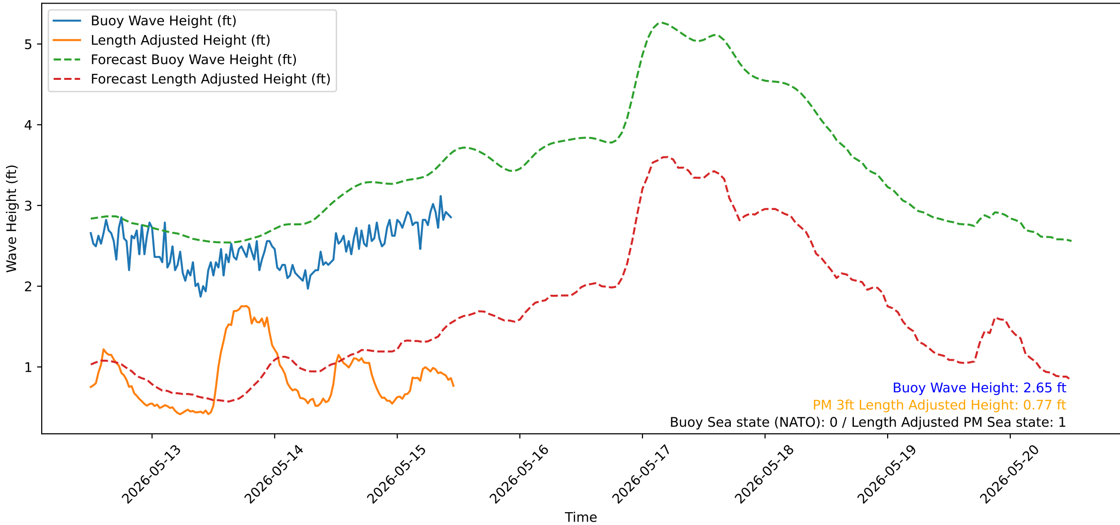
Wave Heights over Time for Red Beach at 2026-05-15 11:50:52
