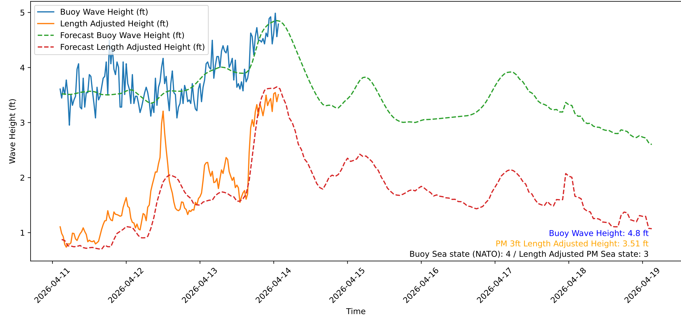
Wave Heights over Time for Green Beach at 2026-04-14 02:31:12
