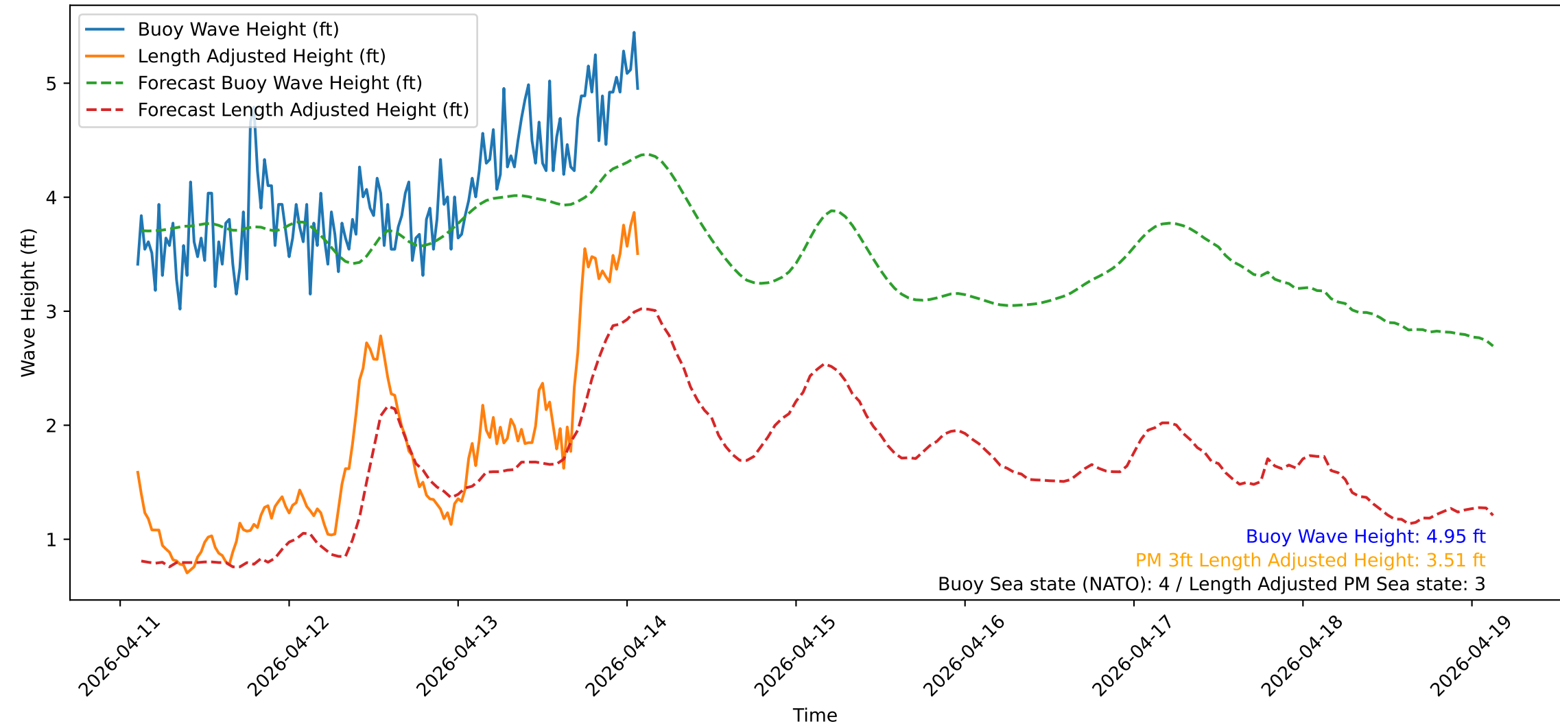
Wave Heights over Time for Oceanside Harbor at 2026-04-14 02:30:31
