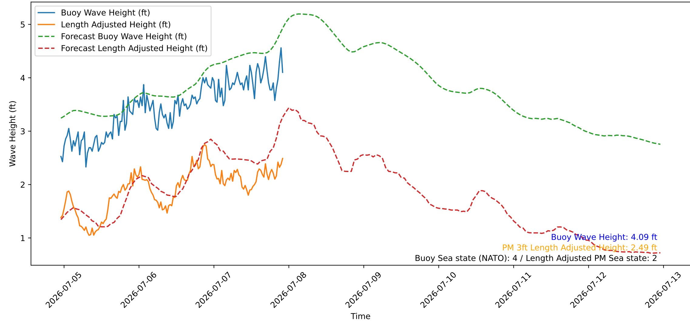
Wave Heights over Time for Oceanside Harbor at 2026-07-07 22:50:27
