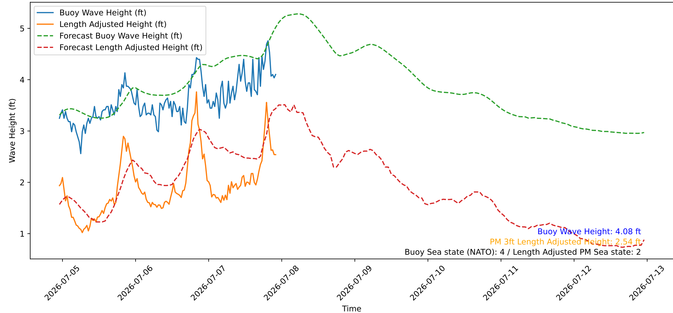
Wave Heights over Time for Green Beach at 2026-07-07 22:51:10
