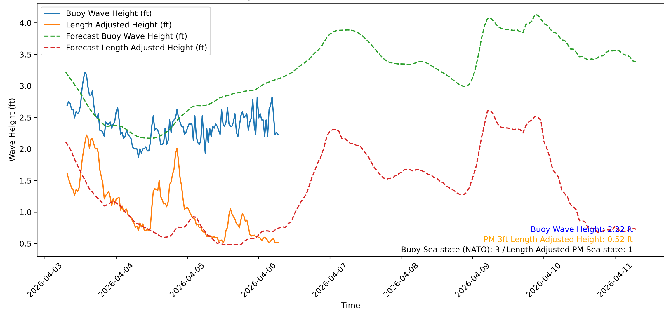
Wave Heights over Time for Red Beach at 2026-04-06 07:10:48
