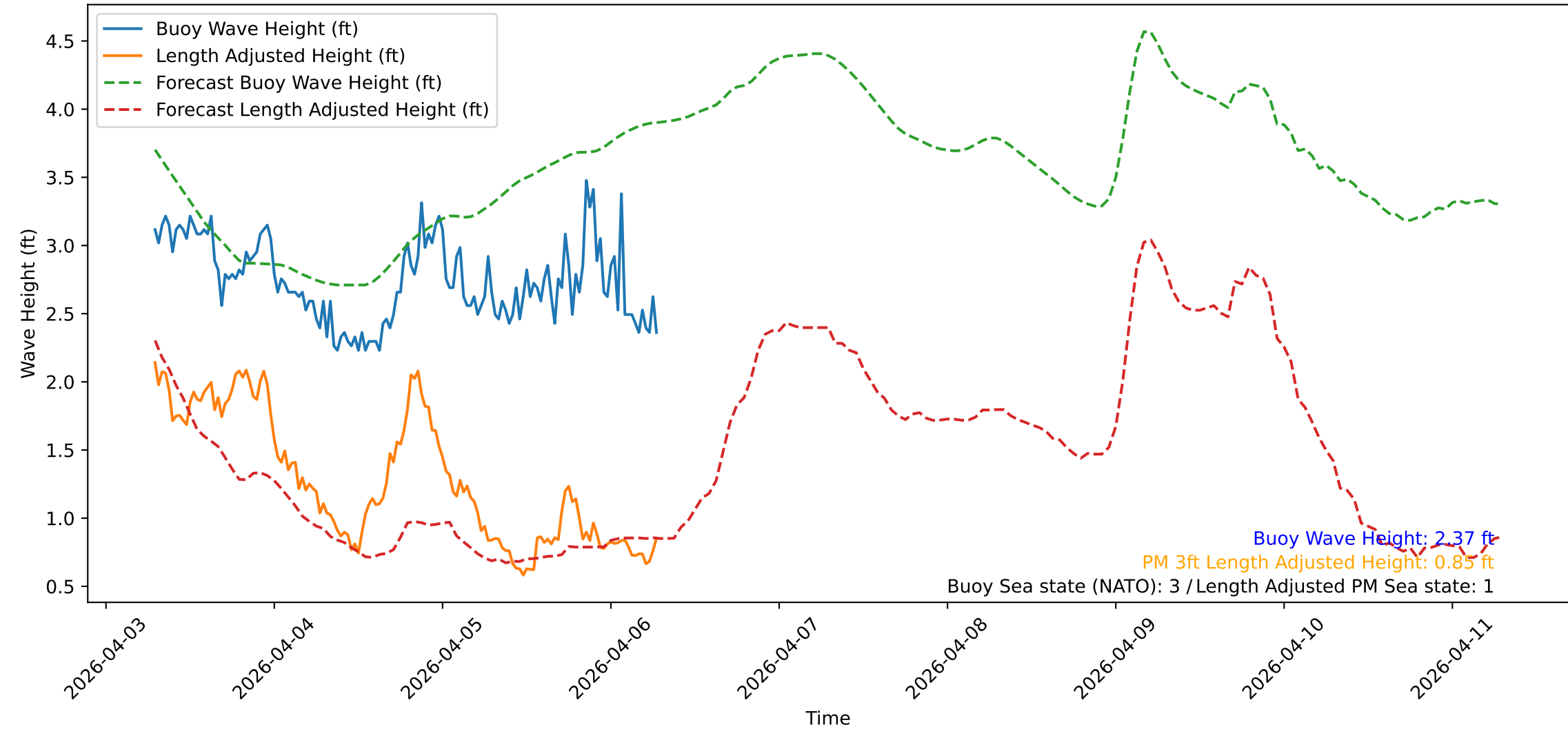
Wave Heights over Time for Green Beach at 2026-04-06 07:11:10
