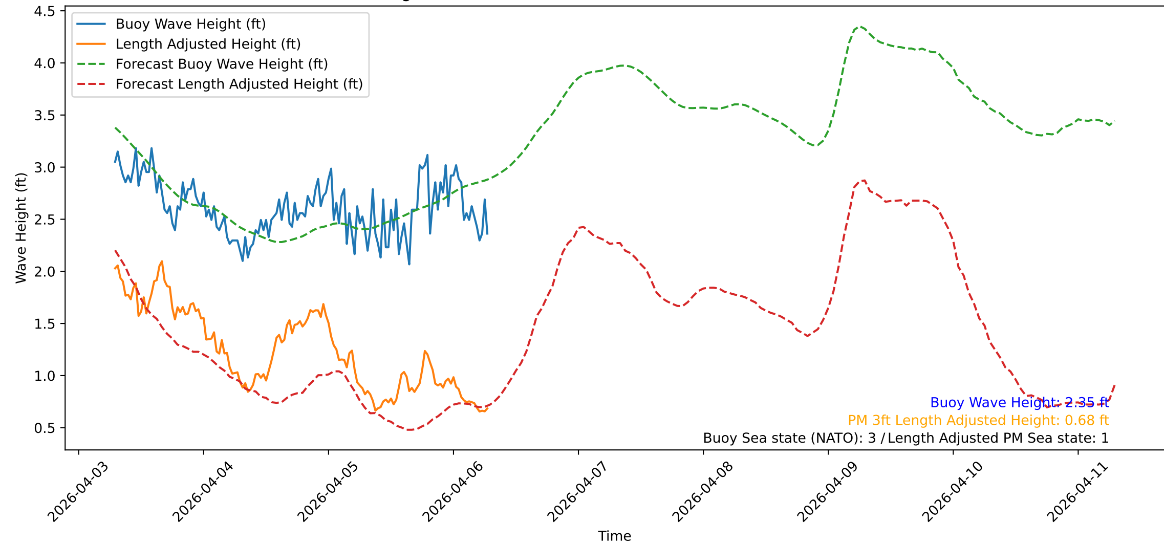
Wave Heights over Time for Oceanside Harbor at 2026-04-06 07:10:31
