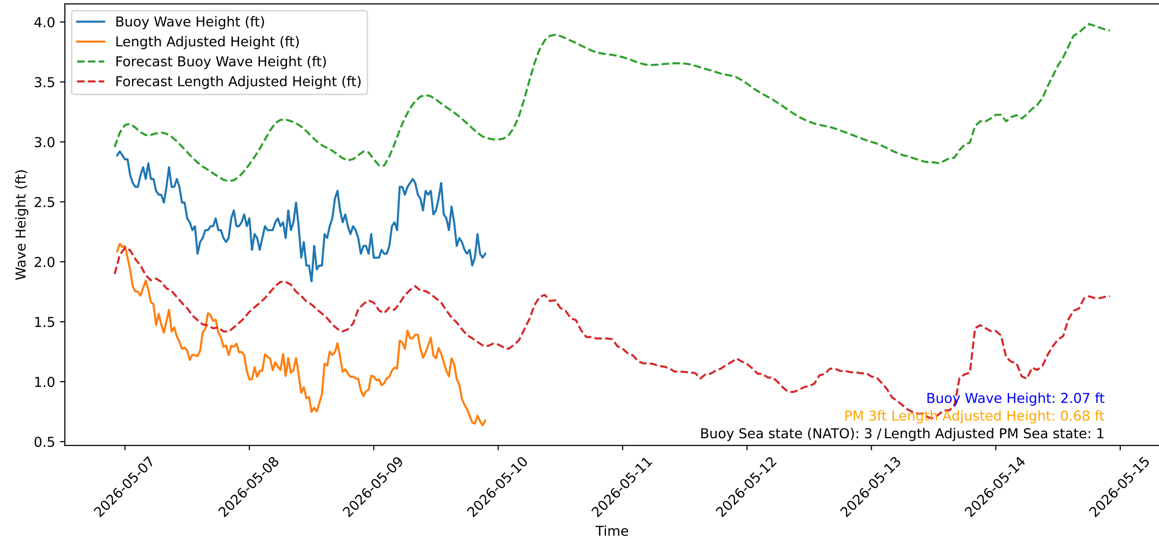
Wave Heights over Time for Green Beach at 2026-05-09 22:21:20
