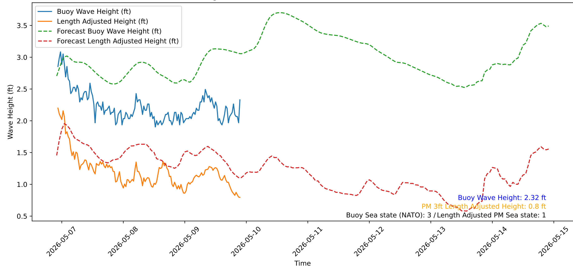
Wave Heights over Time for Red Beach at 2026-05-09 22:20:56
