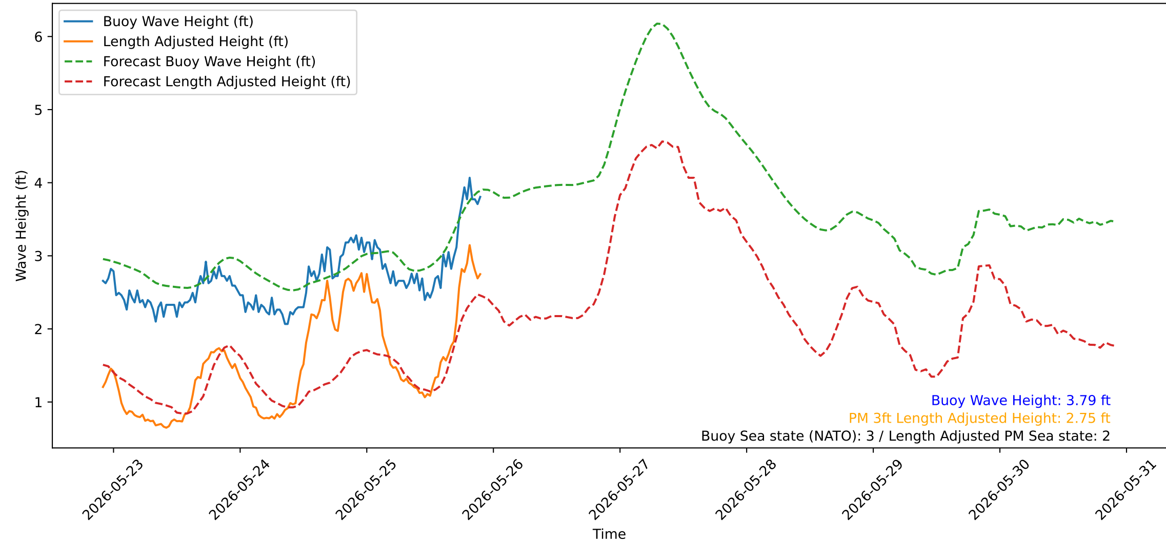
Wave Heights over Time for Green Beach at 2026-05-25 22:11:11
