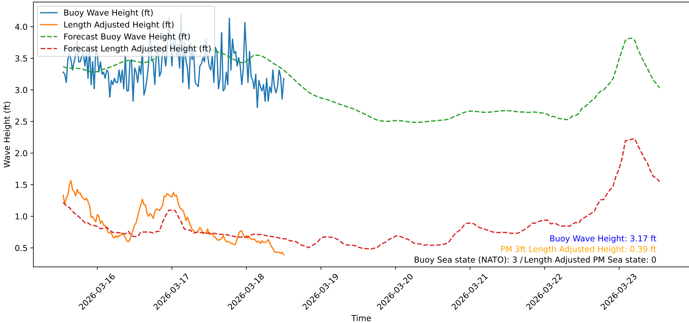
Wave Heights over Time for Green Beach at 2026-03-18 12:51:10
