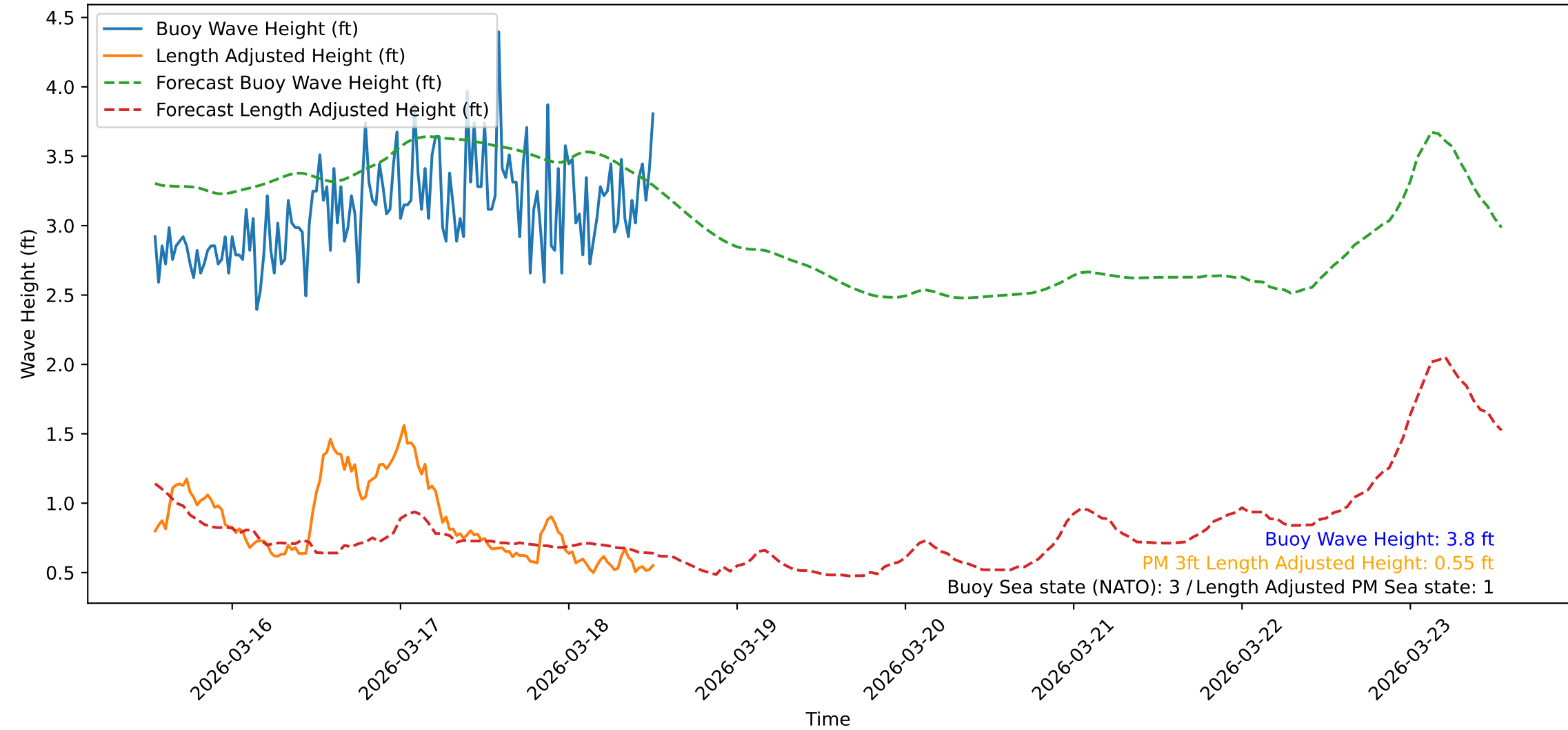
Wave Heights over Time for Oceanside Harbor at 2026-03-18 12:50:31
