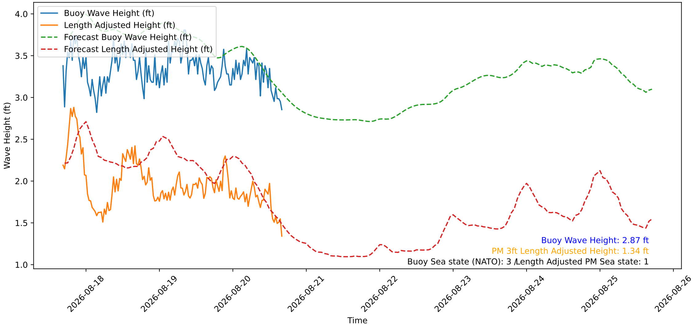
Wave Heights over Time for Oceanside Harbor at 2026-08-20 16:40:26
