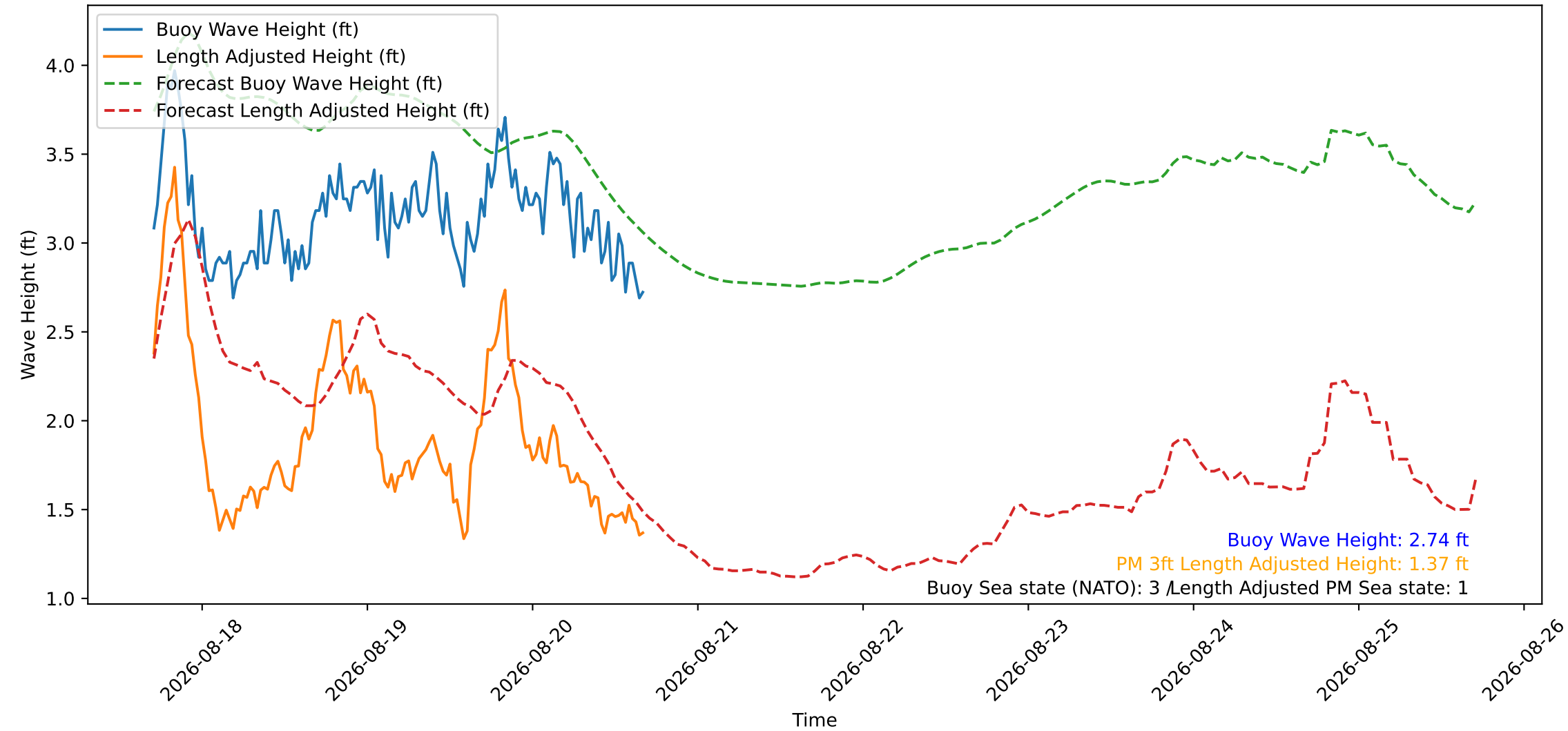
Wave Heights over Time for Green Beach at 2026-08-20 16:41:08
