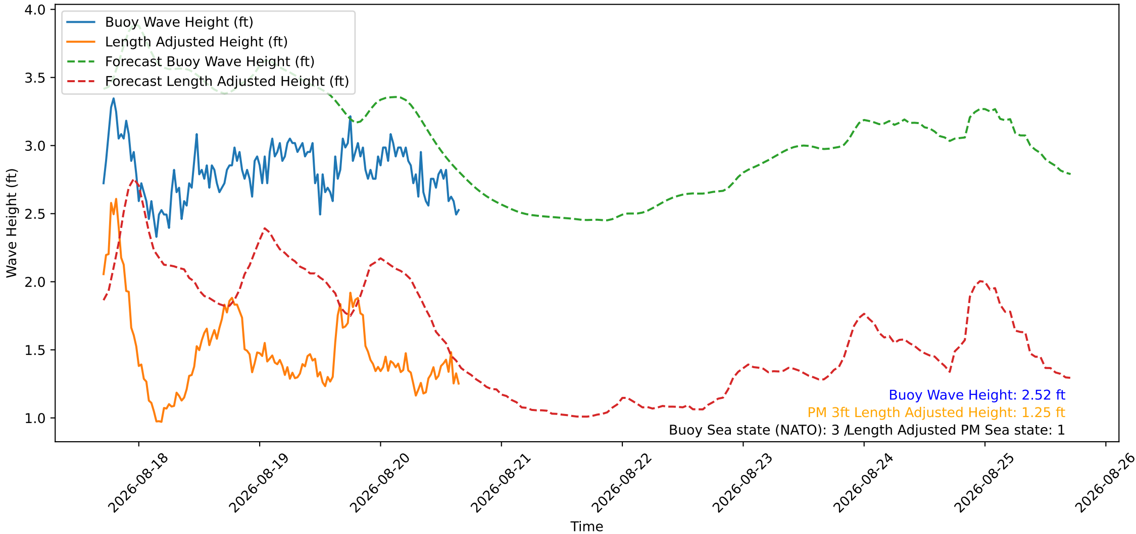
Wave Heights over Time for Red Beach at 2026-08-20 16:40:46
