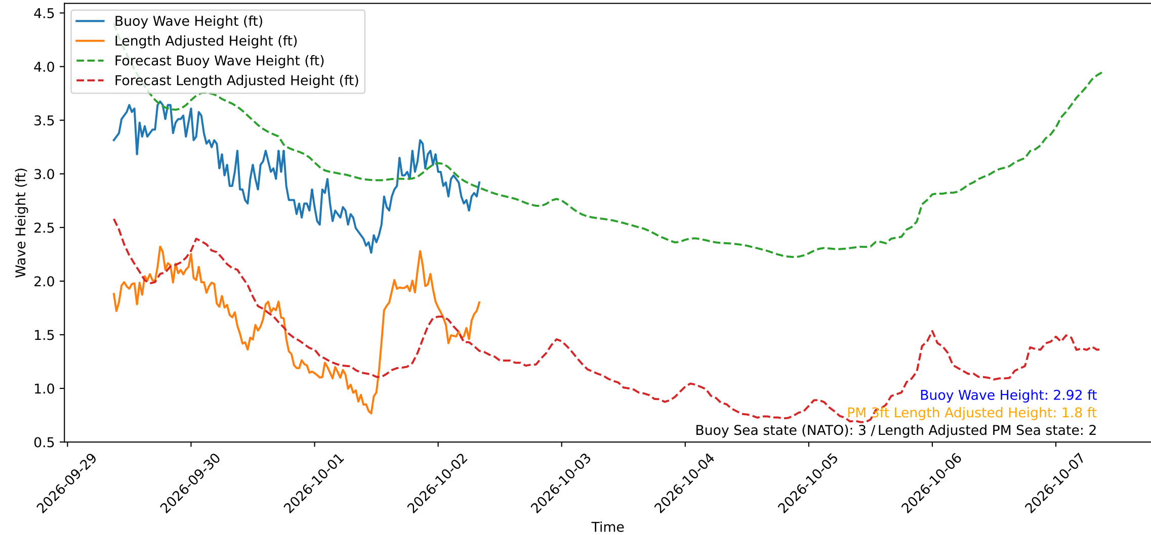
Wave Heights over Time for Oceanside Harbor at 2026-10-02 08:50:29
