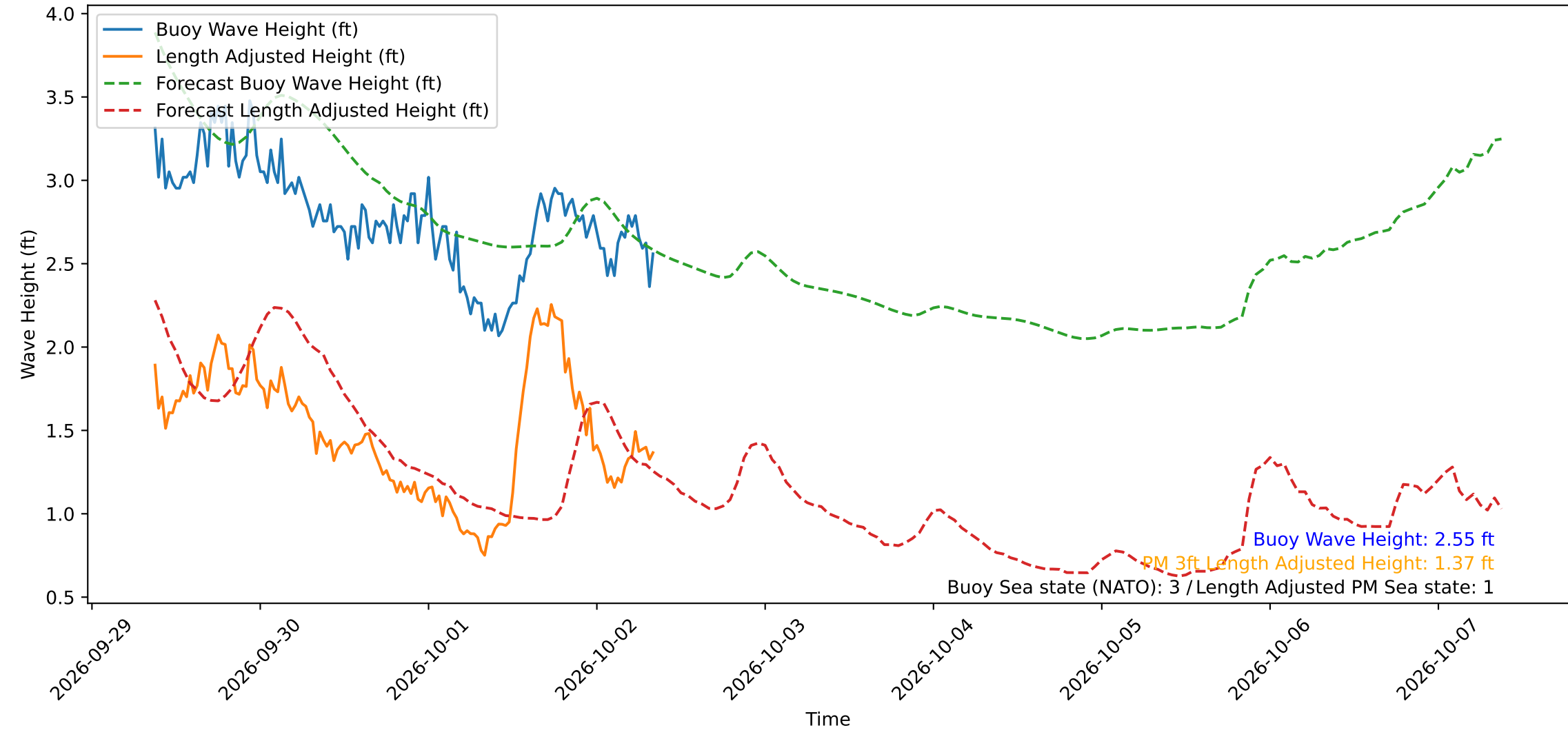
Wave Heights over Time for Red Beach at 2026-10-02 08:50:50
