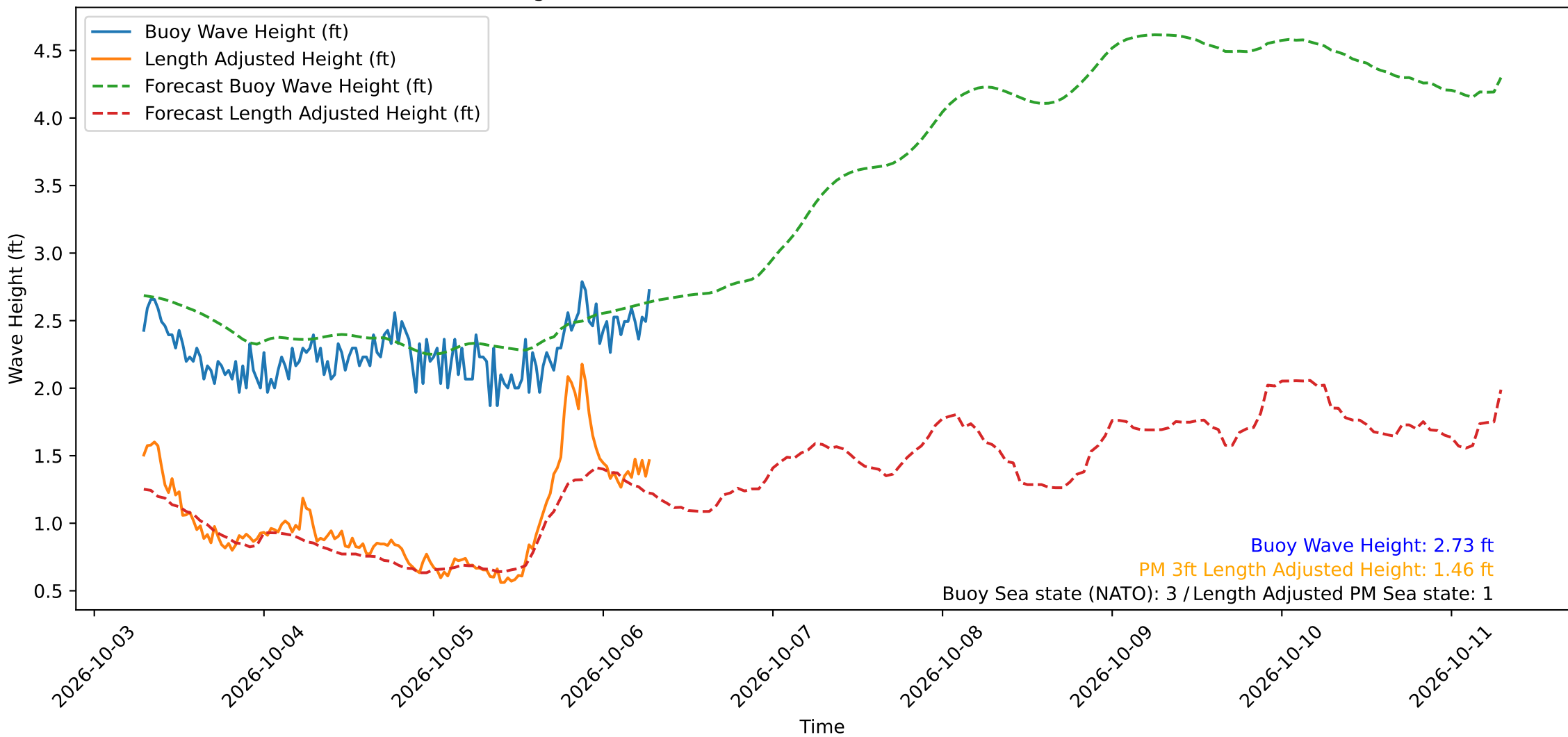
Wave Heights over Time for Oceanside Harbor at 2026-10-06 07:10:30
