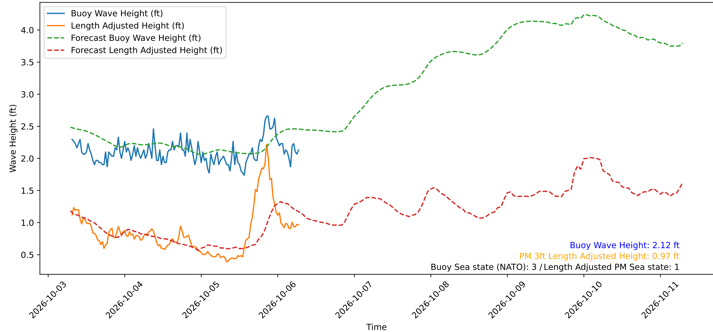
Wave Heights over Time for Red Beach at 2026-10-06 07:10:49
