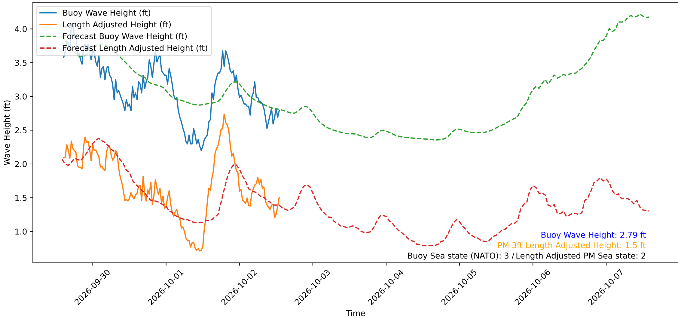
Wave Heights over Time for Green Beach at 2026-10-02 14:01:11
