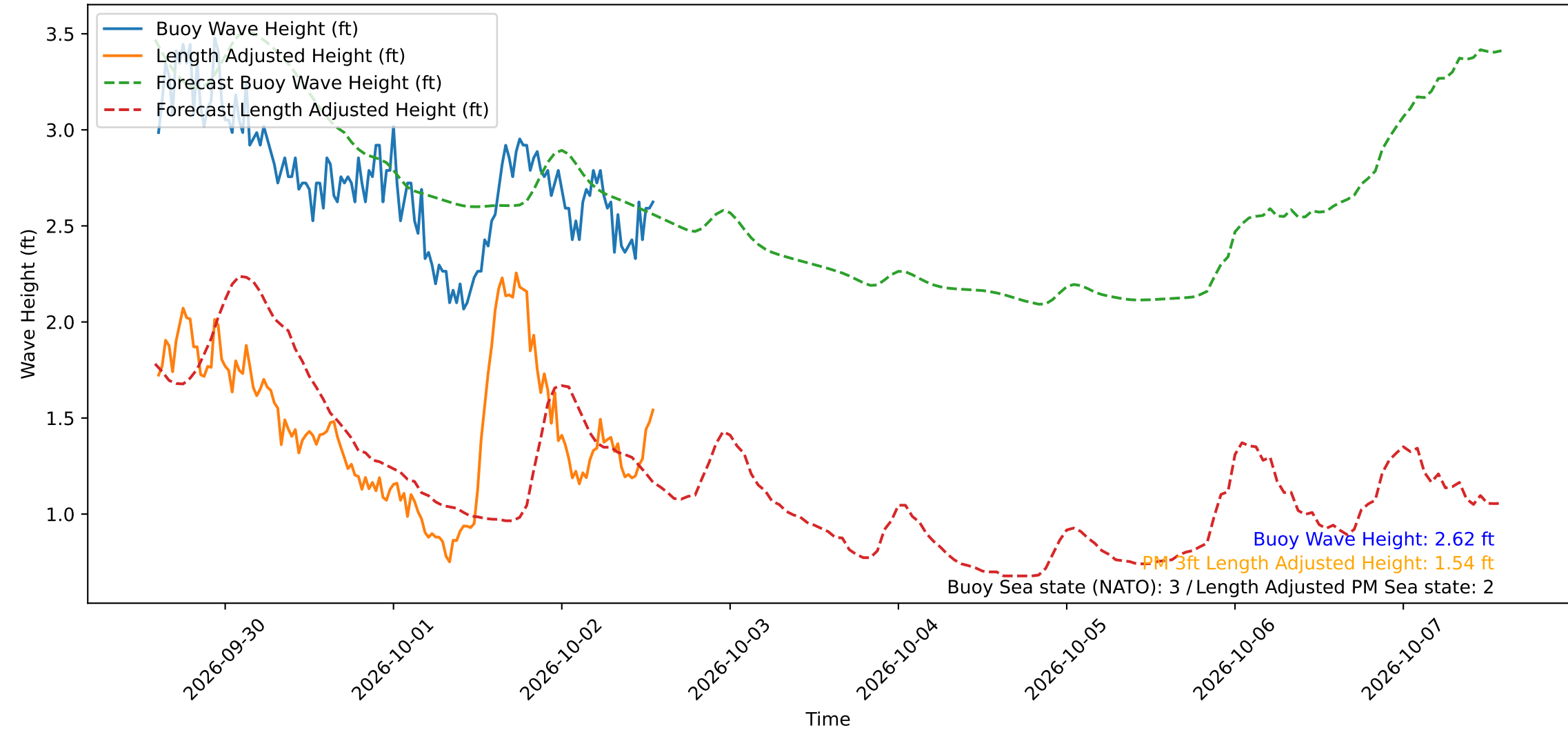
Wave Heights over Time for Red Beach at 2026-10-02 14:00:49
