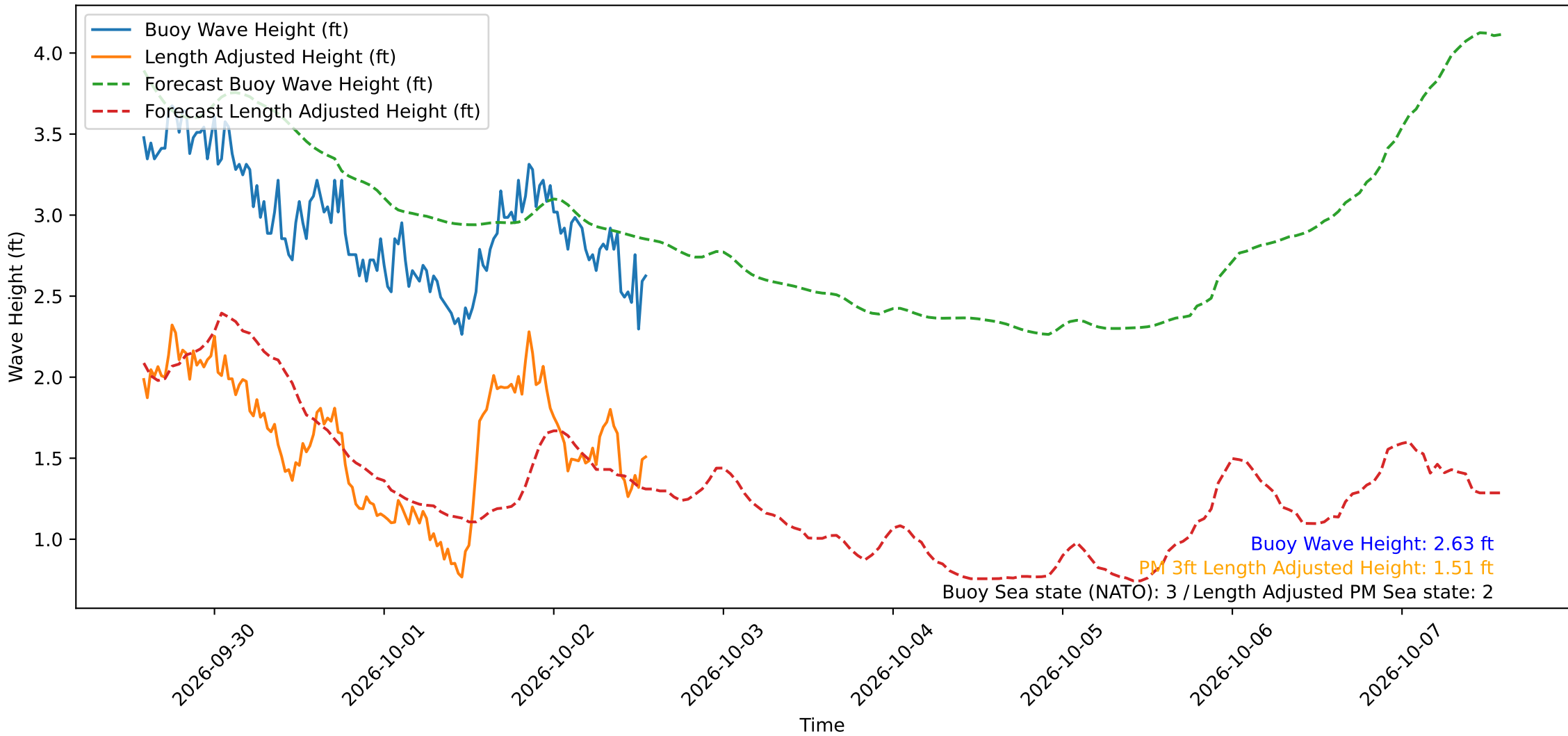
Wave Heights over Time for Oceanside Harbor at 2026-10-02 14:00:30
