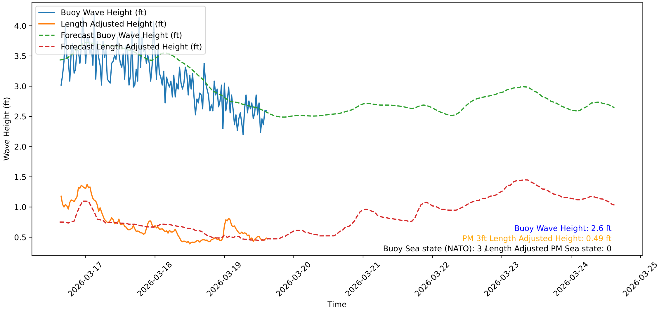
Wave Heights over Time for Green Beach at 2026-03-19 15:21:11
