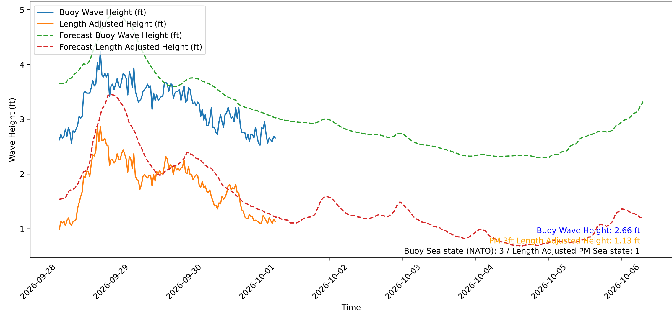
Wave Heights over Time for Oceanside Harbor at 2026-10-01 06:50:29
