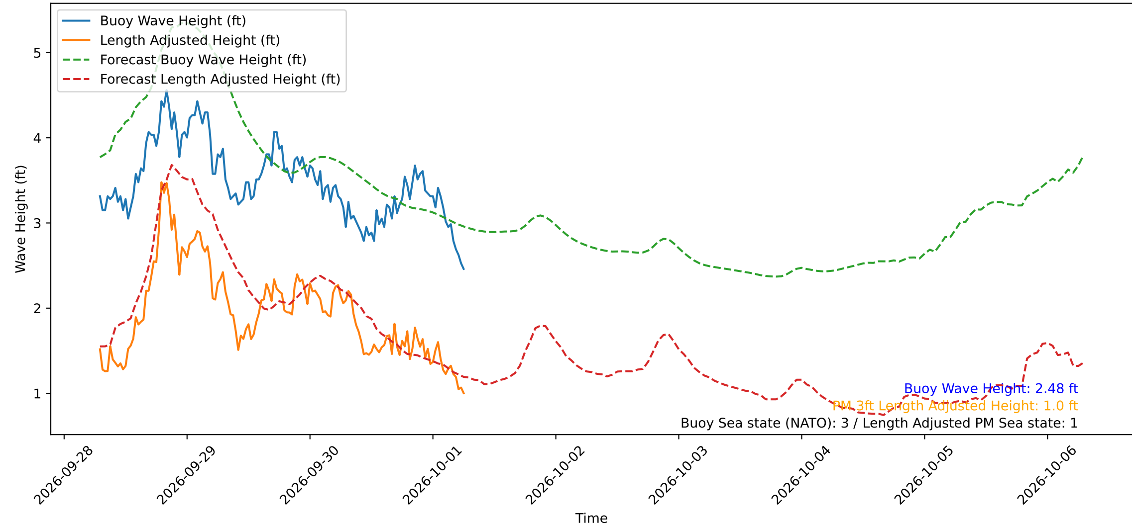
Wave Heights over Time for Green Beach at 2026-10-01 06:51:15
