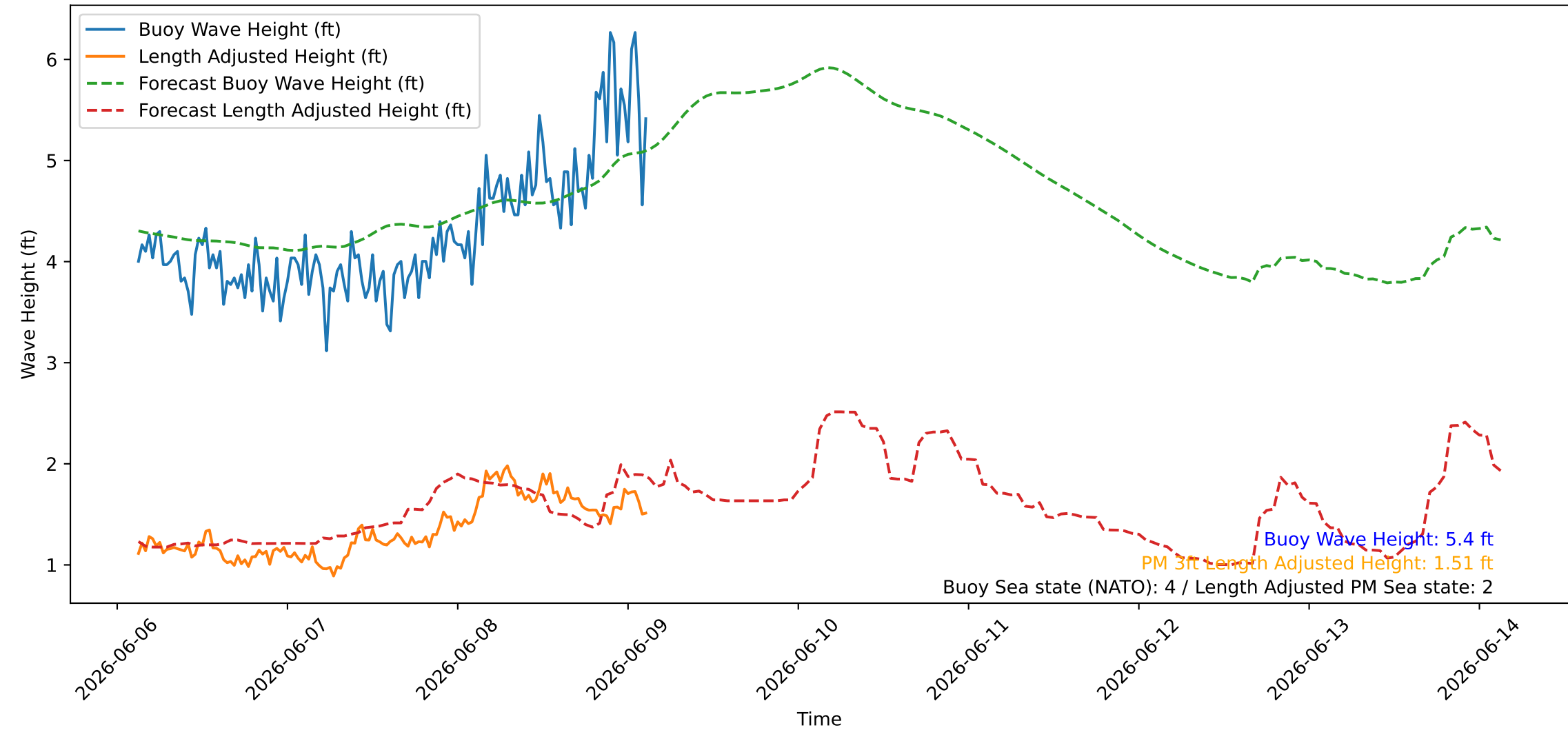
Wave Heights over Time for Green Beach at 2026-06-09 03:11:09
