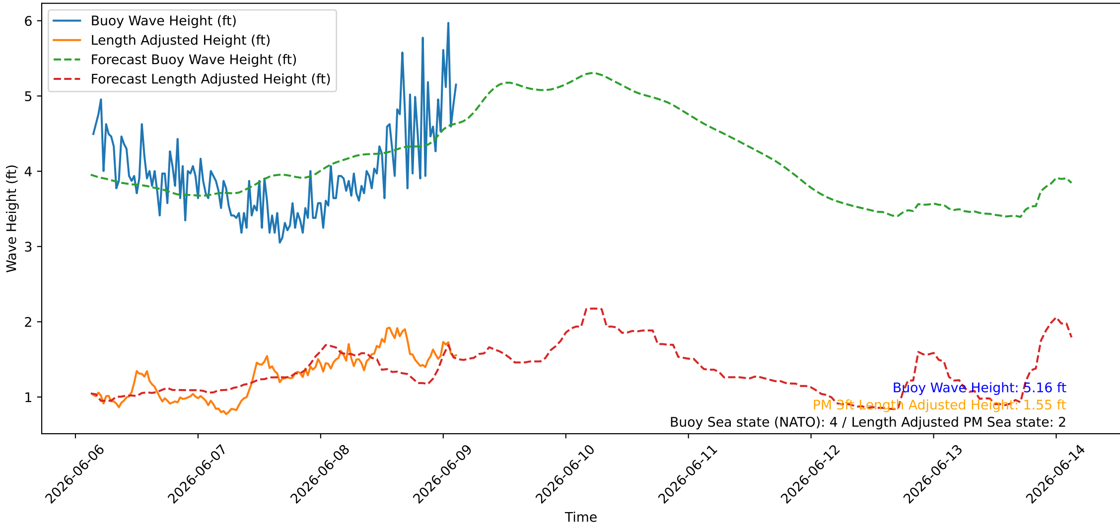
Wave Heights over Time for Red Beach at 2026-06-09 03:10:46
