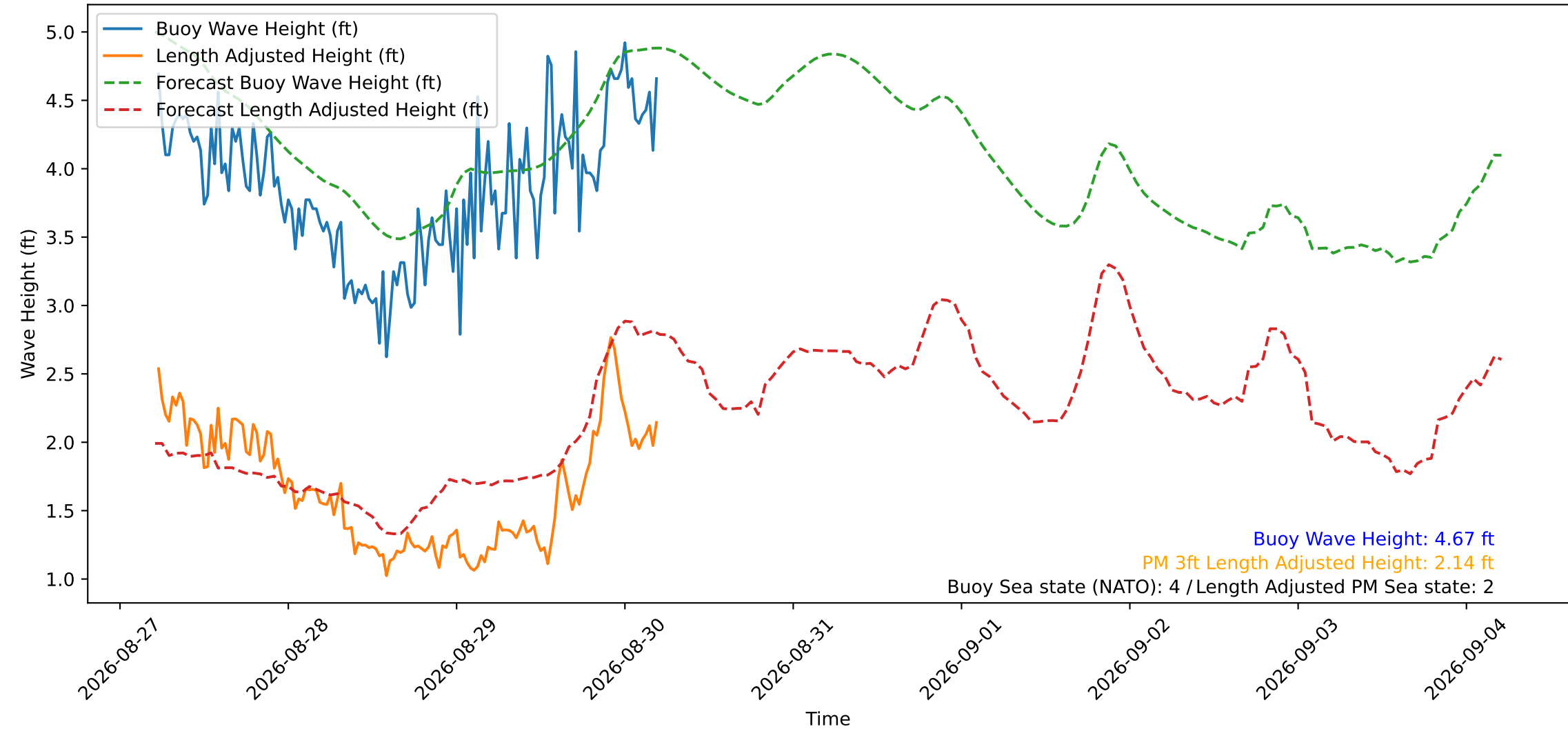
Wave Heights over Time for Green Beach at 2026-08-30 05:11:11
