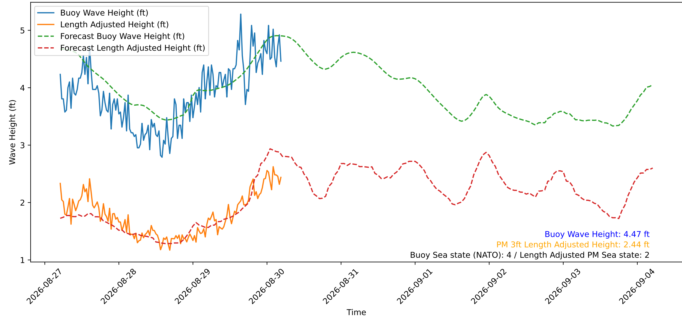
Wave Heights over Time for Oceanside Harbor at 2026-08-30 05:10:29
