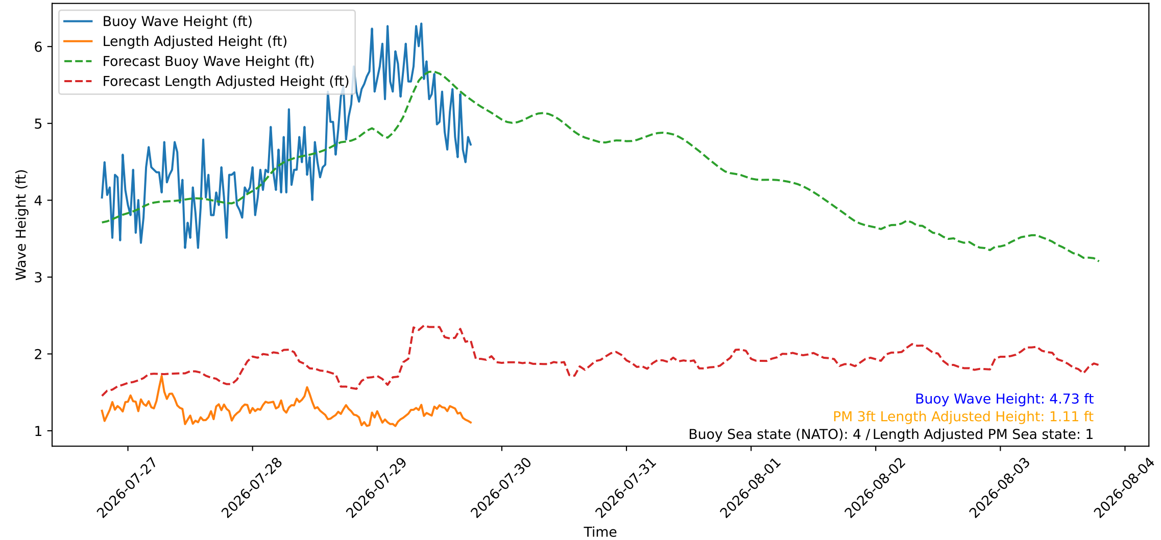
Wave Heights over Time for Green Beach at 2026-07-29 19:01:08
