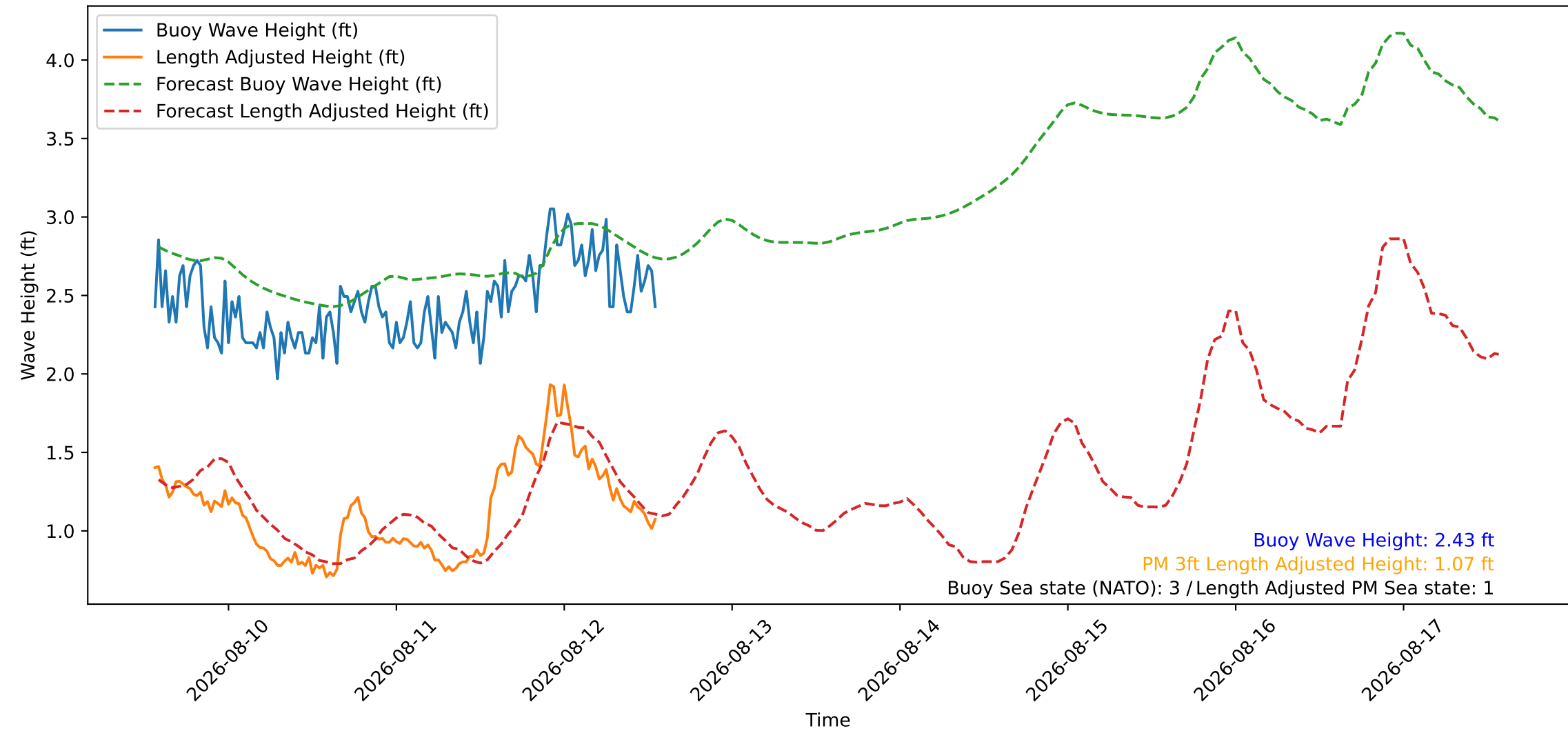
Wave Heights over Time for Oceanside Harbor at 2026-08-12 13:40:27
