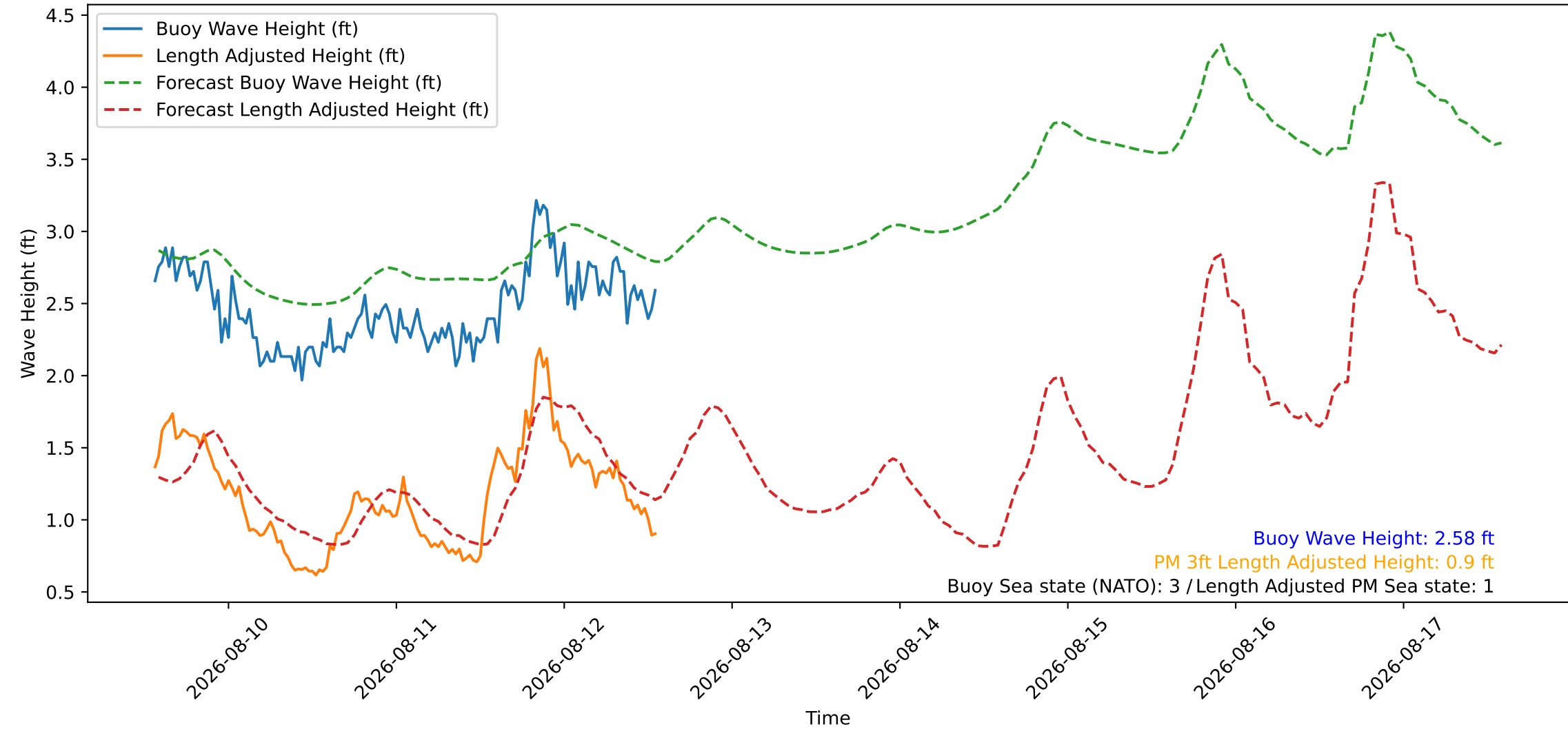
Wave Heights over Time for Green Beach at 2026-08-12 13:41:09
