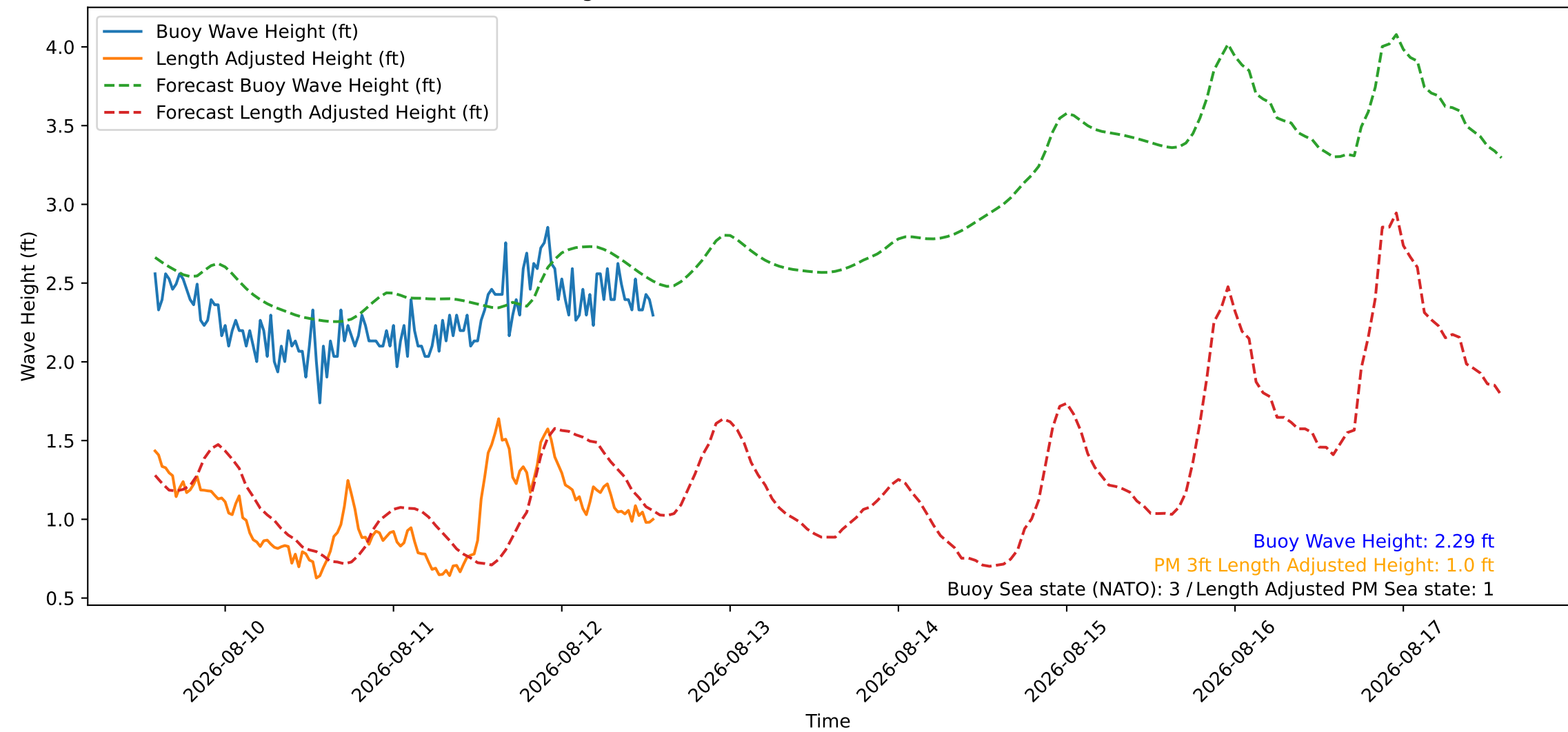
Wave Heights over Time for Red Beach at 2026-08-12 13:40:46
