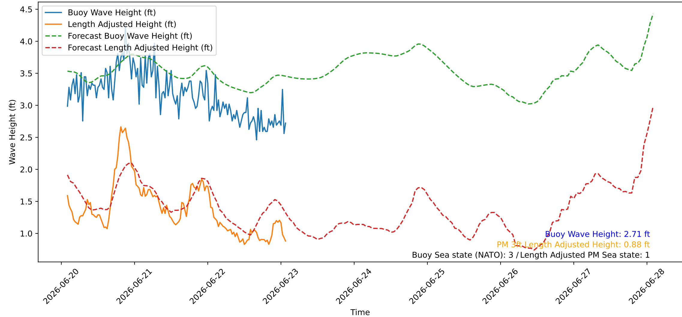
Wave Heights over Time for Green Beach at 2026-06-23 02:11:08
