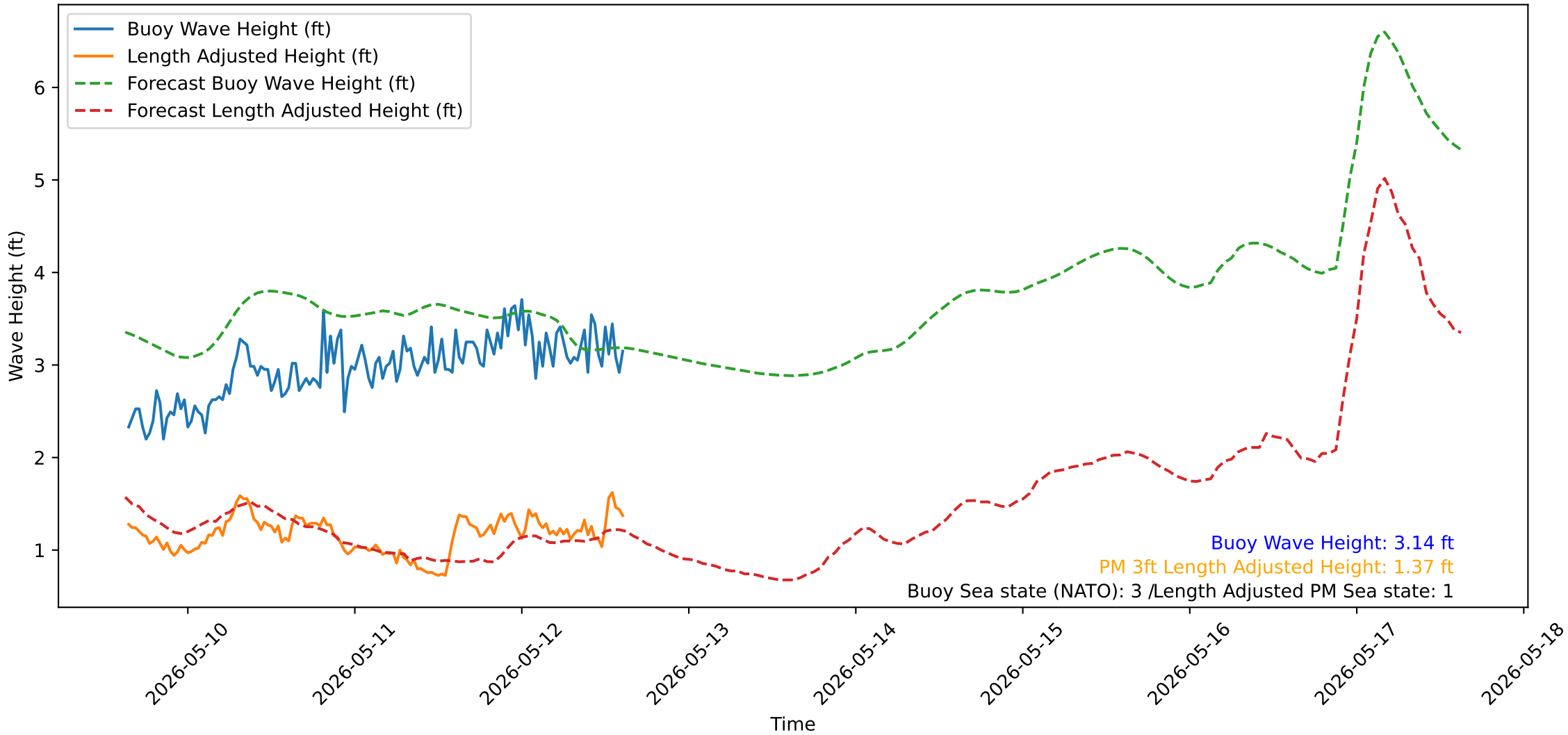
Wave Heights over Time for Oceanside Harbor at 2026-05-12 15:20:31
