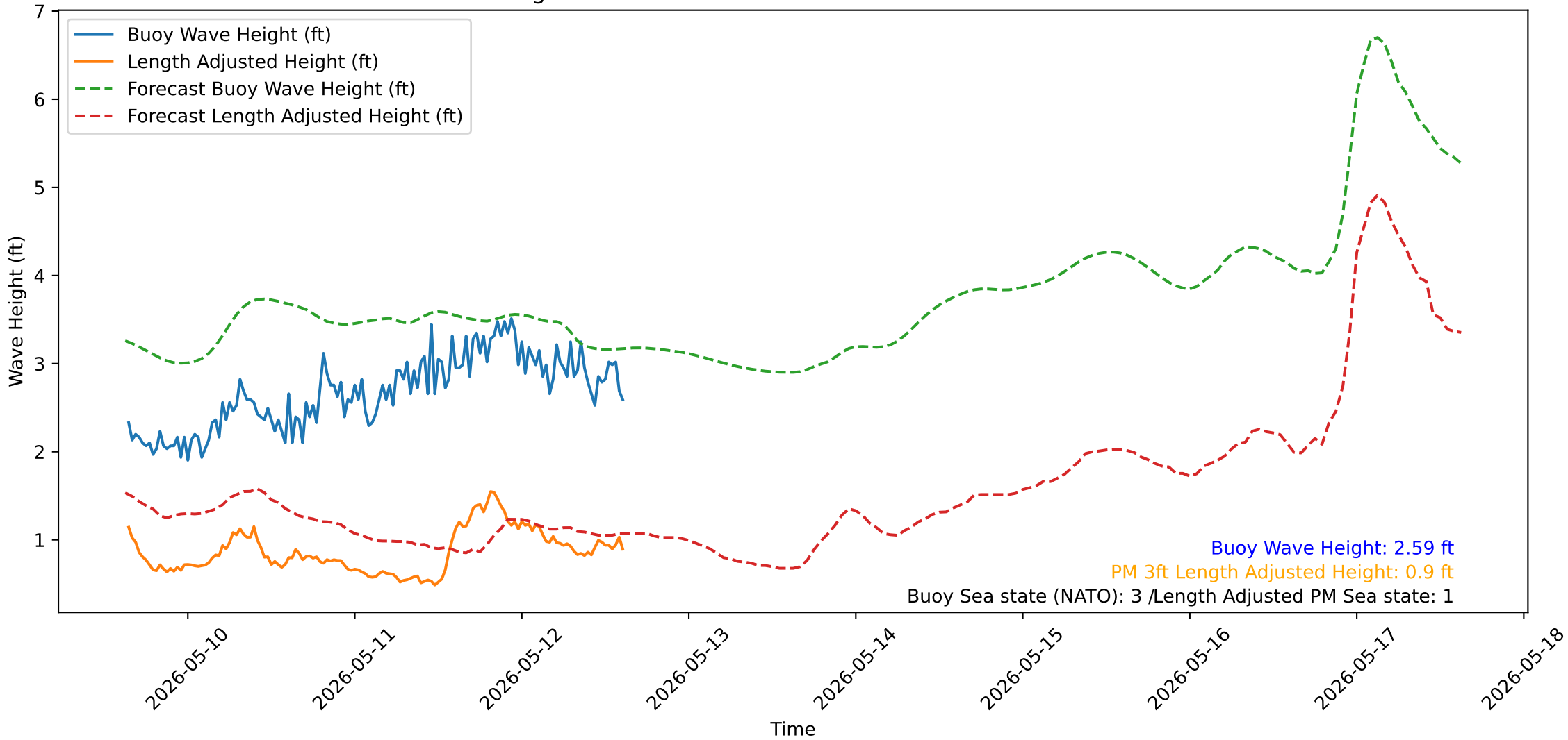
Wave Heights over Time for Green Beach at 2026-05-12 15:21:14
