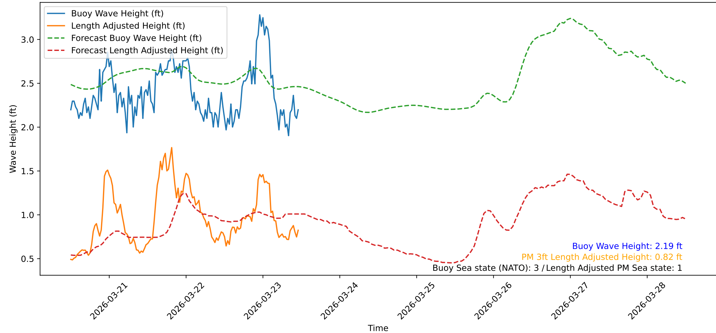
Wave Heights over Time for Green Beach at 2026-03-23 11:51:10
