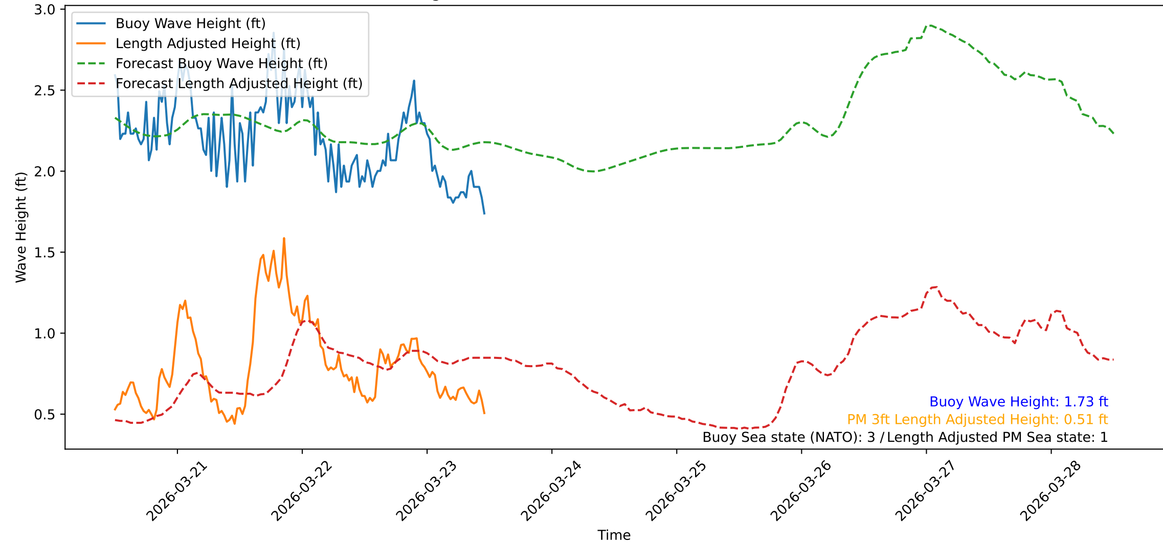
Wave Heights over Time for Red Beach at 2026-03-23 11:50:47
