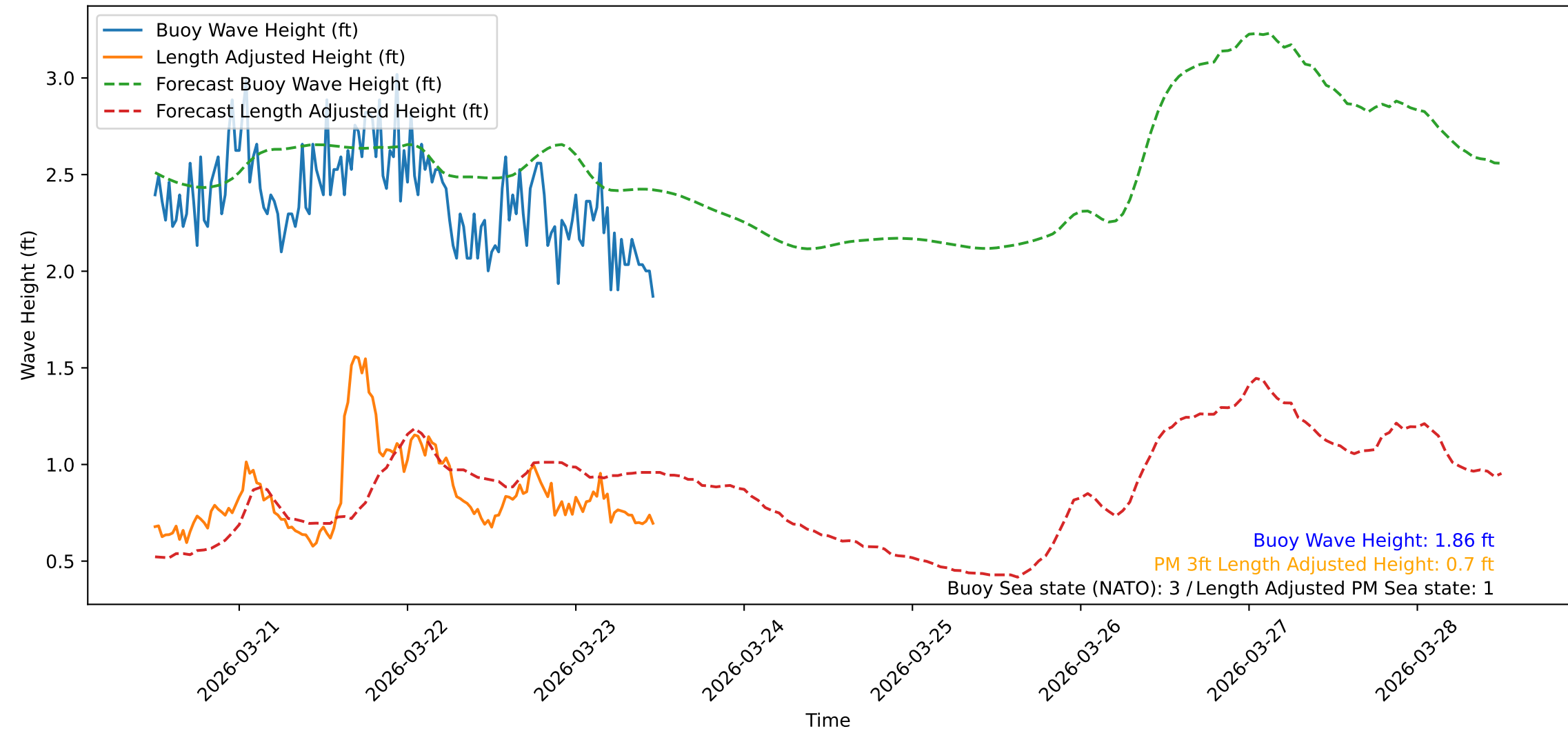
Wave Heights over Time for Oceanside Harbor at 2026-03-23 11:50:31
