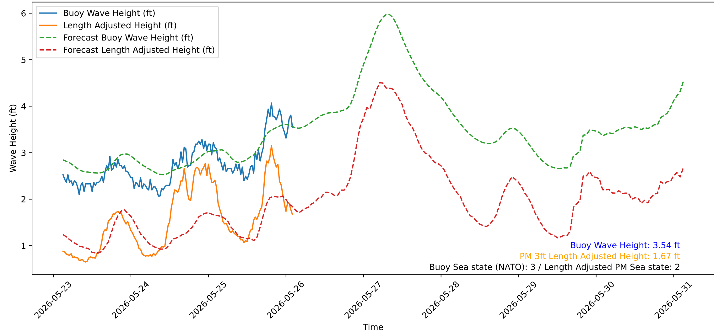
Wave Heights over Time for Green Beach at 2026-05-26 03:01:10
