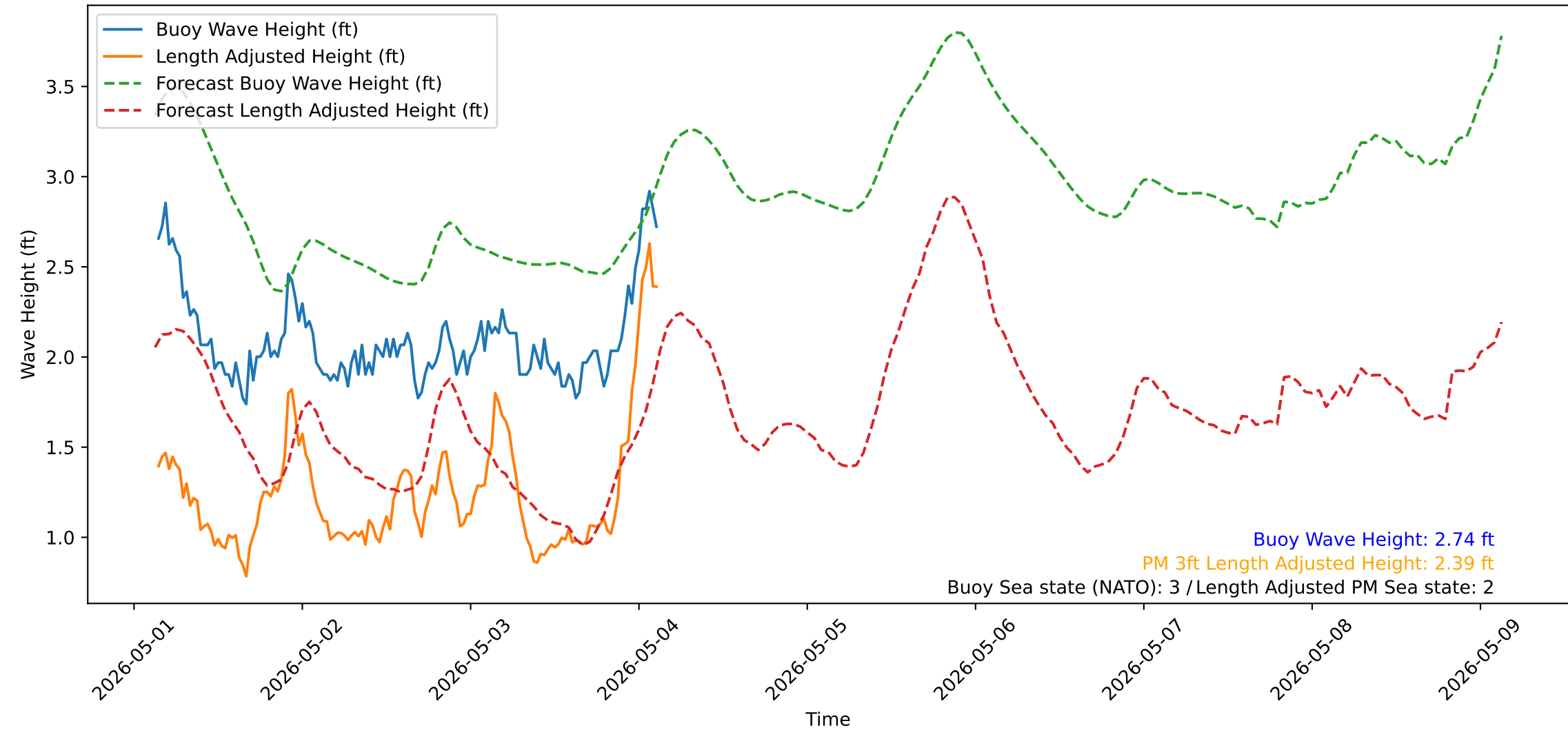
Wave Heights over Time for Green Beach at 2026-05-04 03:21:13
