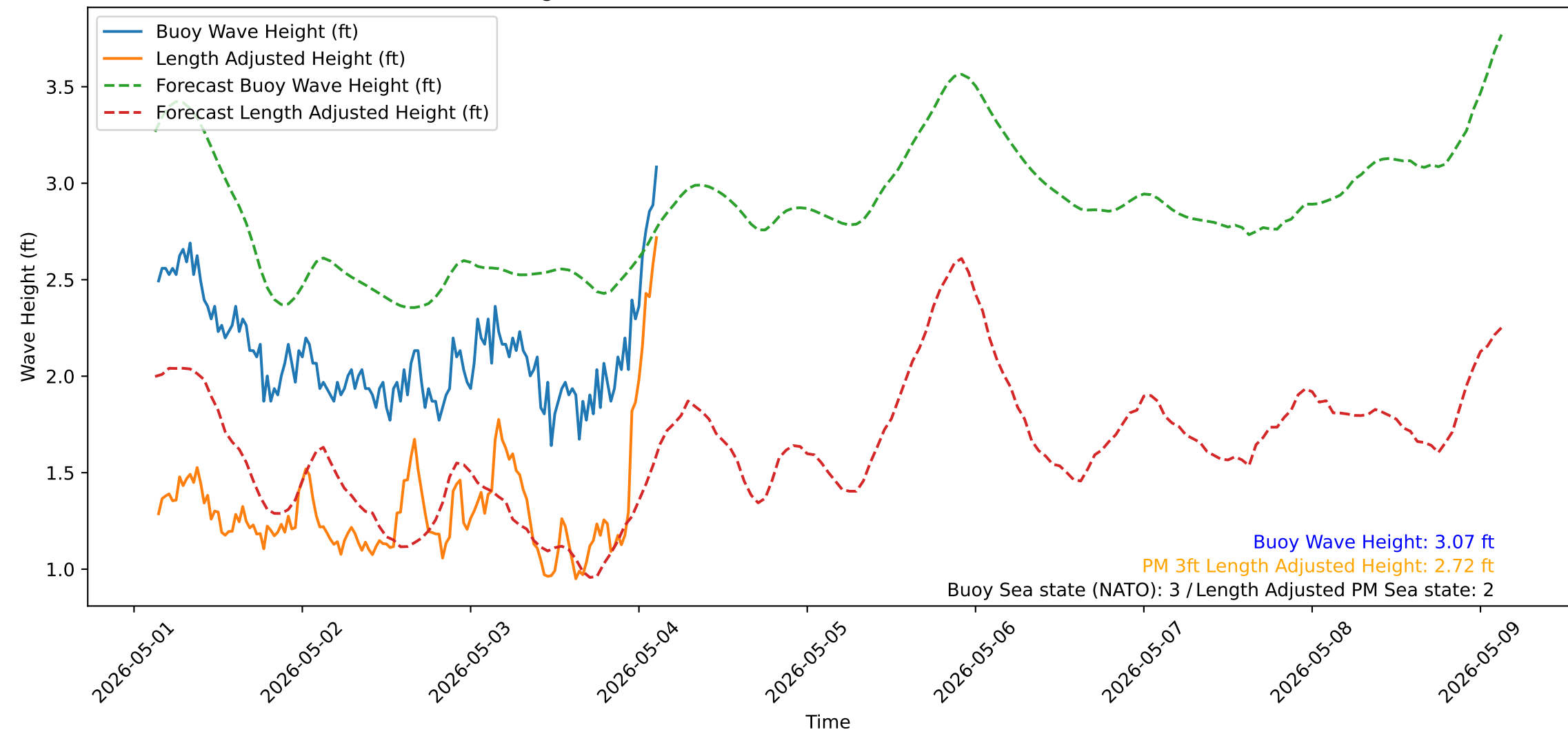
Wave Heights over Time for Oceanside Harbor at 2026-05-04 03:20:31
