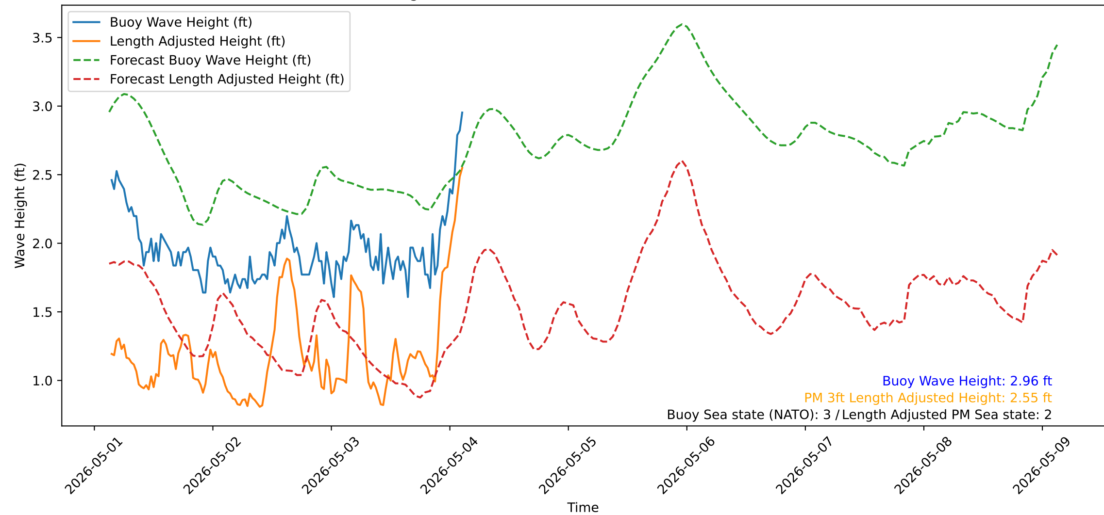
Wave Heights over Time for Red Beach at 2026-05-04 03:20:51
